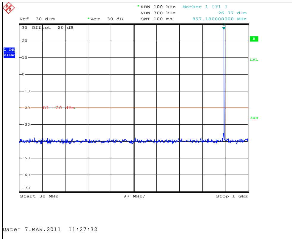
Figure 7.3.2-5: 896.01875 MHz – 30MHz to 1GHz
