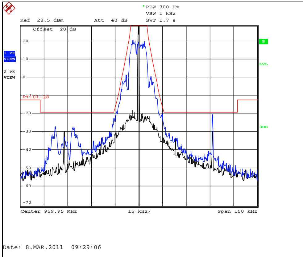
Figure 7.2.2-31: MPass Mode (10k) – 959.95 MHz
