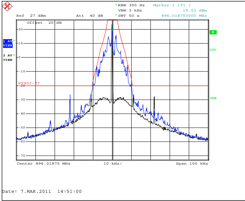
Figure 7.2.2-12: Normal Mode – 896.01875 MHz
