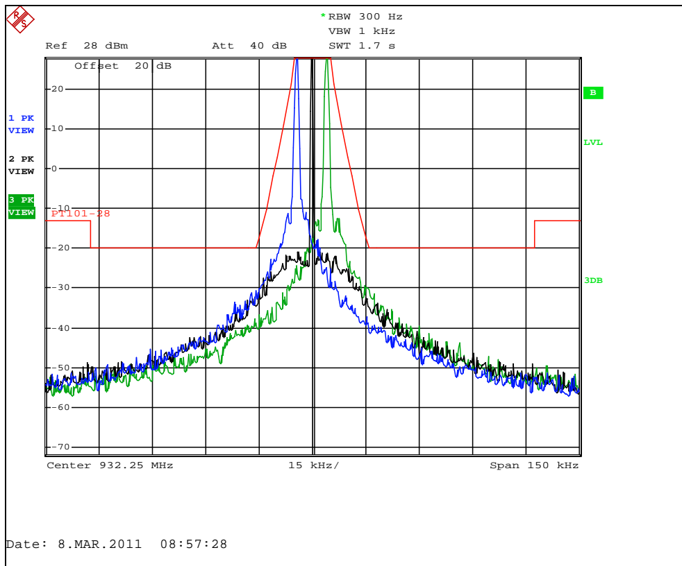
Figure 7.2.2-25: Boost Mode – 932.25 MHz Offset Channel of +/- 7 (+/- 4200 Hz)
