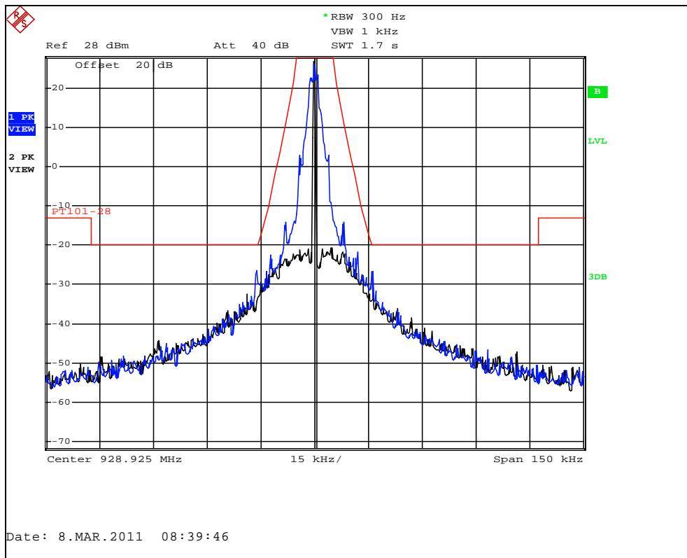
Figure 7.2.2-19: C&I Mode – 928.925 MHz
