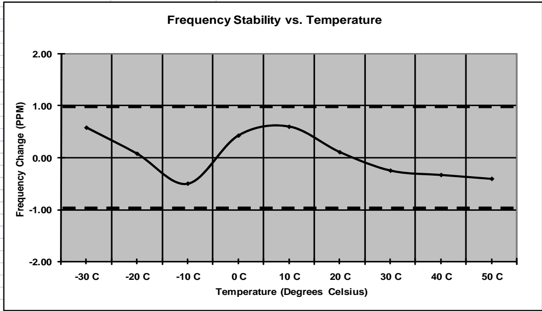
Figure 7.4.2-2: Frequency Stability – 896.01875 MHz
