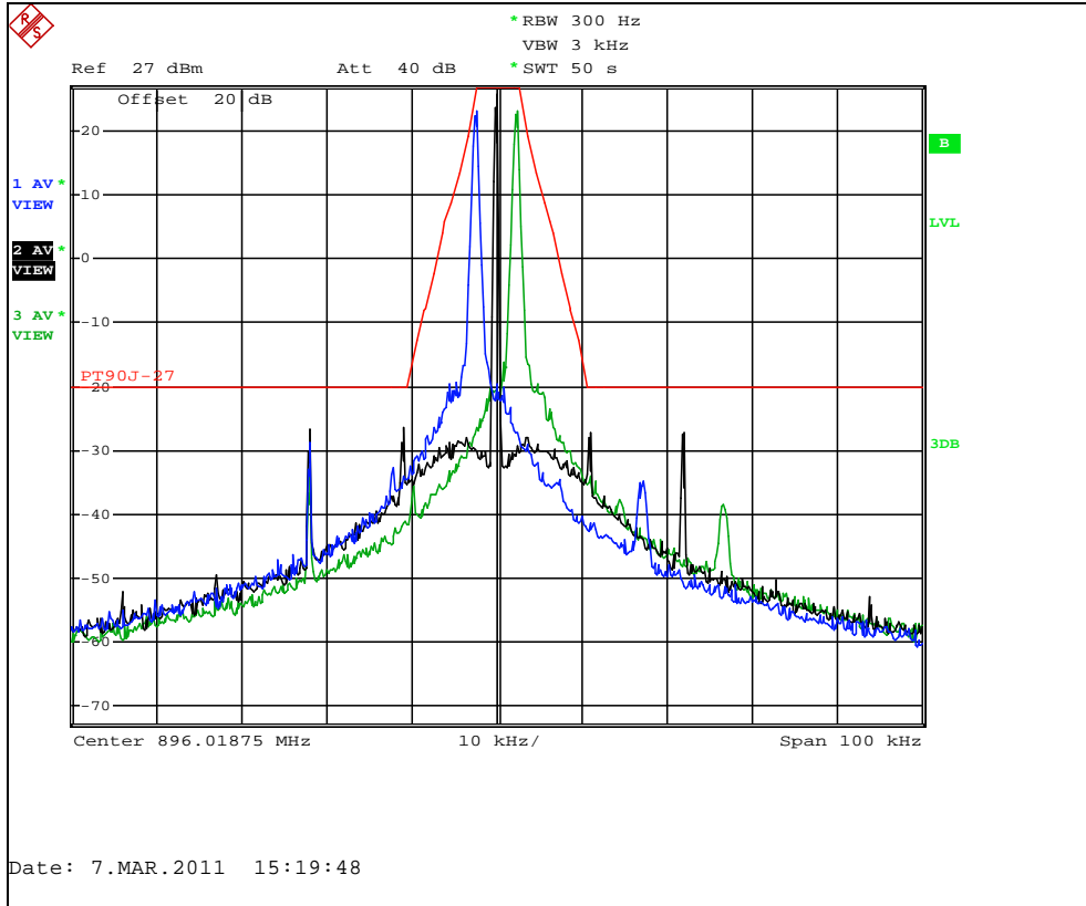
Figure 7.2.2-14: Boost Mode – 896.01875 MHz Offset Channel of +/- 4 (+/- 2400 Hz)
