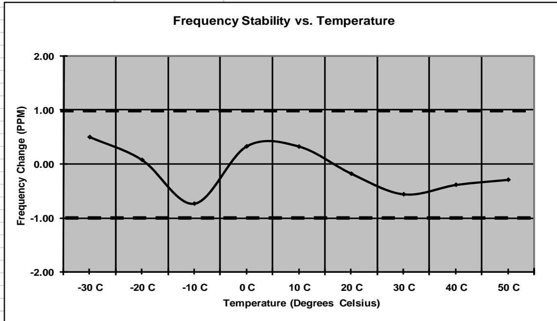
Figure 7.4.2-3: Frequency Stability – 959.925 MHz
