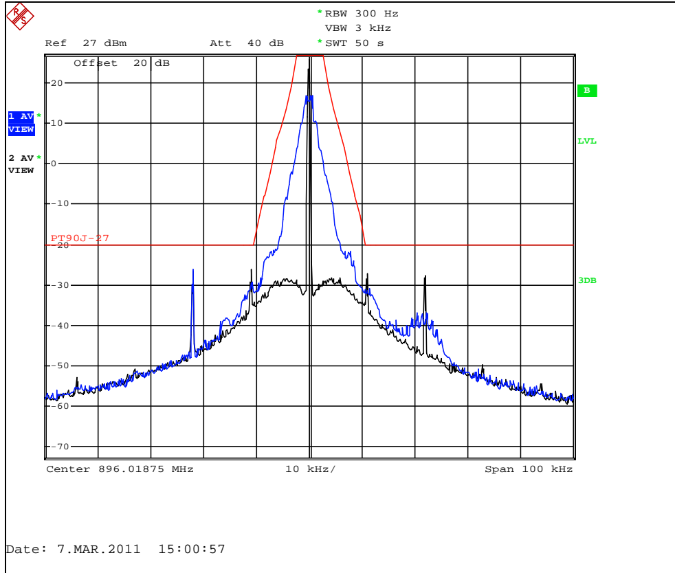
Figure 7.2.2-16: Priority Mode – 896.01875 MHz
