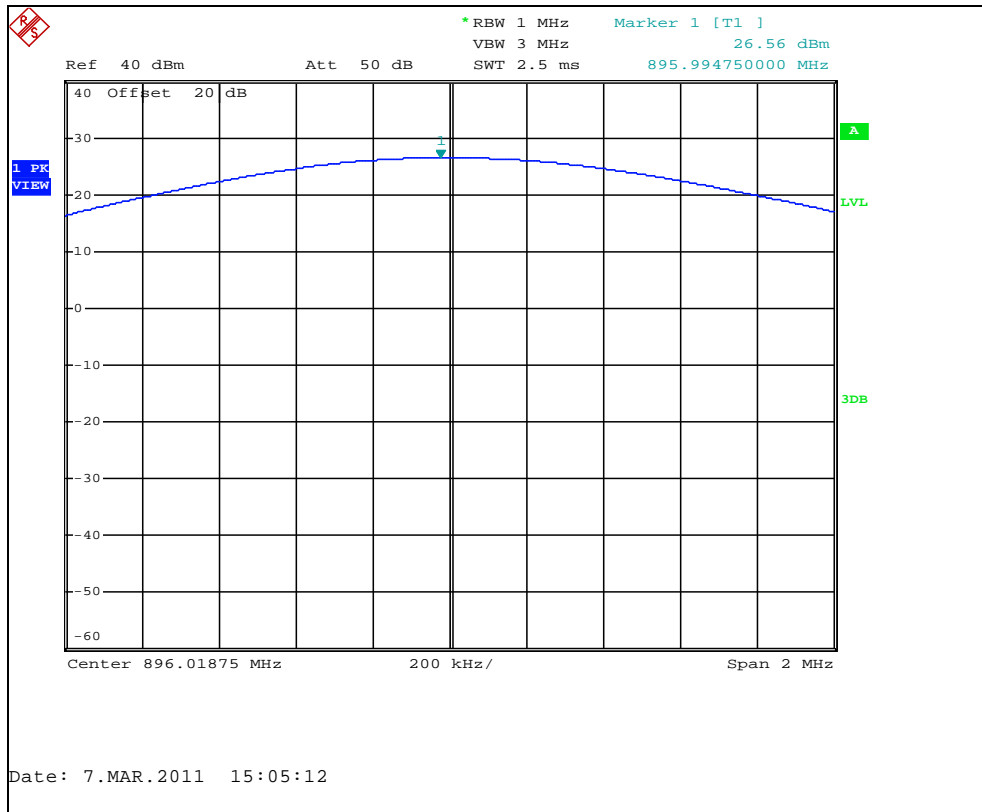
Figure 7.1.2-3: Peak Output Power 896.01875 MHz
