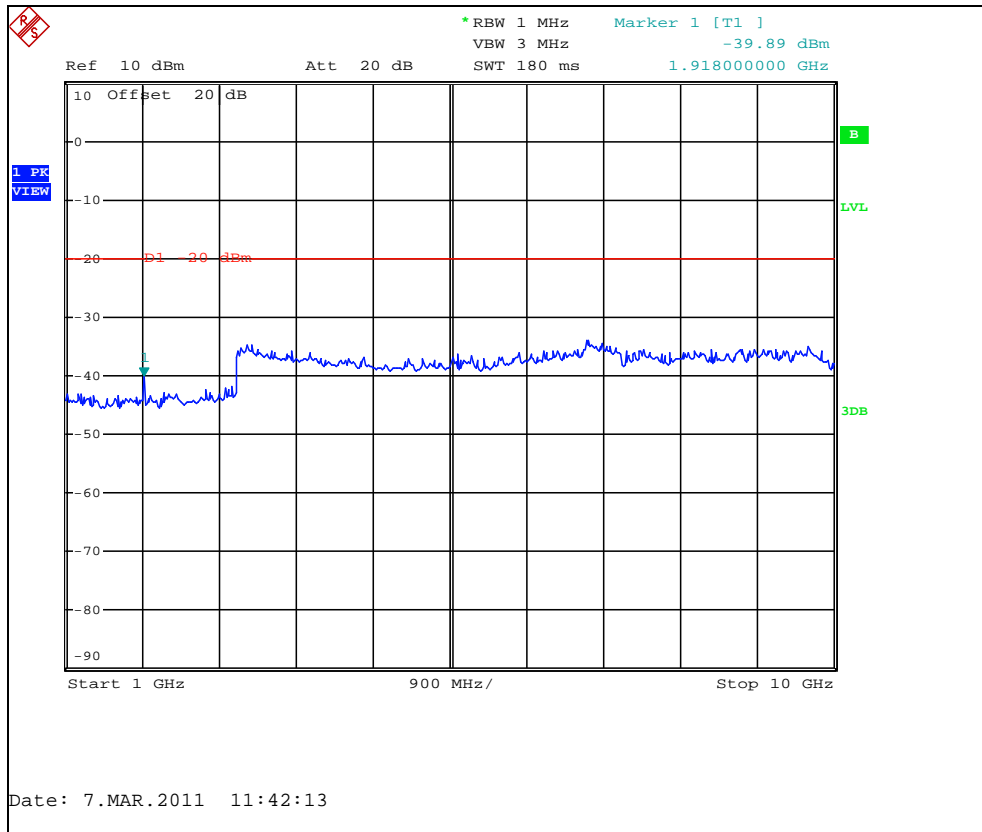
Figure 7.3.2-16: 959.95 MHz – 1GHz to 10GHz
