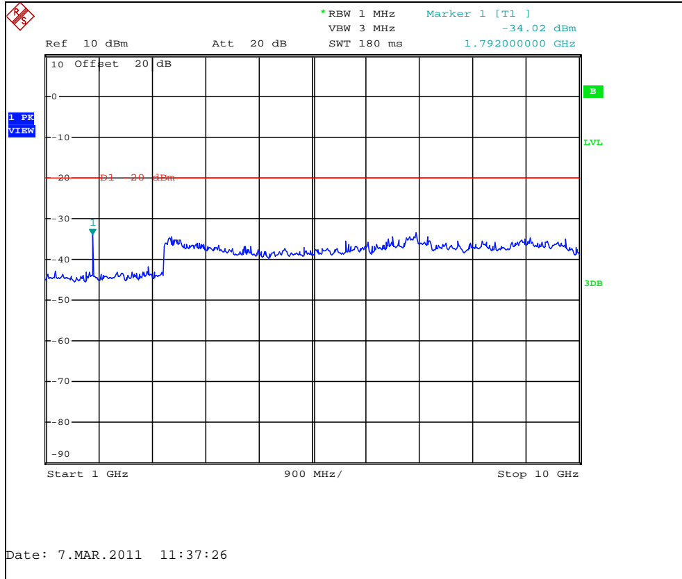
Figure 7.3.2-6: 896.01875 MHz – 1GHz to 10GHz
