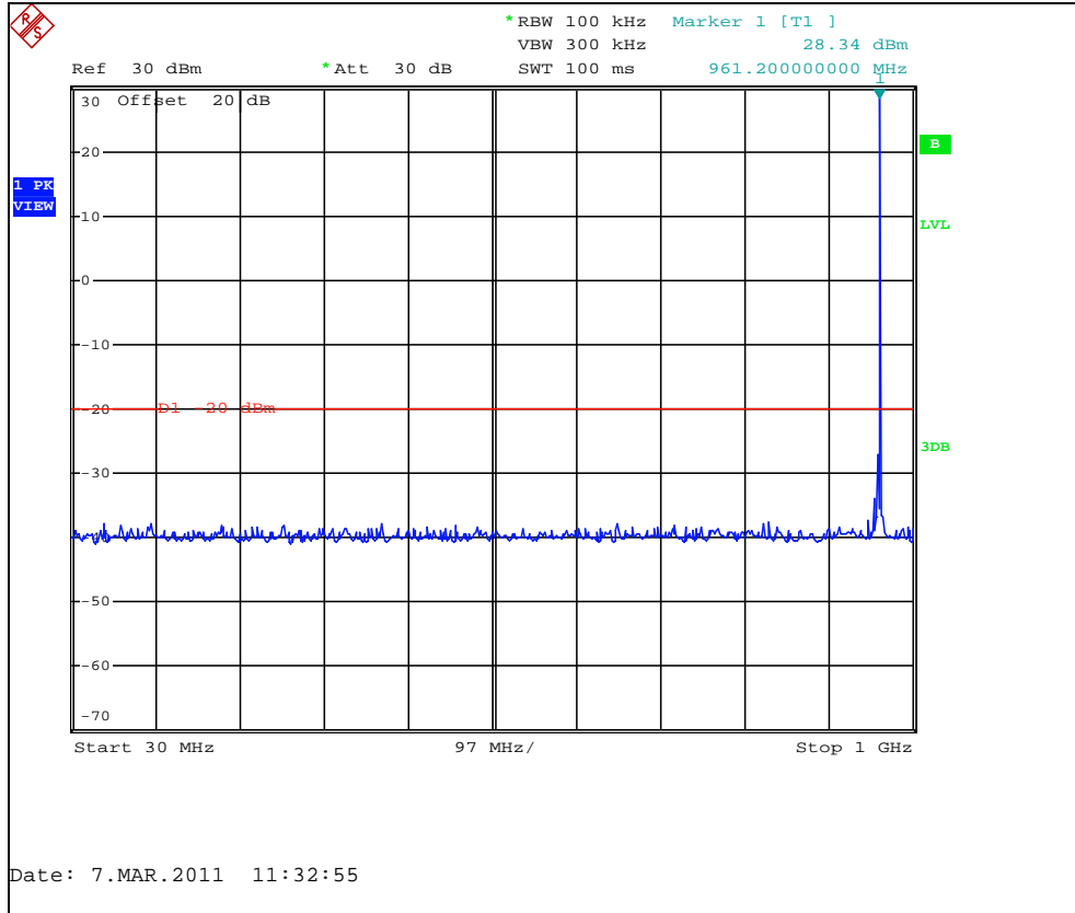
Figure 7.3.2-15: 959.95 MHz – 30MHz to 1GHz
