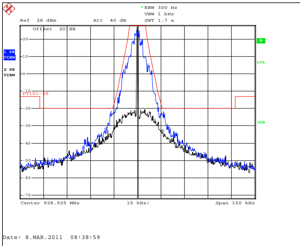
Figure 7.2.2-21: Double Density Mode – 928.925 MHz
