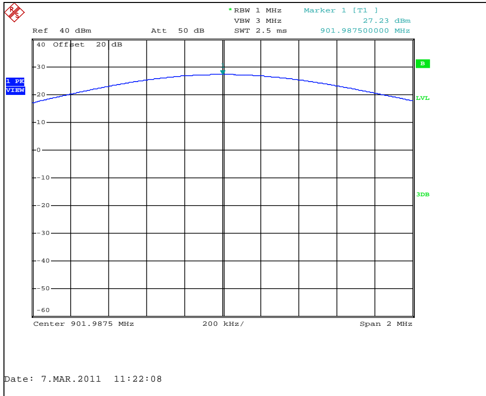
Figure 7.1.2-1: Peak Output Power 901.9875 MHz
