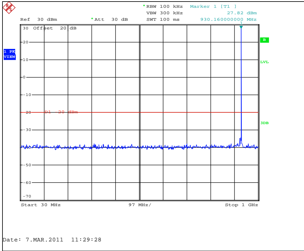
Figure 7.3.2-9: 928.925 MHz – 30MHz to 1GHz
