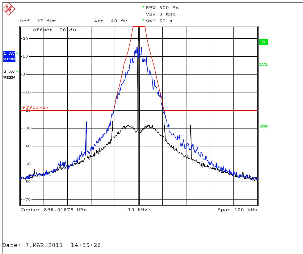
Figure 7.2.2-15: Double Density Mode – 896.01875 MHz
