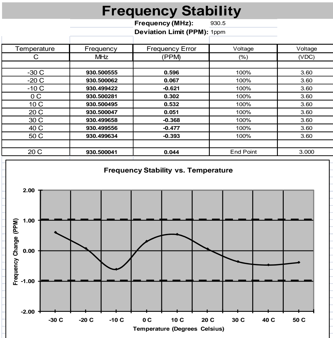
Figure 7.4.2-1: Frequency Stability – 930.5MHz
