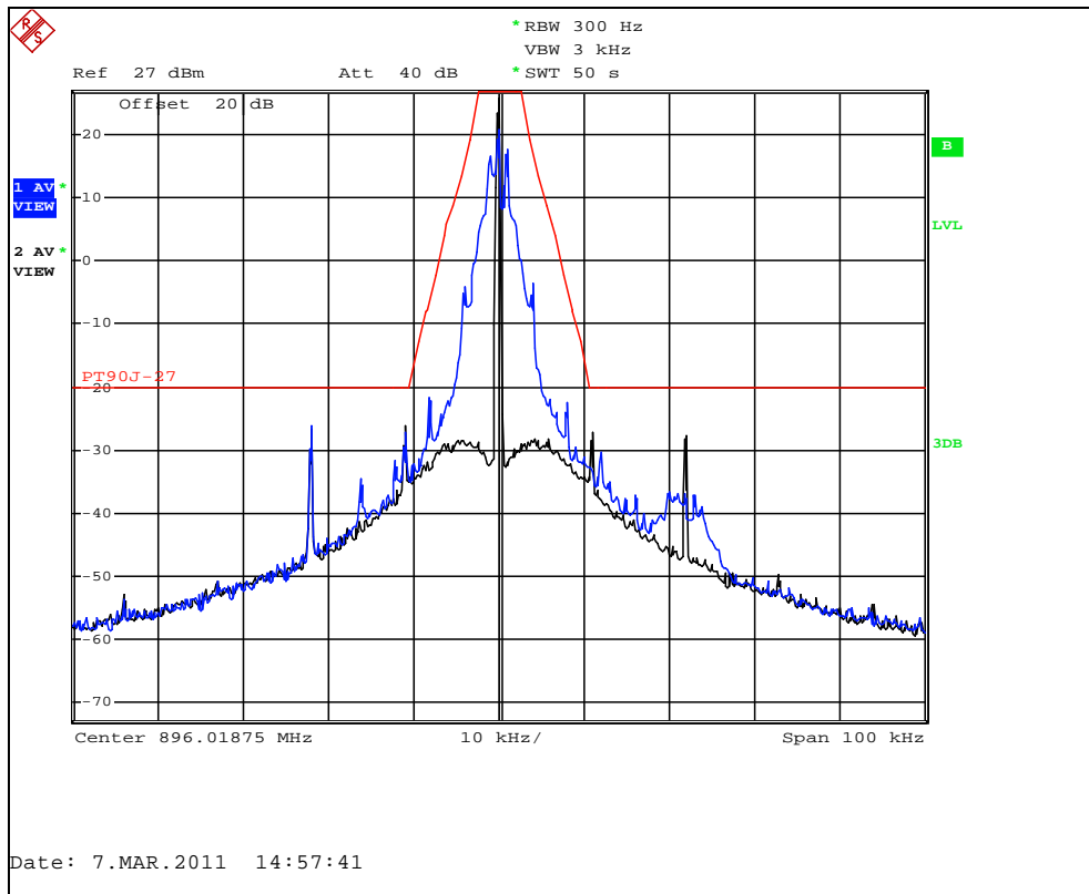
Figure 7.2.2-13: C&I Mode – 896.01875 MHz
