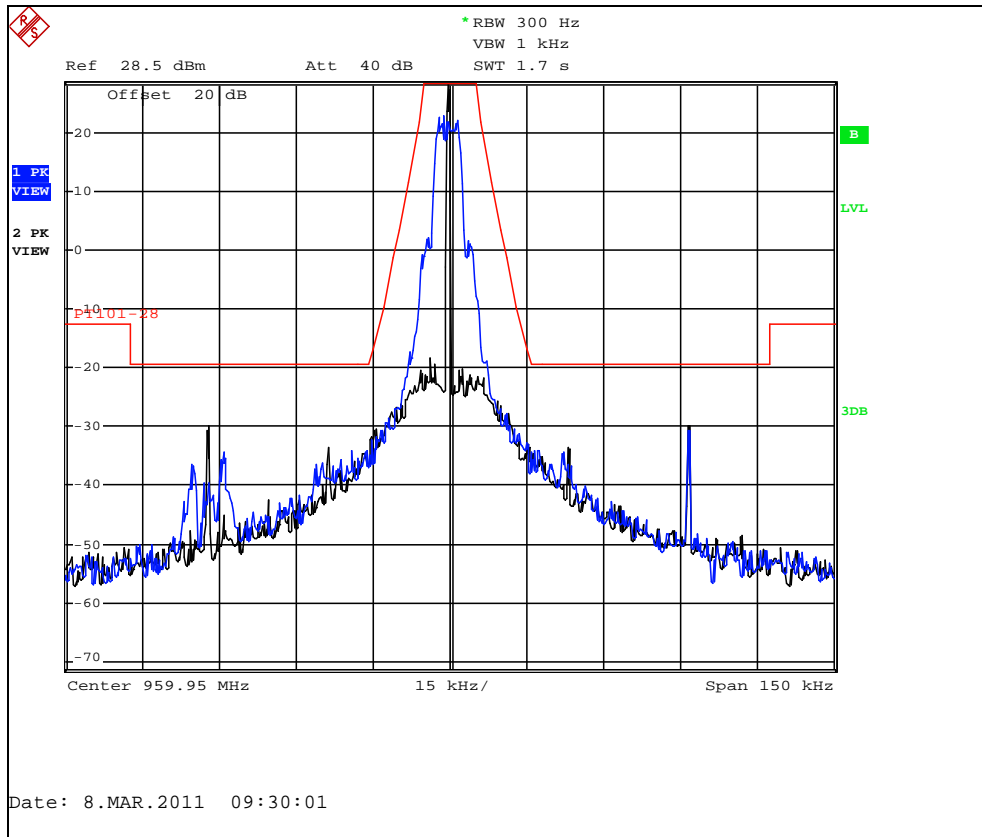
Figure 7.2.2-30: MPass Mode (5k) – 959.95 MHz
