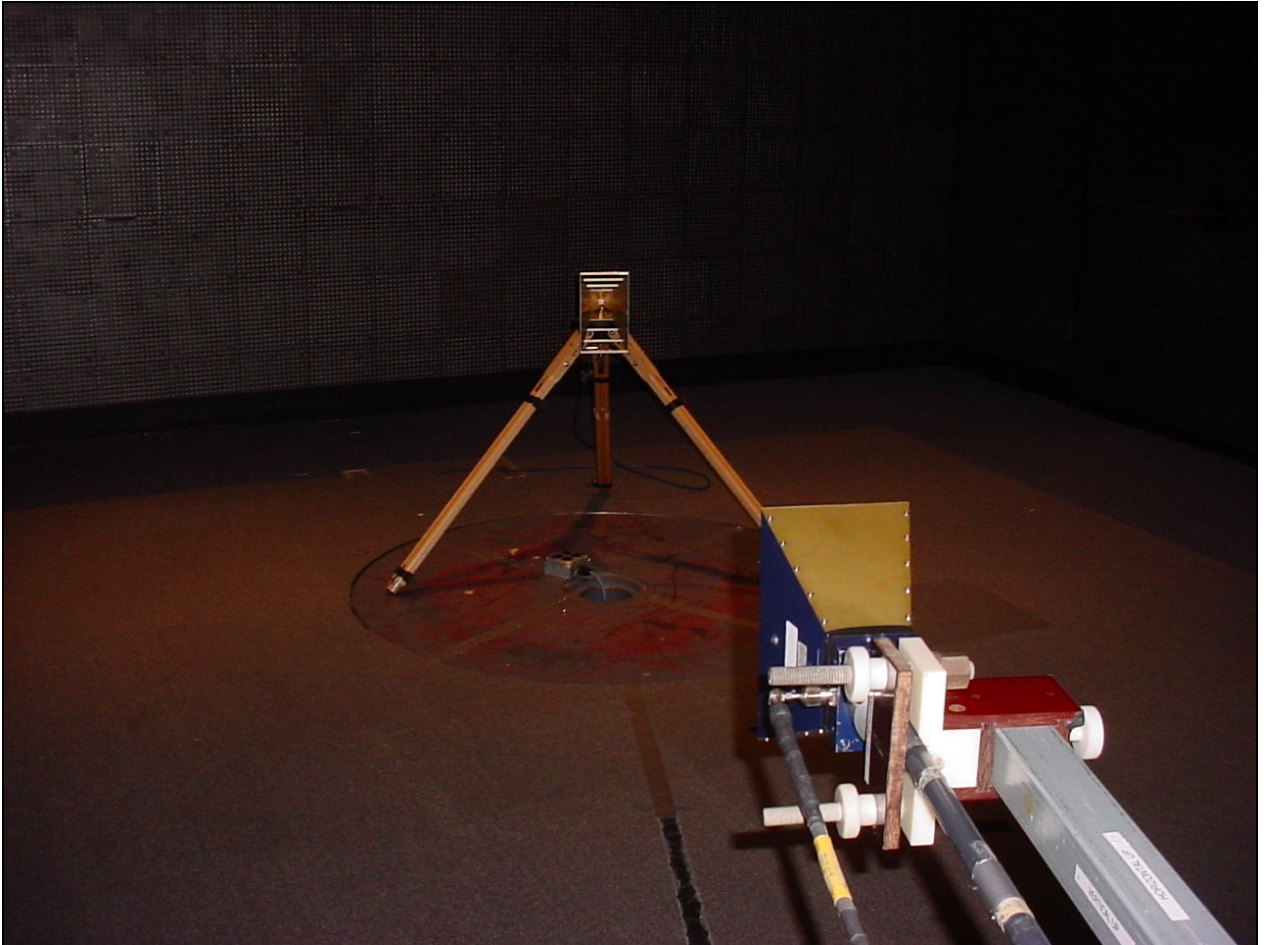
Figure 3: Radiated Emissions (Substitution Measurement)
