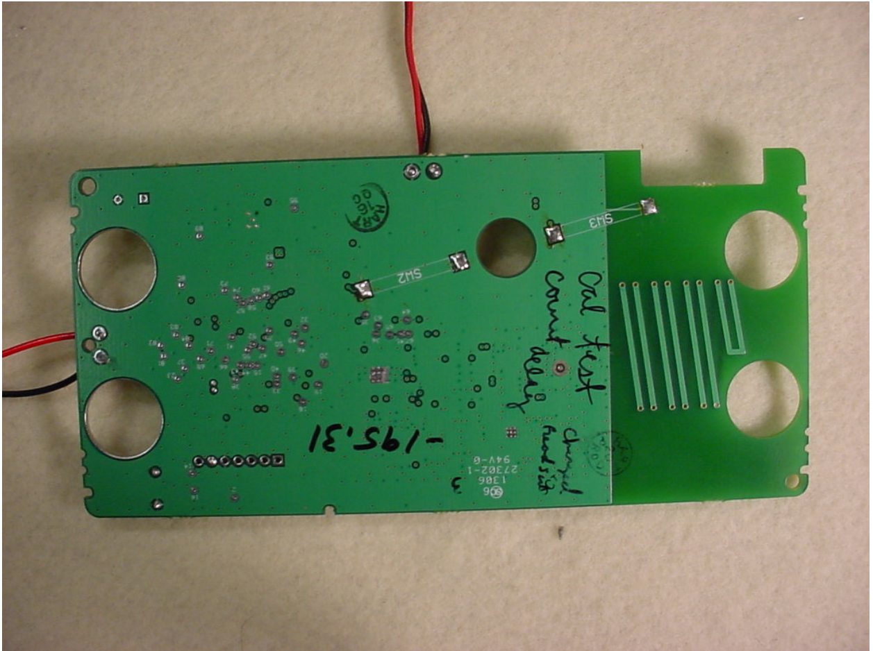
Figure 6: PCB 0217 Back
