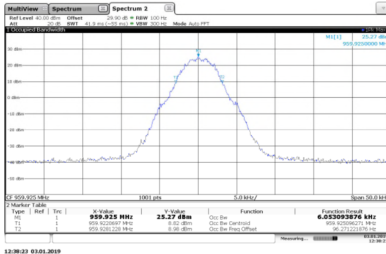
Figure 7.3.2-27: 959.925 MHz– m4Pass 10k Mode
