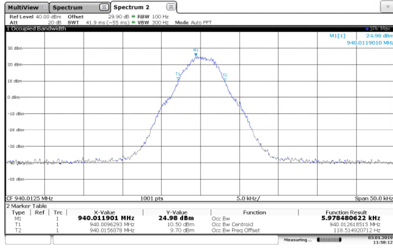
Figure 7.3.2-9: 940.0125 MHz – m4Pass 10k Mode
