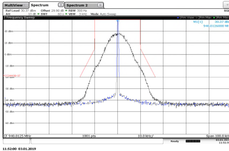
Figure 7.2.2-10: 940.0125 MHz – 25 kHz Channel Spacing – m4Pass20k Mode
