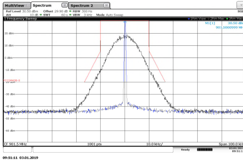
Figure 7.2.2-2: 901.5 MHz – 25 kHz Channel Spacing – 4FSK Mode
