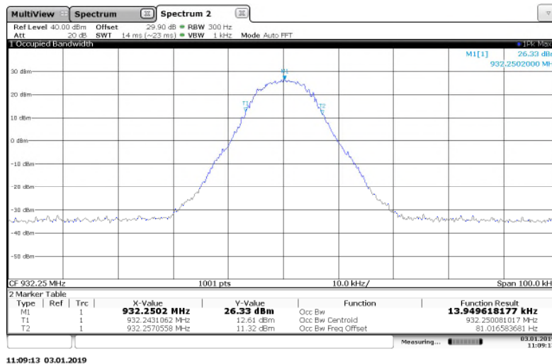
Figure 7.3.2-18: 932.25 MHz – 4FSK Mode
