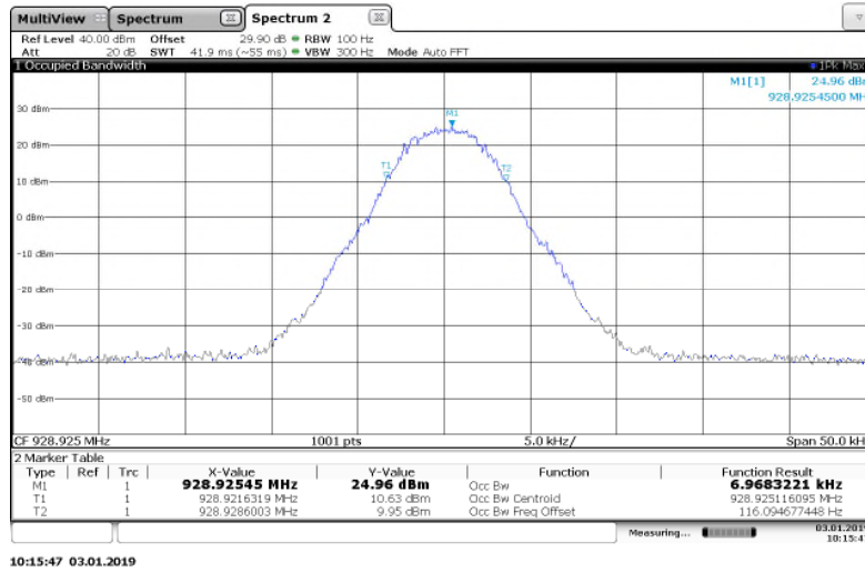
Figure 7.3.2-15: 928.925 MHz – 4FSK (Half Baud) Mode
