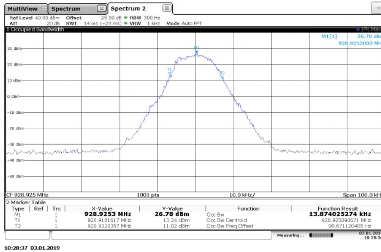
Figure 7.3.2-12: 928.925 MHz – 4FSK Mode
