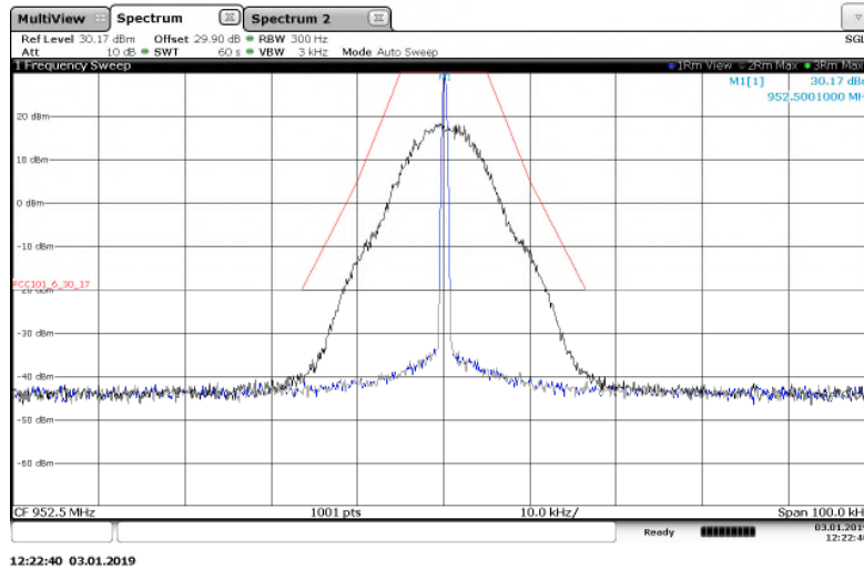
Figure 7.2.2-26: 952.5 MHz – 25 kHz Channel Spacing – m4Pass 20k Mode
