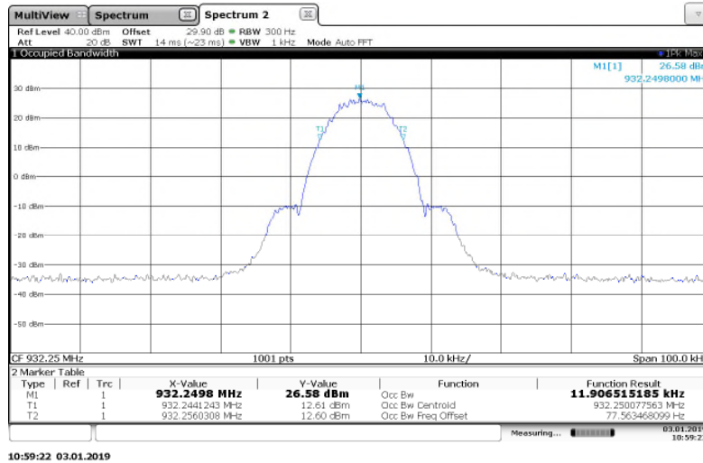
Figure 7.3.2-17: 932.25 MHz – 2FSK Mode
