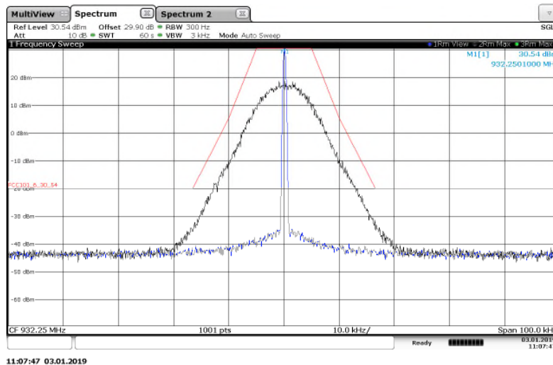
Figure 7.2.2-18: 932.25 MHz – 25 kHz Channel Spacing – 4FSK Mode
