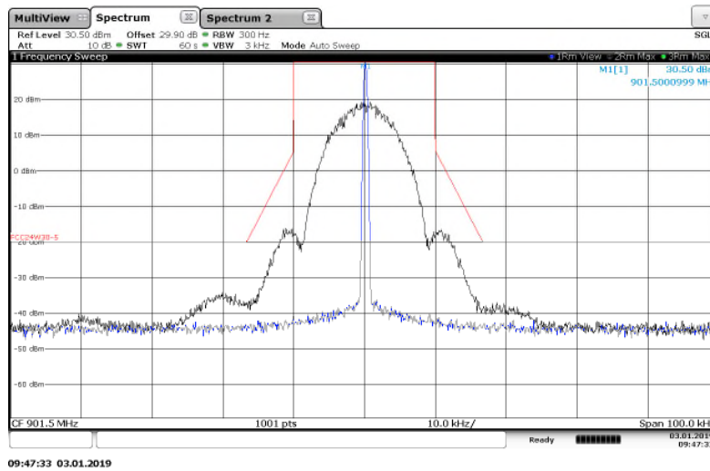
Figure 7.2.2-1: 901.5 MHz – 25 kHz Channel Spacing – 2FSK Mode
