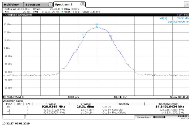
Figure 7.3.2-13: 928.925 MHz – 8FSK Mode
