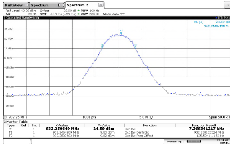
Figure 7.3.2-22: 932.25 MHz — 8FSK(Half Baud) Mode
