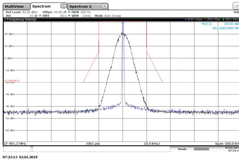
Figure 7.2.2-5: 901.5 MHz – 25 kHz Channel Spacing – 4SFSK (Half Baud) Mode
