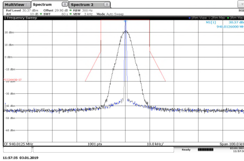
Figure 7.2.2-9: 940.0125 MHz – 25 kHz Channel Spacing – m4Pass10k Mode
