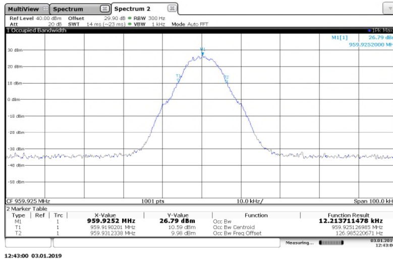
Figure 7.3.2-28: 959.925 MHz– m4Pass 20k Mode
