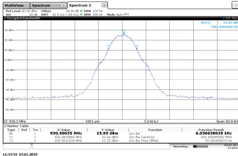
Figure 7.3.2-7: 930.5 MHz – m4Pass 10k Mode
