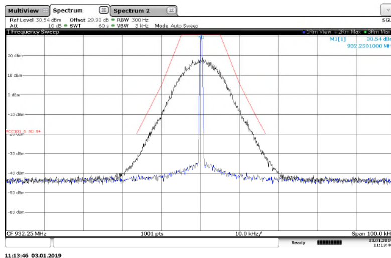
Figure 7.2.2-19: 932.25 MHz – 25 kHz Channel Spacing – 8FSK Mode
