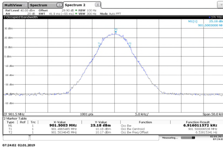
Figure 7.3.2-5: 901.5 MHz – 4SFSK (Half Baud) Mode
