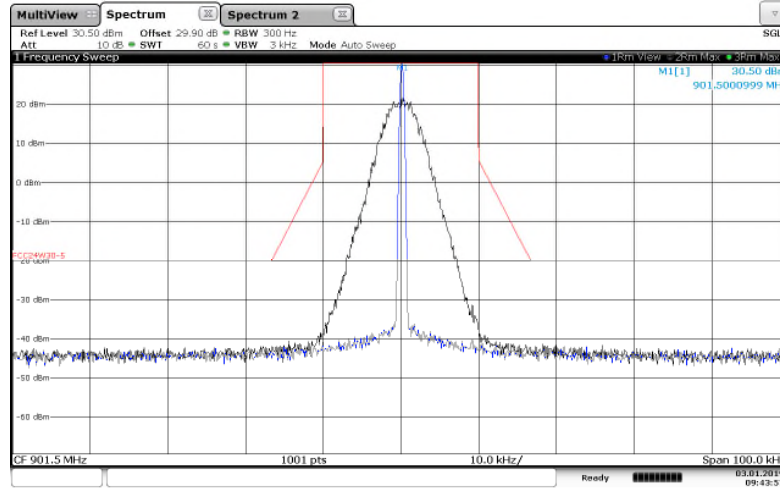
Figure 7.2.2-6: 901.5 MHz – 25 kHz Channel Spacing – 8SFSK (Half Baud) Mode
