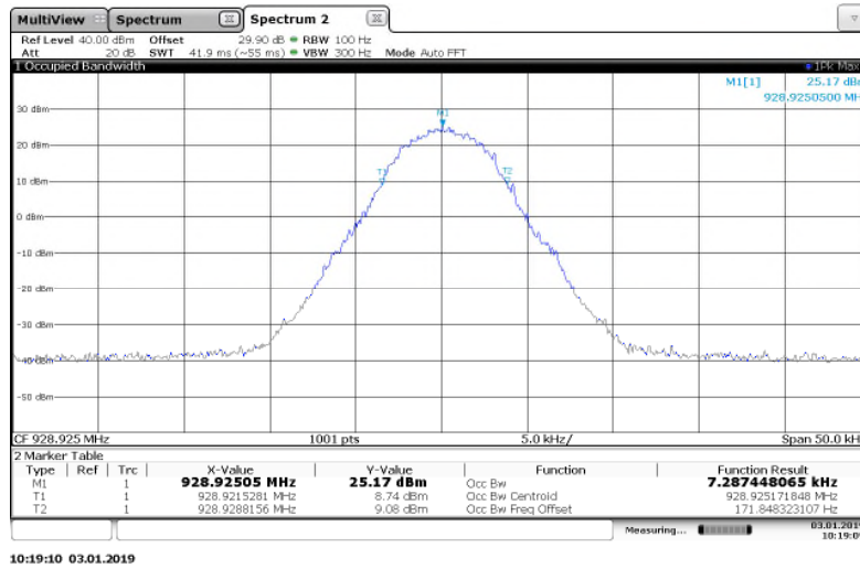
Figure 7.3.2-16: 928.925 MHz – 8FSK (Half Baud) Mode
