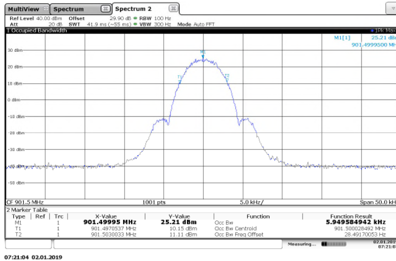
Figure 7.3.2-4: 901.5 MHz – 2SFSK (Half Baud) Mode
