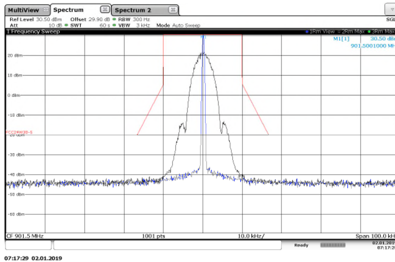
Figure 7.2.2-4: 901.5 MHz – 25 kHz Channel Spacing – 2SFSK (Half Baud) Mode
