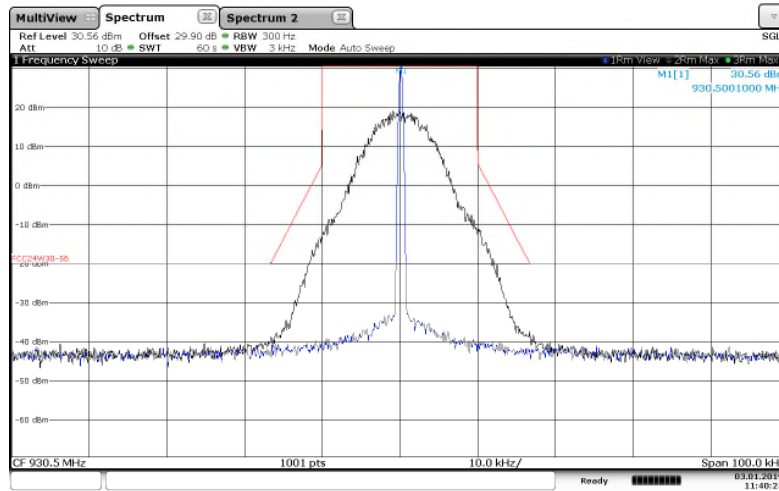
Figure 7.2.2-8: 930.5 MHz – 25 kHz Channel Spacing – m4Pass20k Mode
