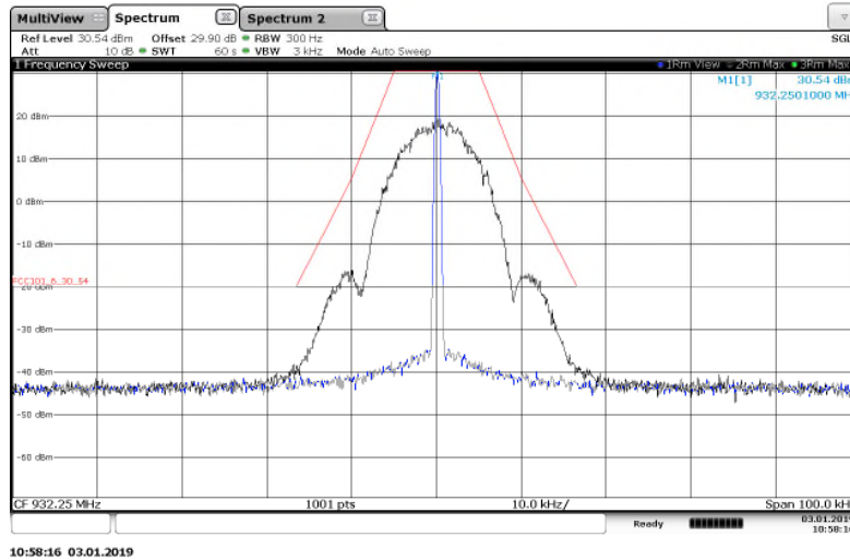
Figure 7.2.2-17: 932.25 MHz – 25 kHz Channel Spacing - 2FSK Mode
