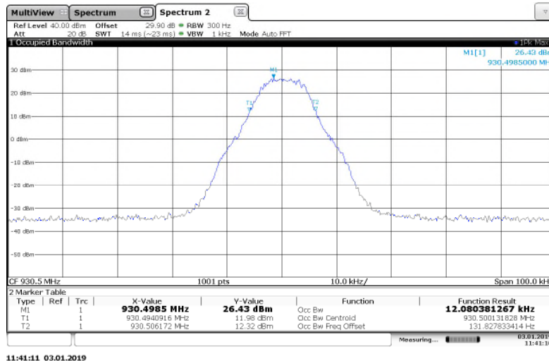
Figure 7.3.2-8: 930.5 MHz – m4Pass 20k Mode
