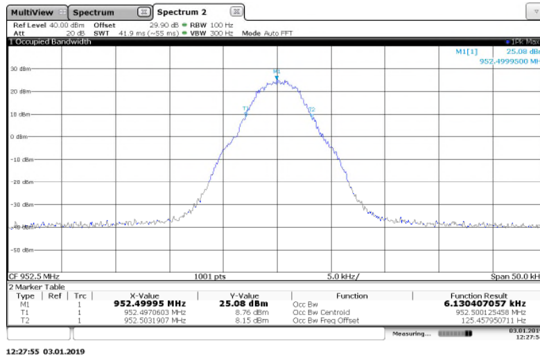
Figure 7.3.2-25: 952.5 MHz – m4Pass 10k Mode
