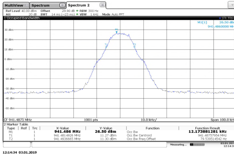
Figure 7.3.2-24: 941.4875 MHz – m4Pass 20k Mode
