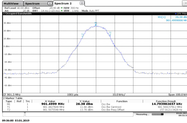
Figure 7.3.2-3: 901.5 MHz – 8FSK Mode
