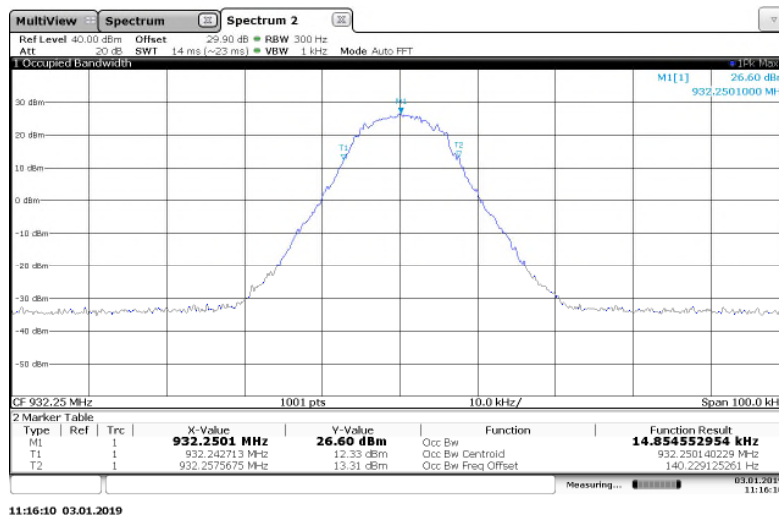
Figure 7.3.2-19: 932.25 MHz – 8FSK Mode
