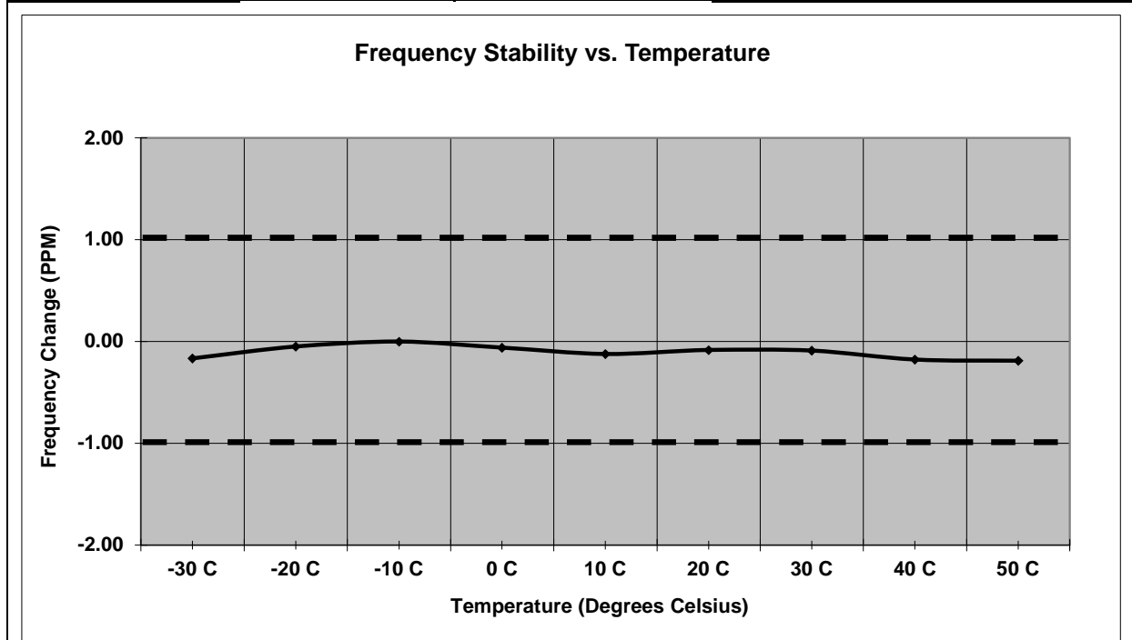
Figure 7.6.2-3: Frequency Stability – 930.5 MHz – KDS/CBA
