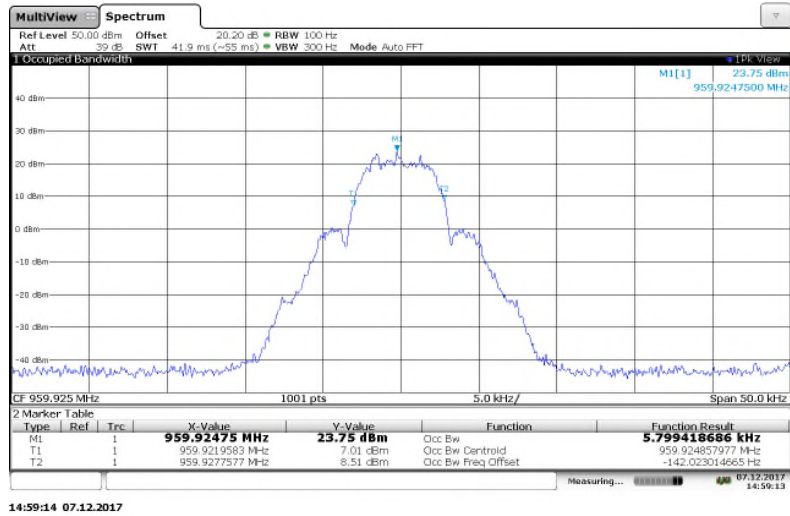
Figure 7.3.2-21: 959.925 MHz– mPass 5k Mode
