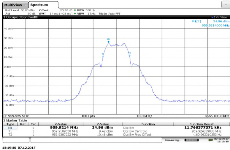
Figure 7.3.2-22: 959.925 MHz– mPass 10k Mode
