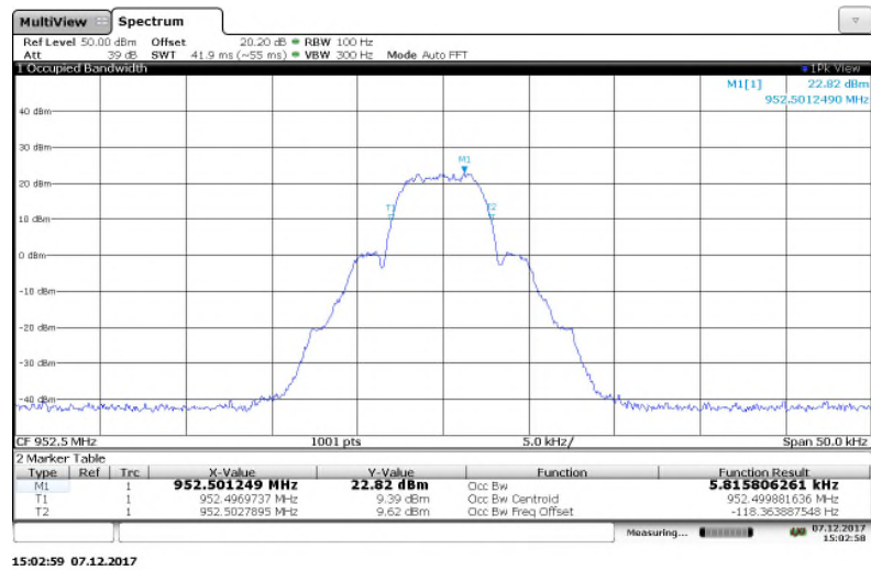
Figure 7.3.2-19: 952.5 MHz – MPass 5k Mode
