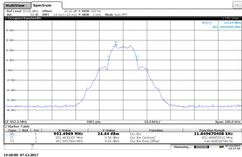
Figure 7.3.2-20: 952.5 MHz – MPass 10k Mode
