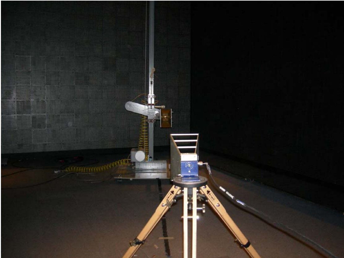
Figure 3: Radiated Emissions – Substitution
