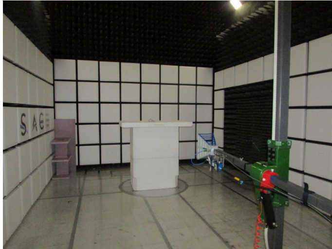
Figure 3: Radiated Emissions – Front – Above 1GHz- XPOS
