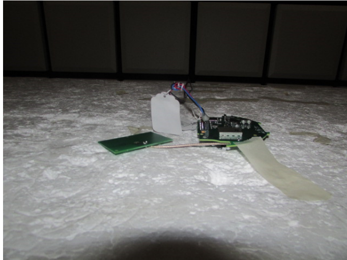
Figure 5: Radiated Emissions – Front – Above 1GHz – XPOS
