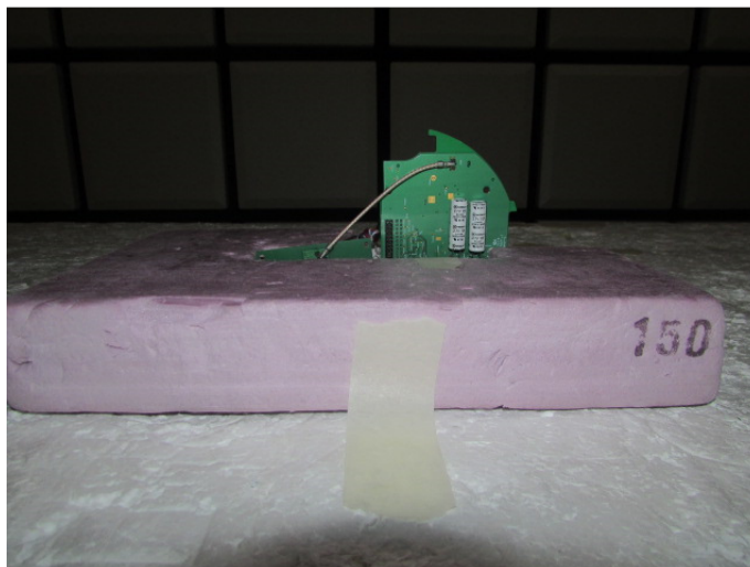
Figure 7: Radiated Emissions – Front – Above 1GHz – ZPOS
