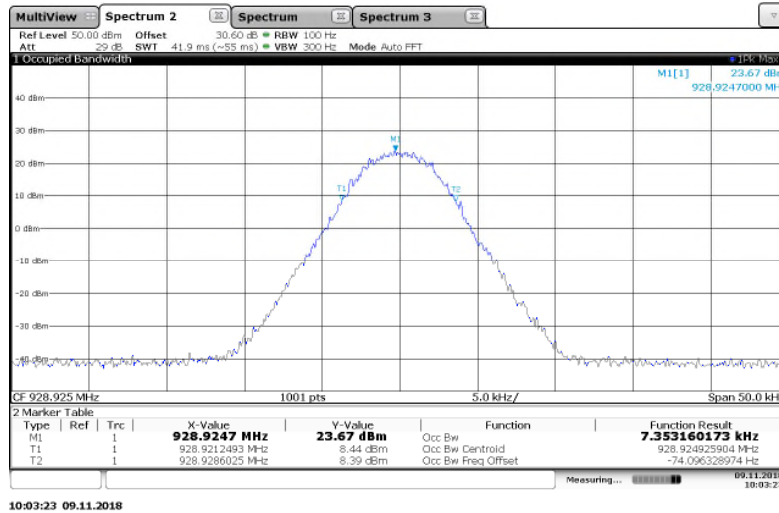
Figure 7.3.2-25: 928.925 MHz – 8FSK (Half Baud) Mode
