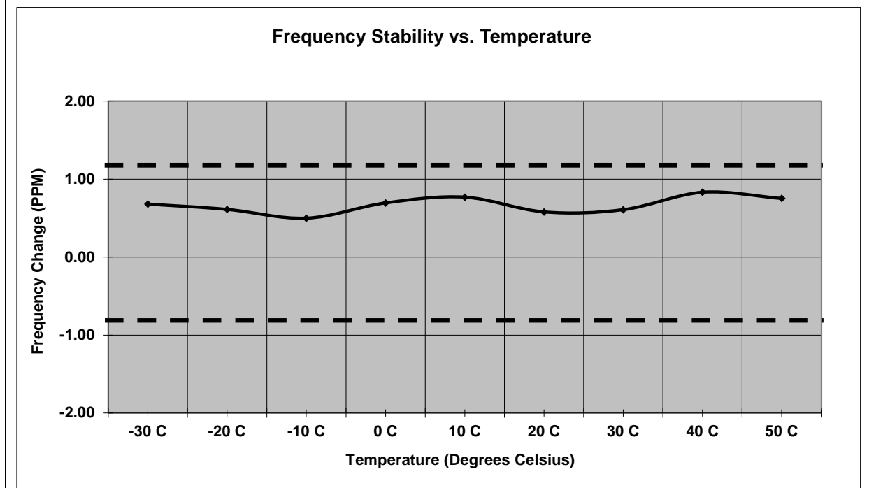
Figure 7.6.2-8: Frequency Stability – 959.925 MHz – TXC
