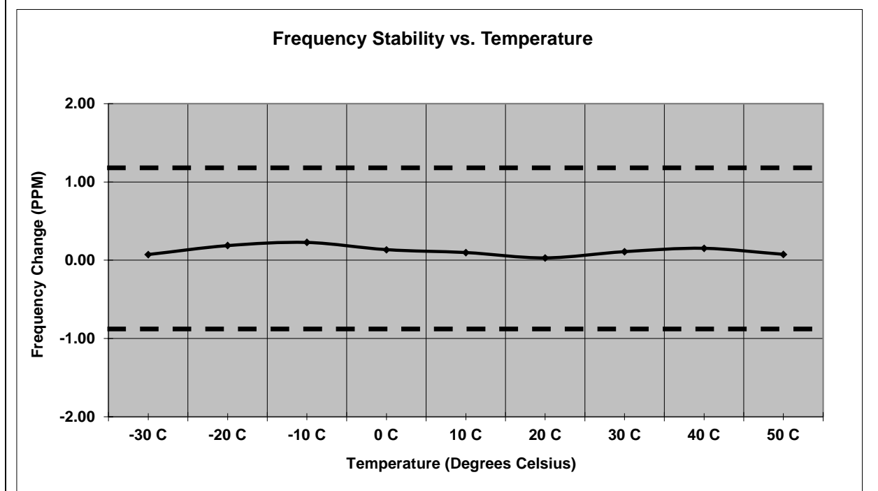
Figure 7.6.2-4: Frequency Stability – 930.5 MHz – KDS
