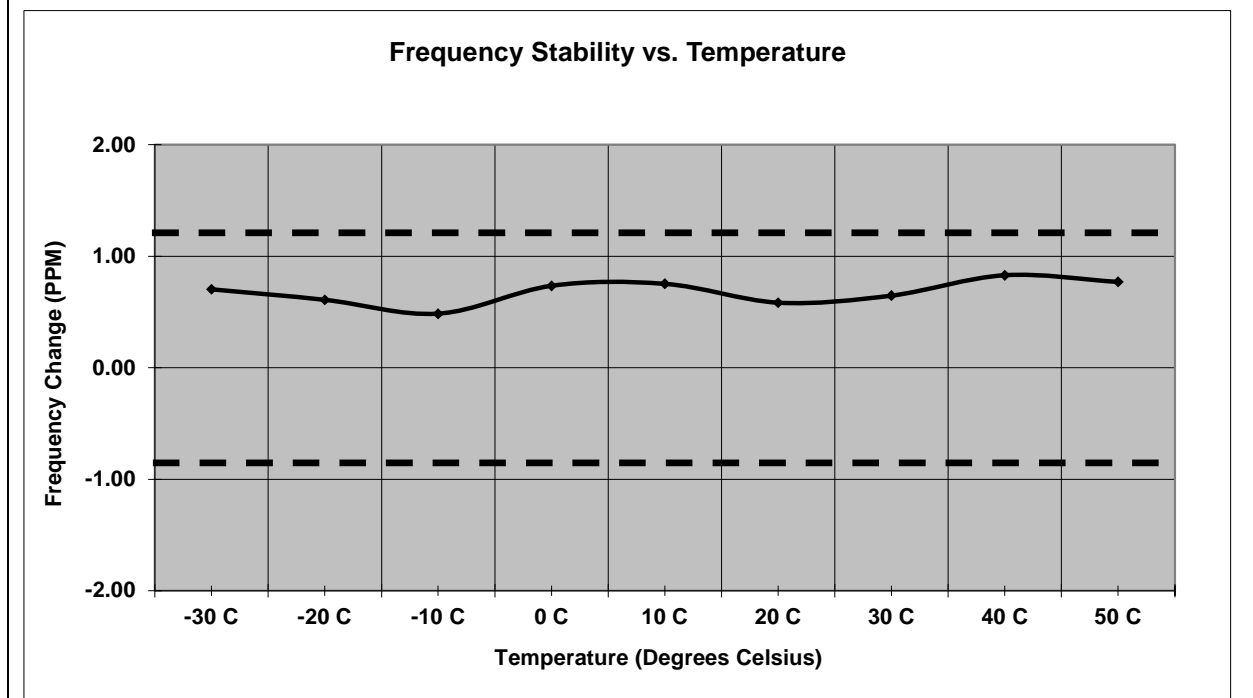
Figure 7.6.2-5: Frequency Stability – 930.5 MHz – TXC
