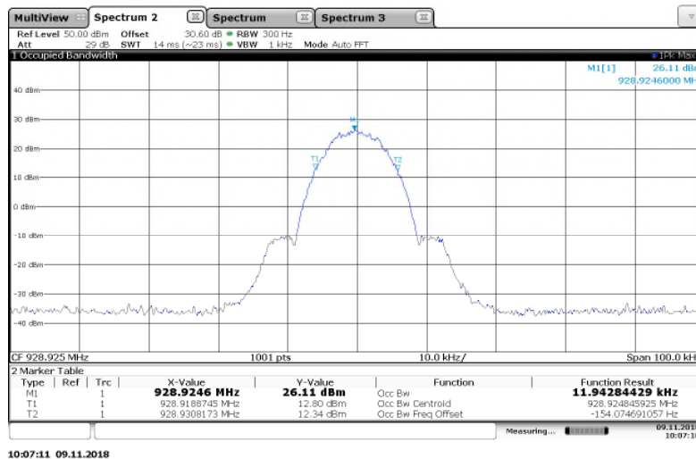
Figure 7.3.2-26: 928.925 MHz – 2SFSK Mode
