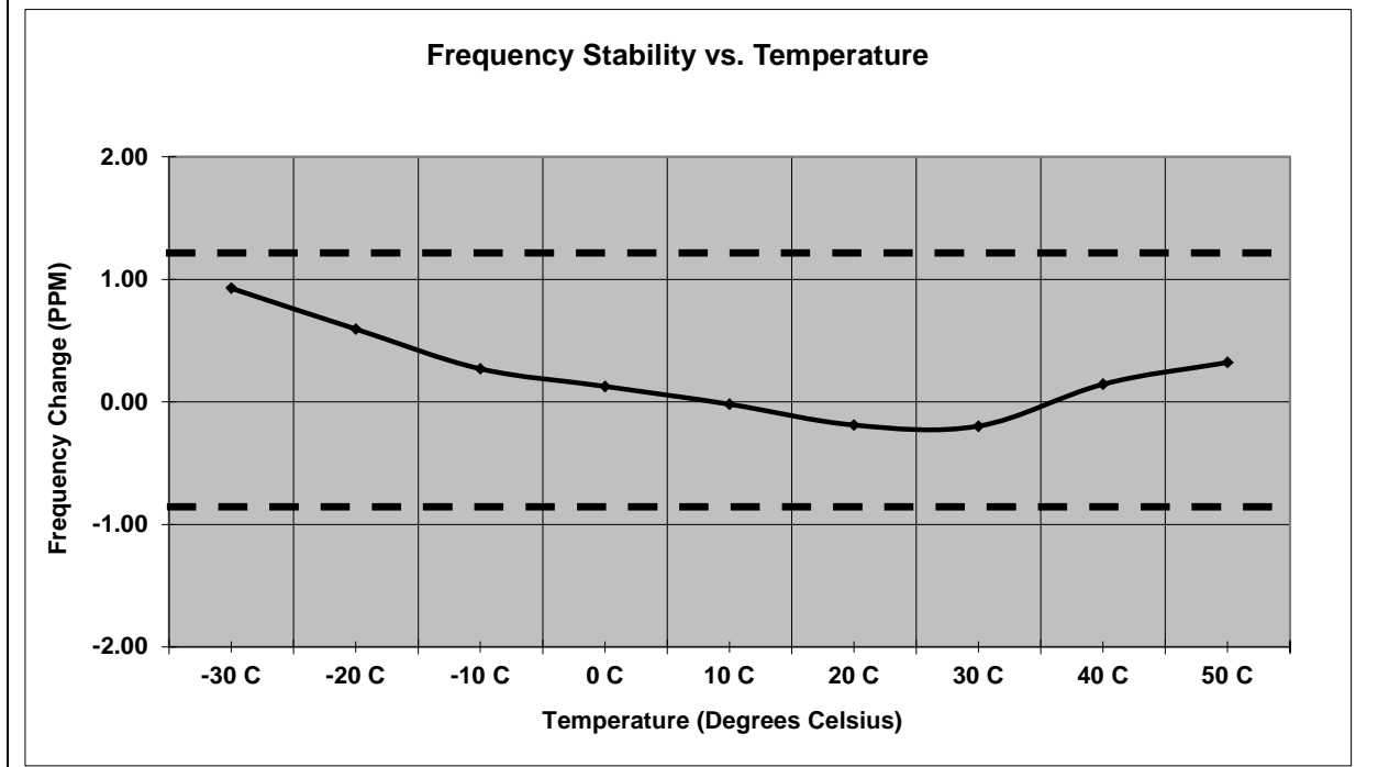
Figure 7.6.2-6: Frequency Stability – 930.5 MHz – EPSON
