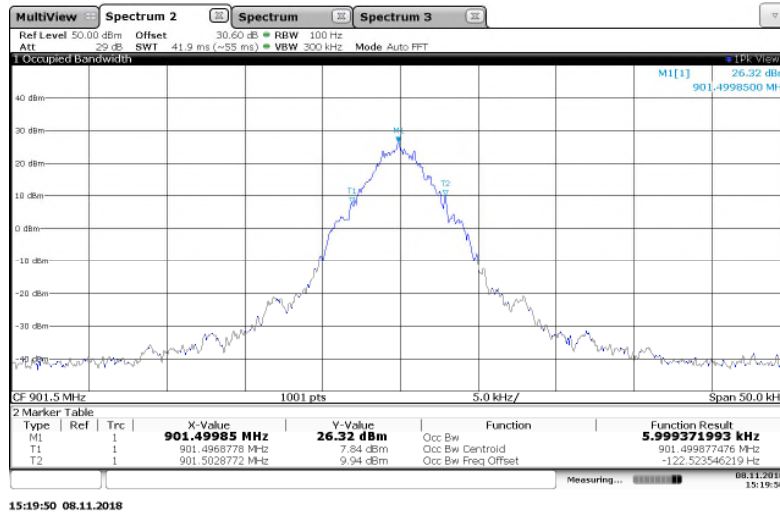
Figure 7.3.2-3: 901.5 MHz – C&I (Half Baud) Mode
