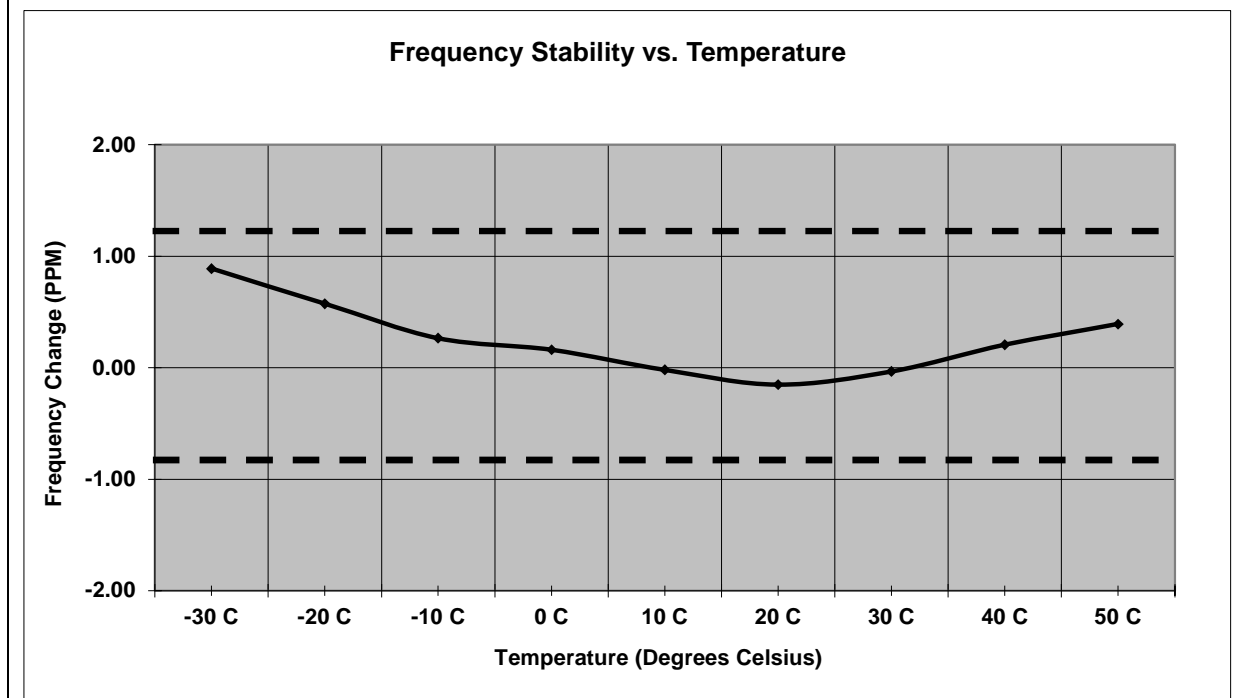
Figure 7.6.2-3: Frequency Stability – 901.5 MHz – EPSON
