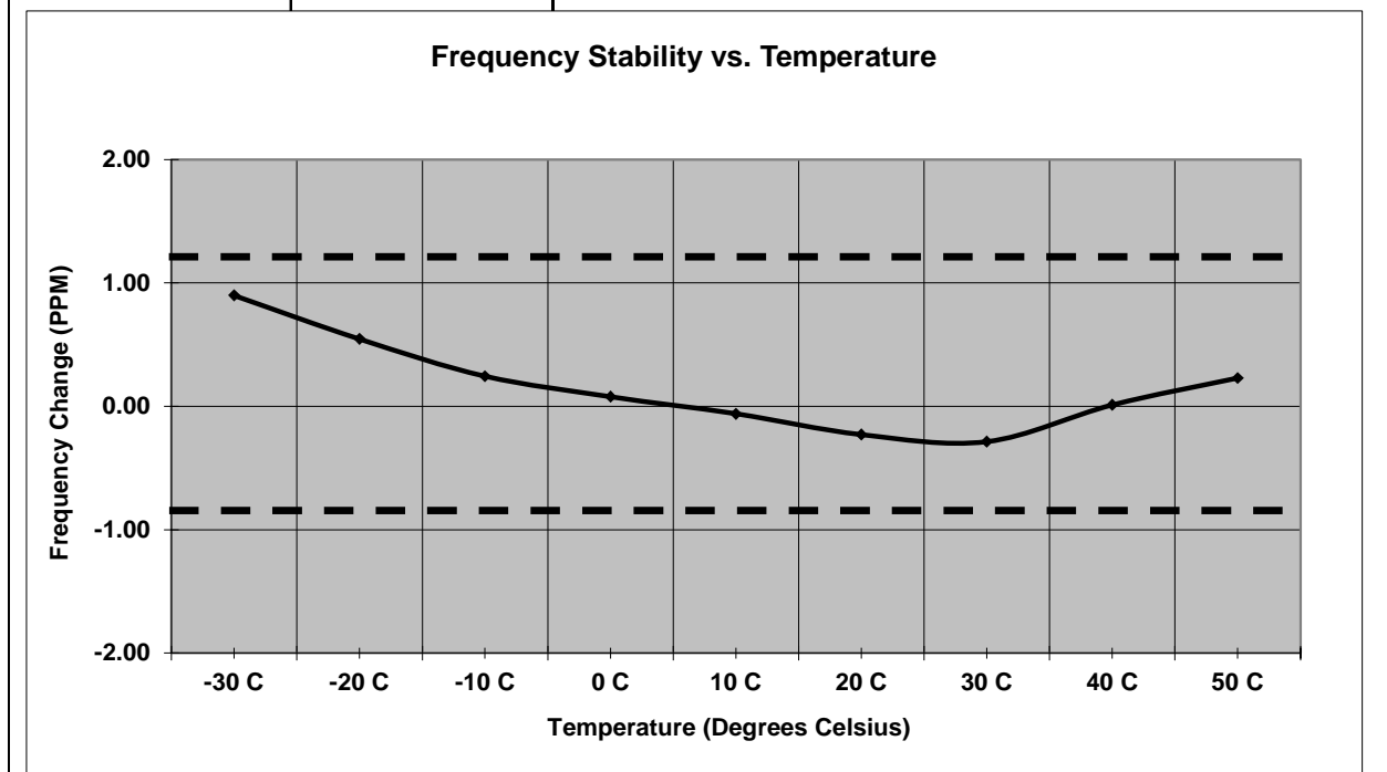
Figure 7.6.2-9: Frequency Stability – 959.925 MHz – EPSON
