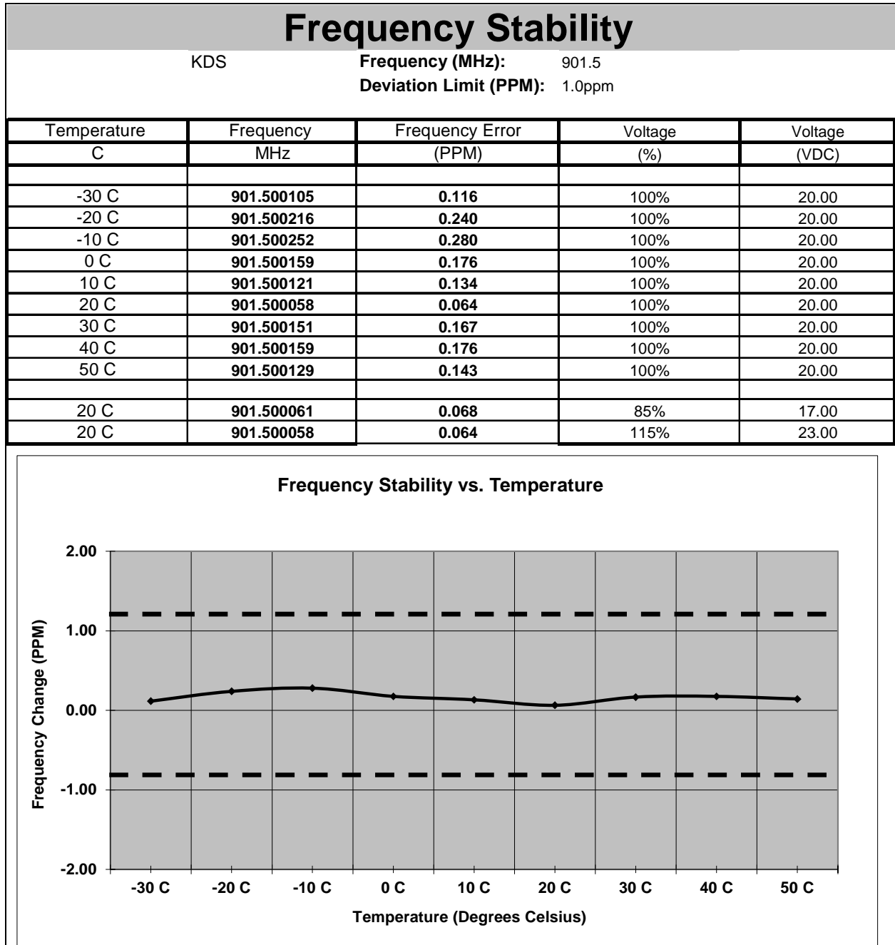
Figure 7.6.2-1: Frequency Stability – 901.5 MHz – KDS
