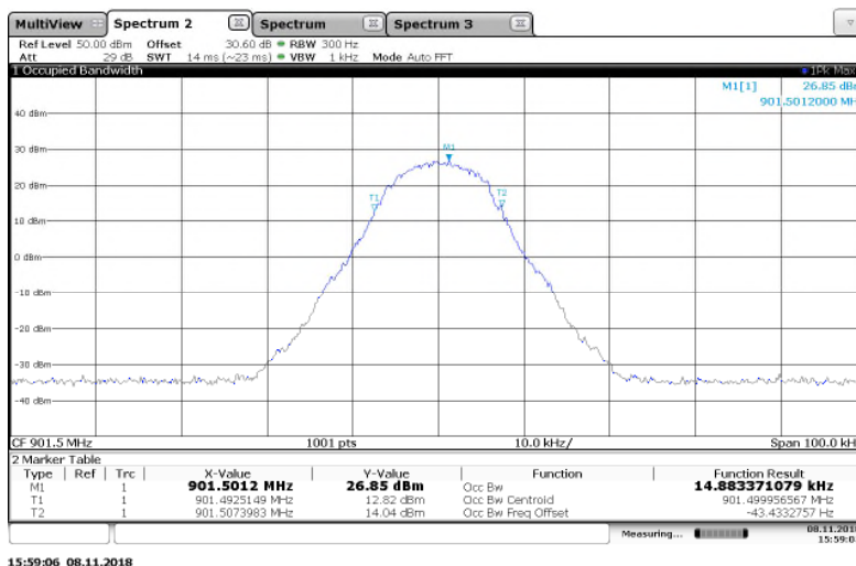
Figure 7.3.2-10: 901.5 MHz – 8SFSK Mode
