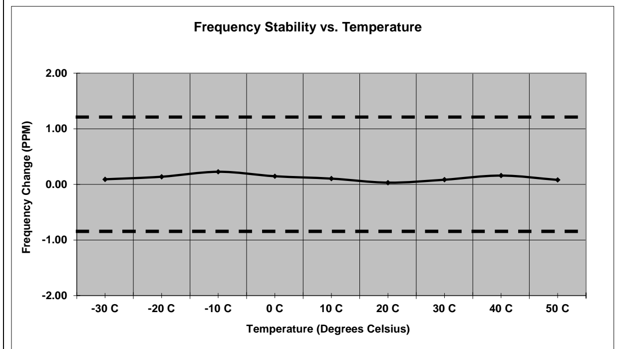
Figure 7.6.2-7: Frequency Stability – 959.925 MHz – KDS
