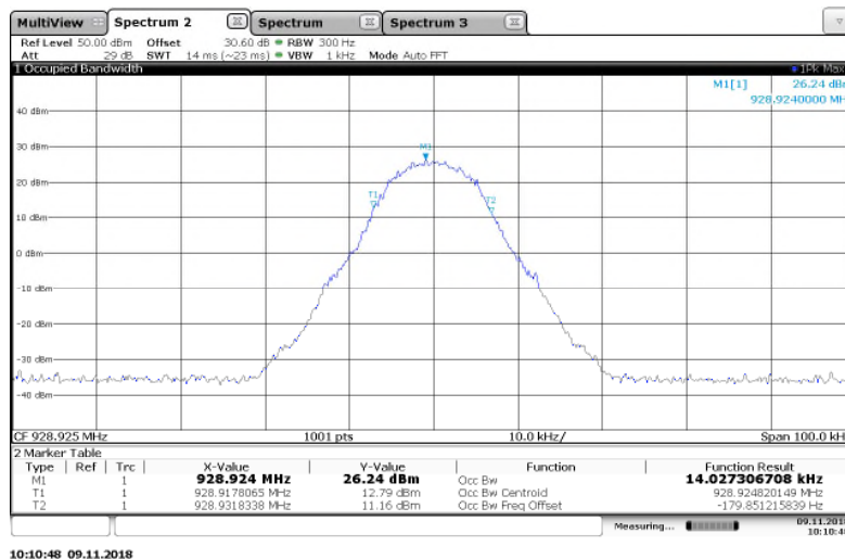
Figure 7.3.2-27: 928.925 MHz – 4SFSK Mode
