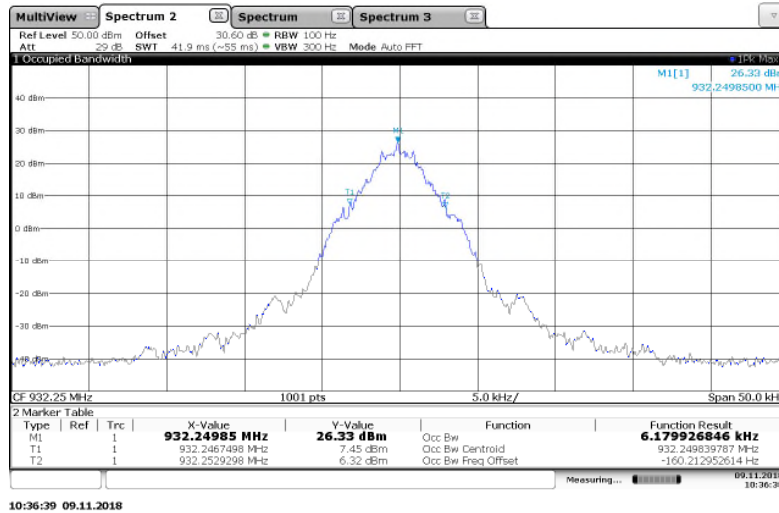
Figure 7.3.2-31: 932.25 MHz – C&I (Half Baud) Mode
