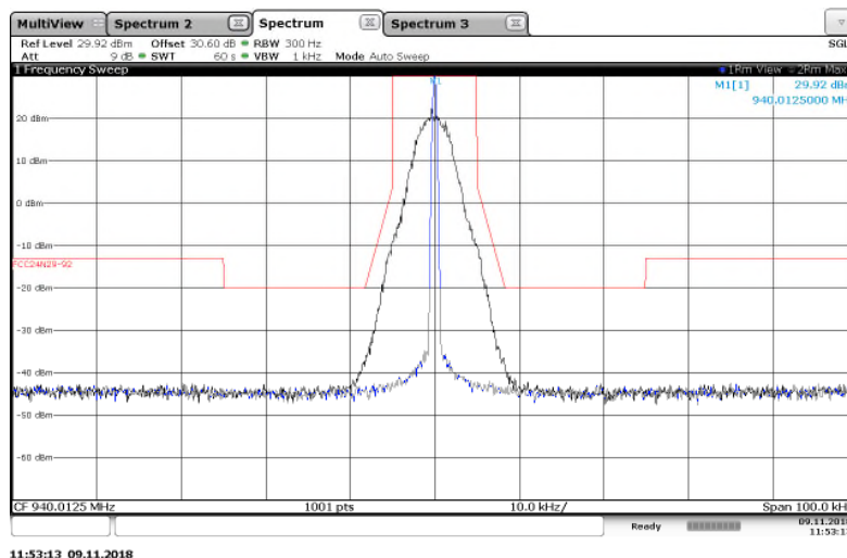
Figure 7.2.2-17: 940.0125 MHz – 25 kHz Channel Spacing – m4Pass 10k Mode
