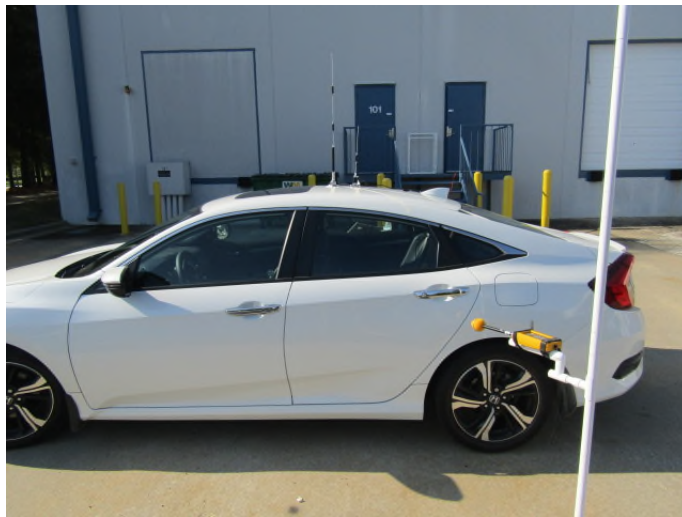
Figure 2 – Bystander at 30 degrees - Test Set-up
