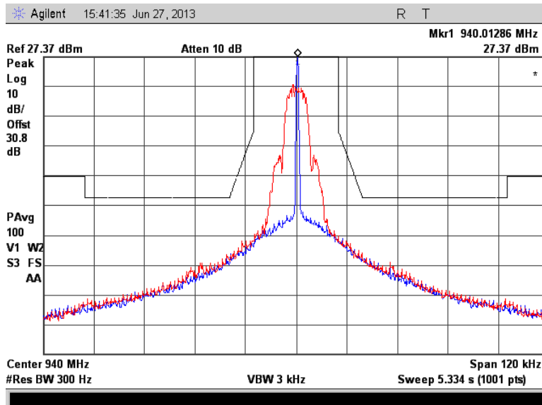
Figure 7.2.2-14: 940.0125 MHz – 25 kHz Channel Spacing – mPass 5k Mode
