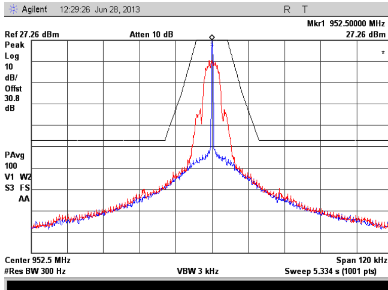
Figure 7.2.2-34: 952.5 MHz – mPass 5k Mode
