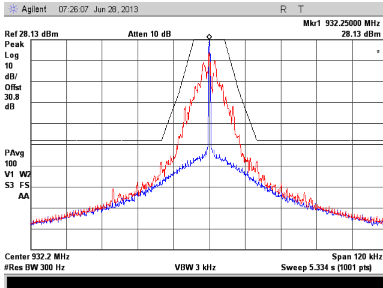
Figure 7.2.2-24: 932.25 MHz – Normal Mode
