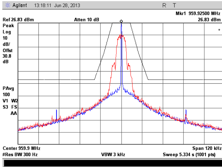
Figure 7.2.2-36: 959.925 MHz – mPass 5k Mode
