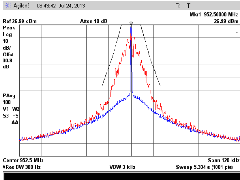
Figure 7.2.2-32: 952.5 MHz – Normal Mode
