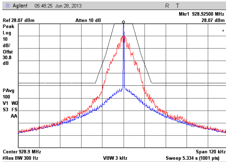
Figure 7.2.2-17: 928.925 MHz – Double Density Mode
