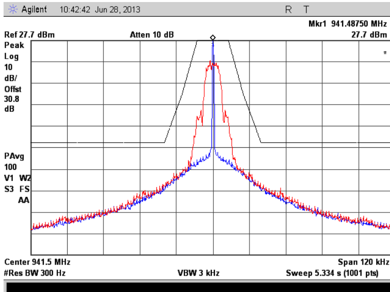
Figure 7.2.2-28: 941.4875 MHz – mPass 5k Mode
