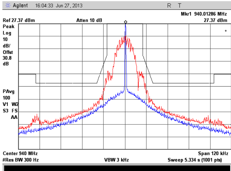
Figure 7.2.2-15: 940.0125 MHz – 25 kHz Channel Spacing – mPass 10k Mode
