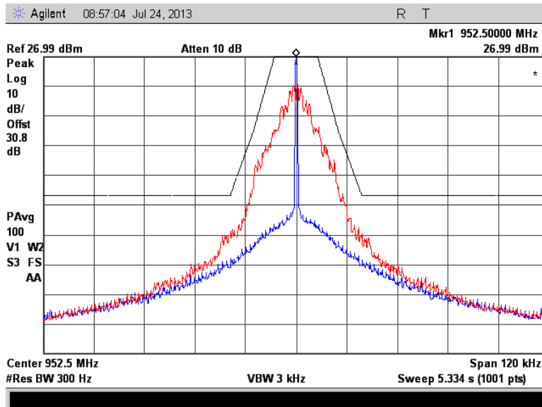
Figure 7.2.2-31: 952.5 MHz – Double Density Mode
