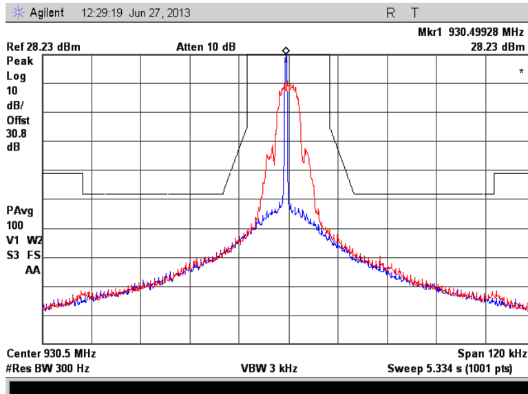
Figure 7.2.2-11: 930.5 MHz – 25 kHz Channel Spacing – mPass 5k Mode
