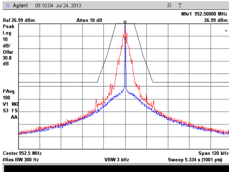
Figure 7.2.2-30: 952.5 MHz – C&I Mode
