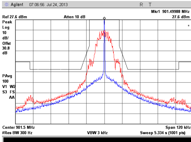
Figure 7.2.2-9: 901.5 MHz – 25 kHz Channel Spacing – mPass10k Mode
