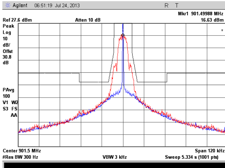
Figure 7.2.2-7: 901.5 MHz – 12.5 kHz Channel Spacing – mPass5k Mode
