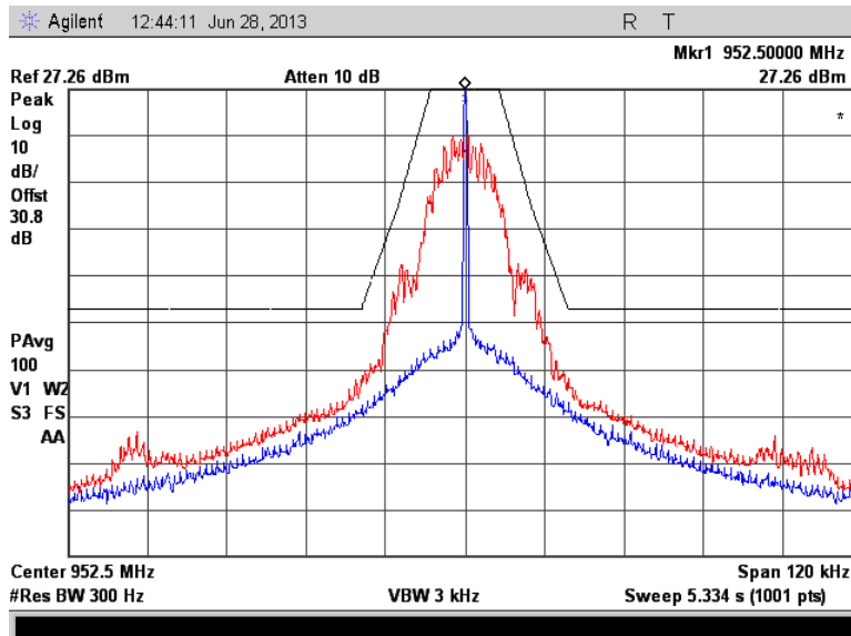
Figure 7.2.2-35: 952.5 MHz – mPass 10k Mode
