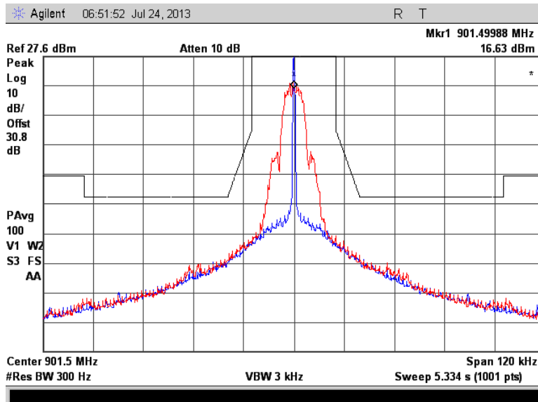
Figure 7.2.2-8: 901.5 MHz – 25 kHz Channel Spacing – mPass5k Mode
