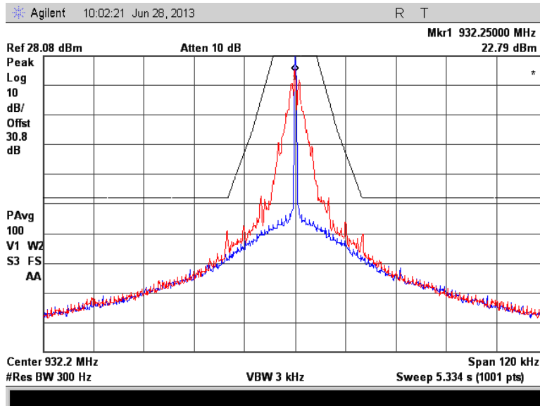
Figure 7.2.2-22: 932.25 MHz – C&I Mode
