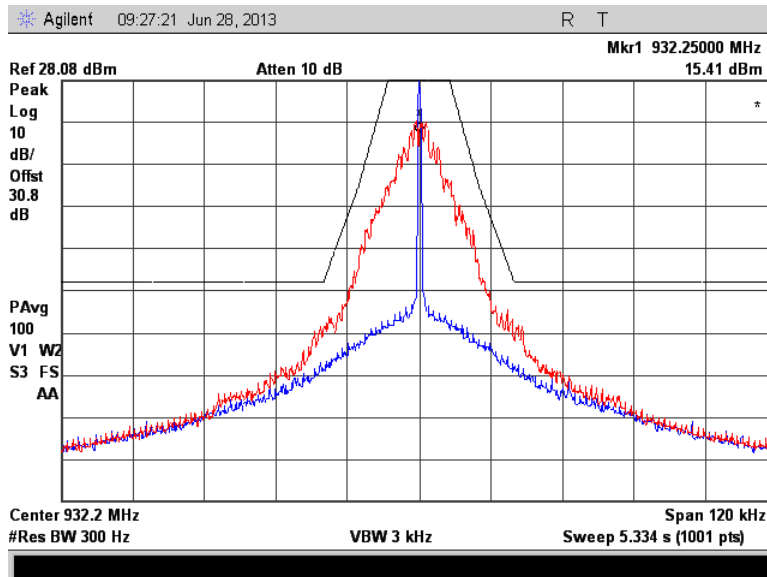
Figure 7.2.2-23: 932.25 MHz – Double Density Mode
