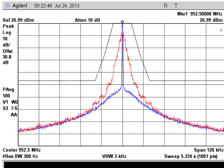
Figure 7.2.2-33: 952.5 MHz – Priority Mode
