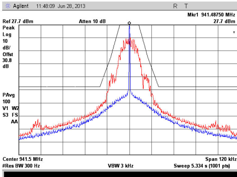
Figure 7.2.2-29: 941.4875 MHz – mPass 10k Mode
