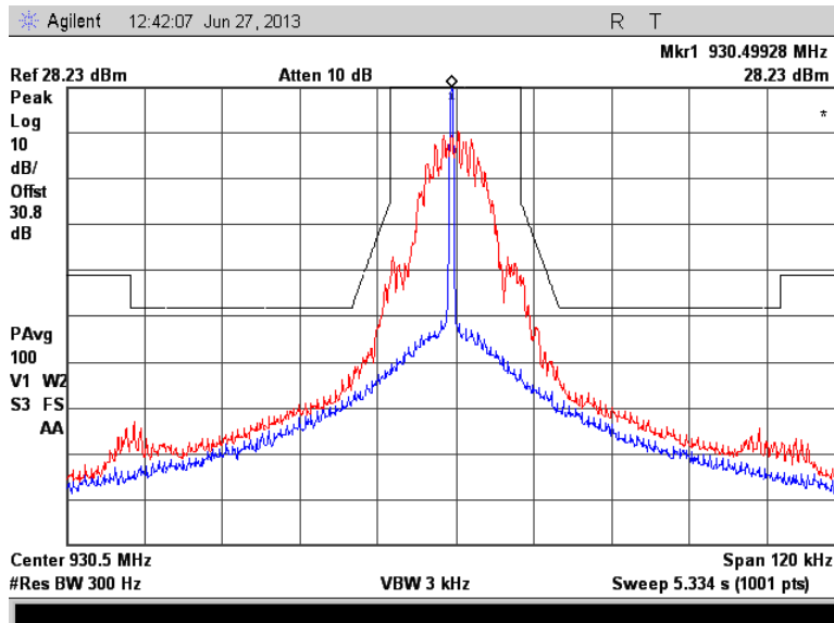
Figure 7.2.2-12: 930.5 MHz – 25 kHz Channel Spacing – mPass 10k Mode
