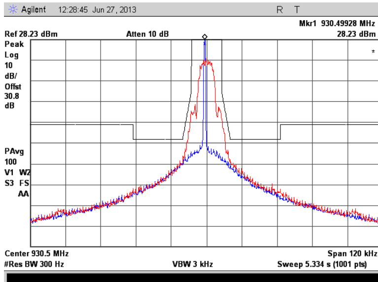
Figure 7.2.2-10: 930.5 MHz – 12.5 kHz Channel Spacing – mPass 5k Mode
