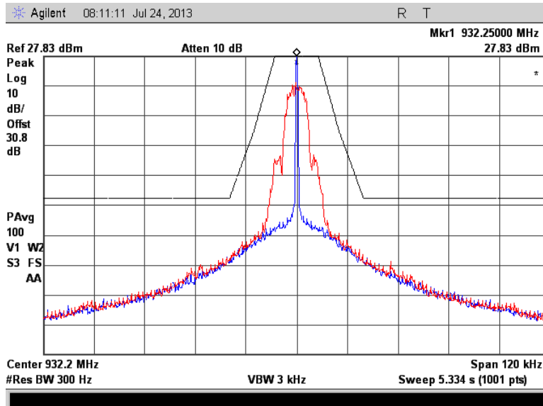
Figure 7.2.2-26: 932.25 MHz – mPass5k Mode
