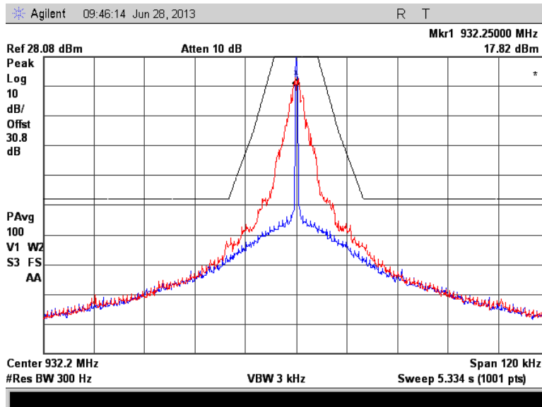
Figure 7.2.2-25: 932.25 MHz — Priority Mode
