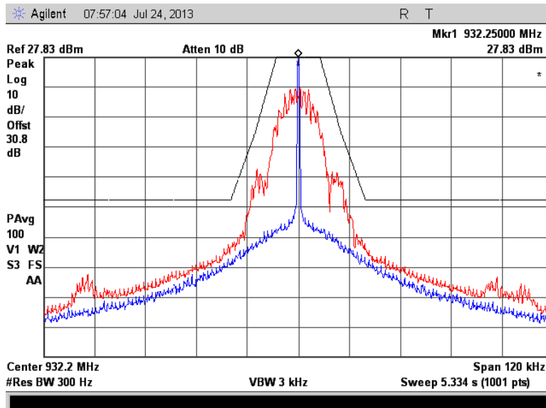
Figure 7.2.2-27: 932.25 MHz – mPass10k Mode
