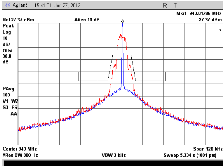
Figure 7.2.2-13: 940.0125 MHz – 12.5 kHz Channel Spacing – mPass 5k Mode
