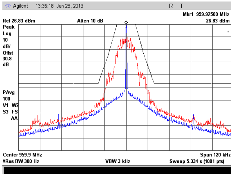
Figure 7.2.2-37: 959.925 MHz – mPass 10k Mode
