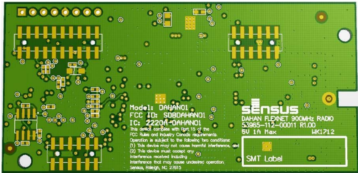
Figure 2: Compliance information location on DAHAN01 Radio Module PCB
