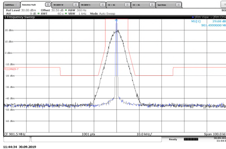
Figure 7.2.2-6: 901.5 MHz – 12.5 kHz Channel Spacing – 4SFSK (Half Baud) Mode
