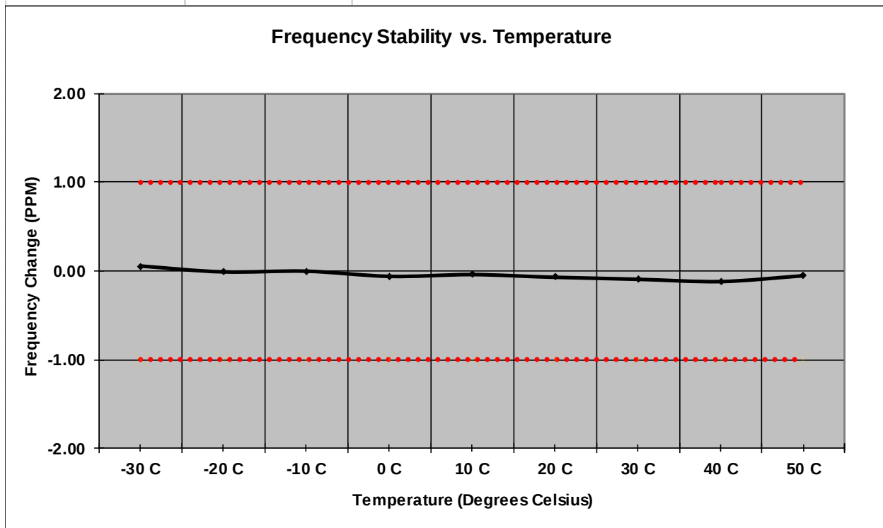
Figure 7.6.2-1: Frequency Stability – 901.5 MHz
