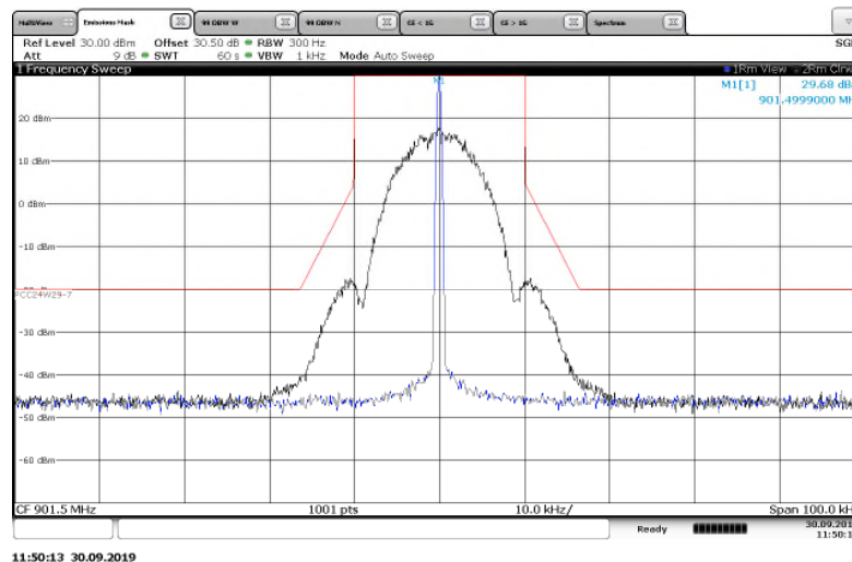
Figure 7.2.2-8: 901.5 MHz – 25 kHz Channel Spacing – 2SFSK Mode
