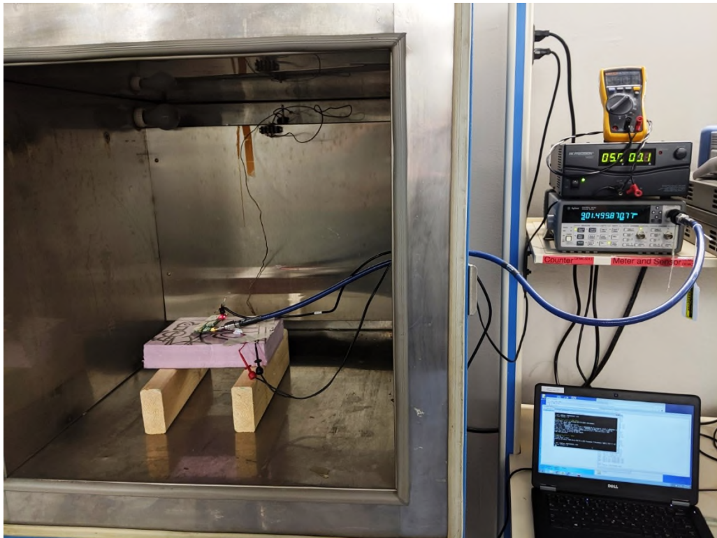
Figure 9: Frequency Stability
