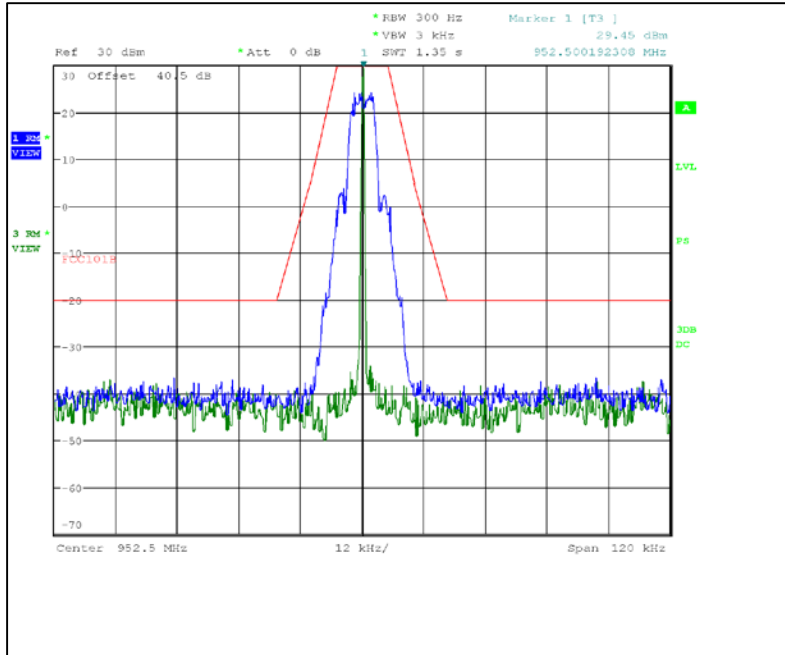
Figure 7.2.2-23: 952.5 MHz – mPass 5k Mode
