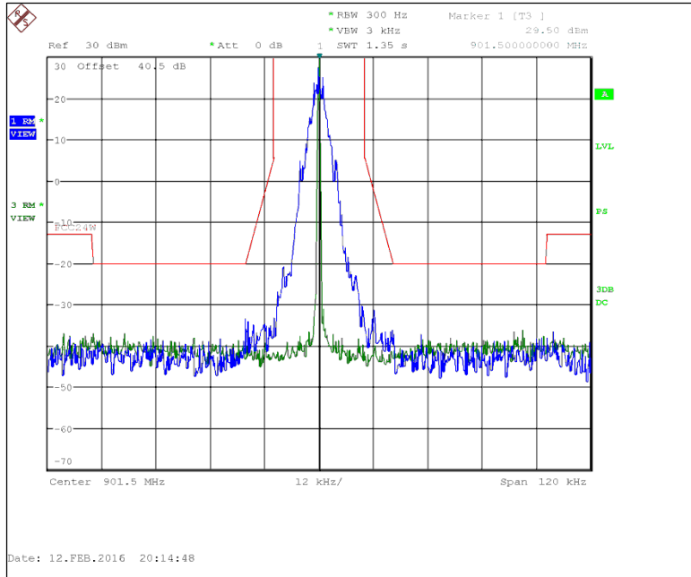
Figure 7.2.2-5: 901.5 MHz – 25 kHz Channel Spacing – C&I Mode
