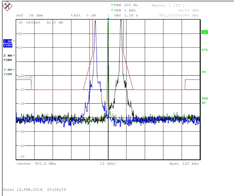
Figure 7.2.2-3: 901.5 MHz – 25 kHz Channel Spacing – Boost Mode
