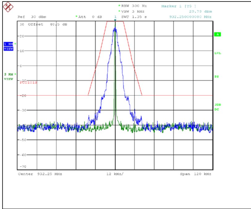
Figure 7.2.2-18: 932.25 MHz – C&I Mode
