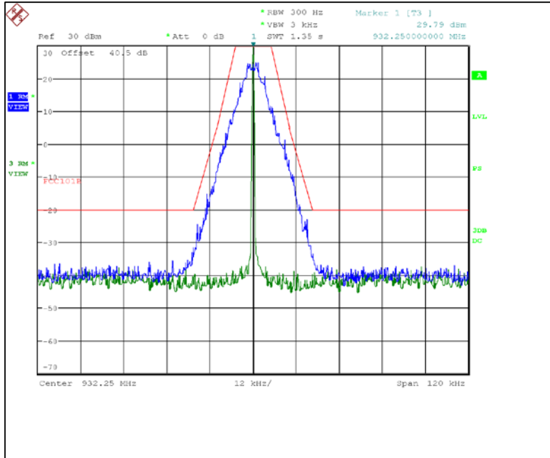
Figure 7.2.2-19: 932.25 MHz – Double Density Mode
