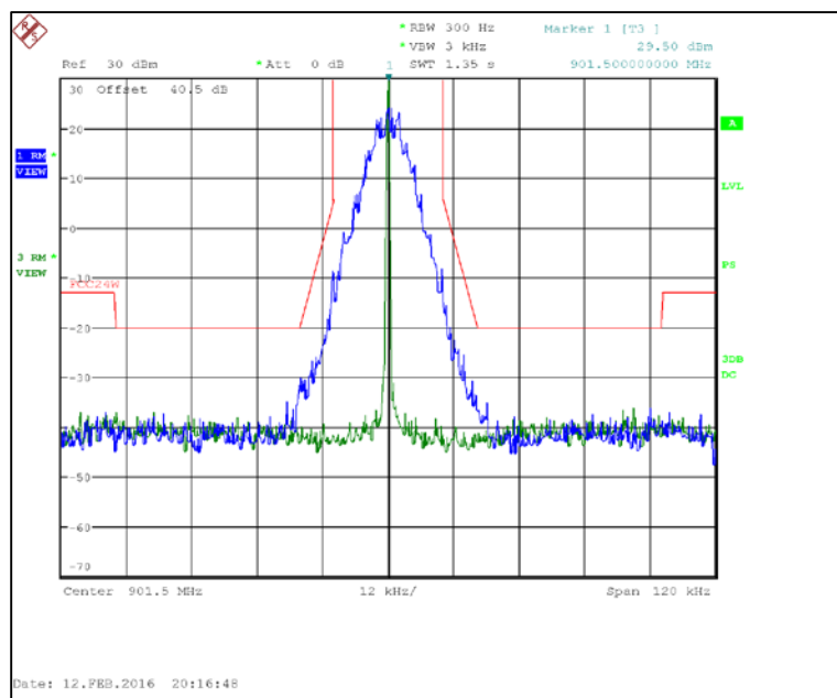
Figure 7.2.2-2: 901.5 MHz – 25 kHz Channel Spacing – Normal Mode
