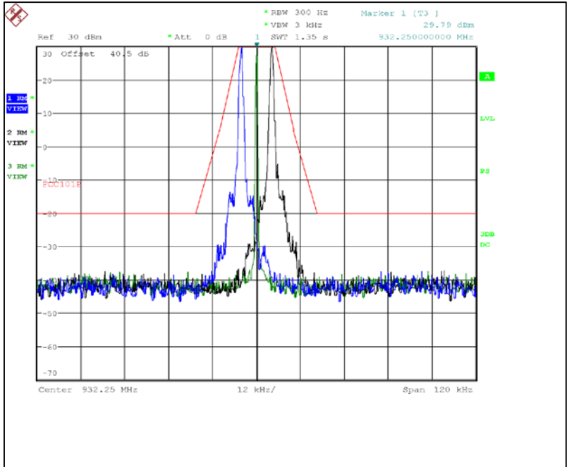
Figure 7.2.2-17: 932.25 MHz – Boost Mode
