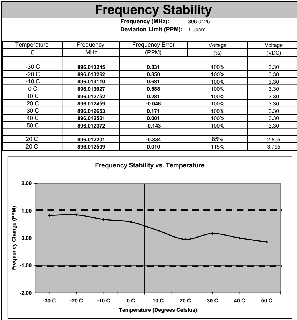
Figure 7.5.2-3: Frequency Stability – 896.0125MHz
