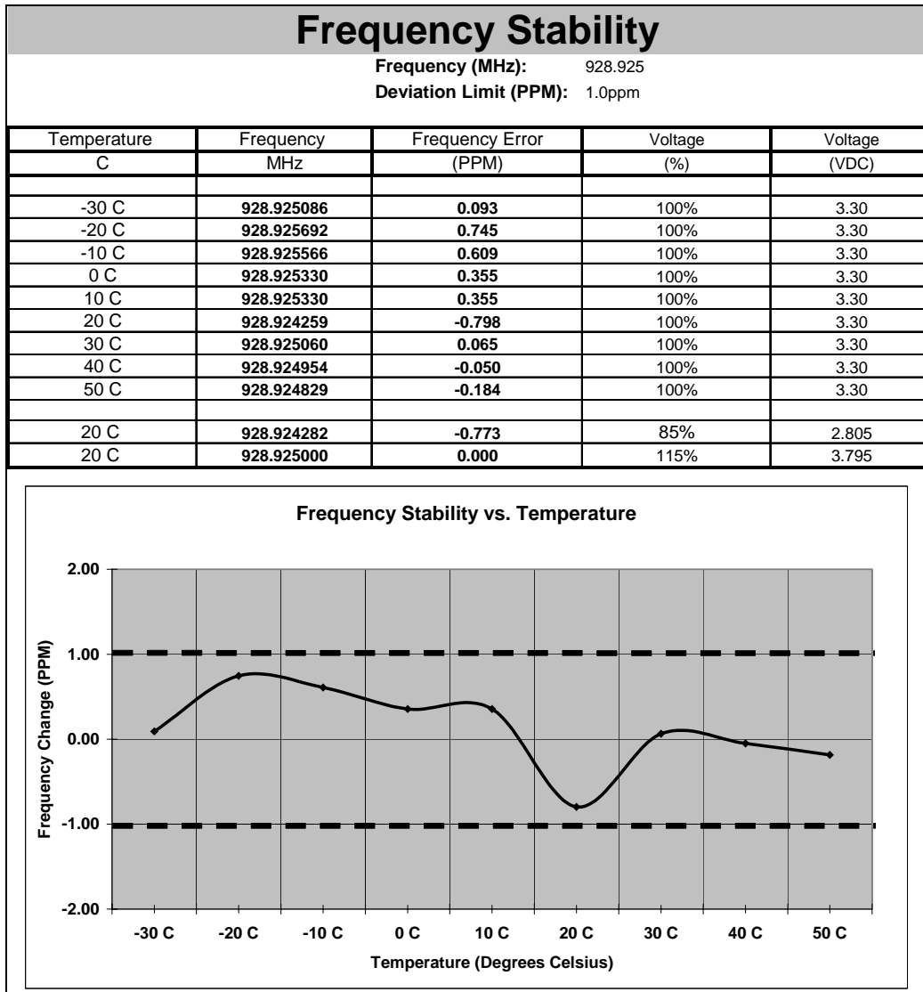
Figure 7.5.2-5: Frequency Stability – 928.925MHz
