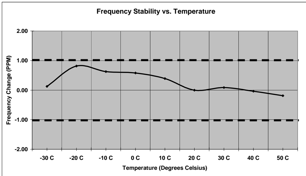
Figure 7.5.2-4: Frequency Stability – 935.0125MHz
