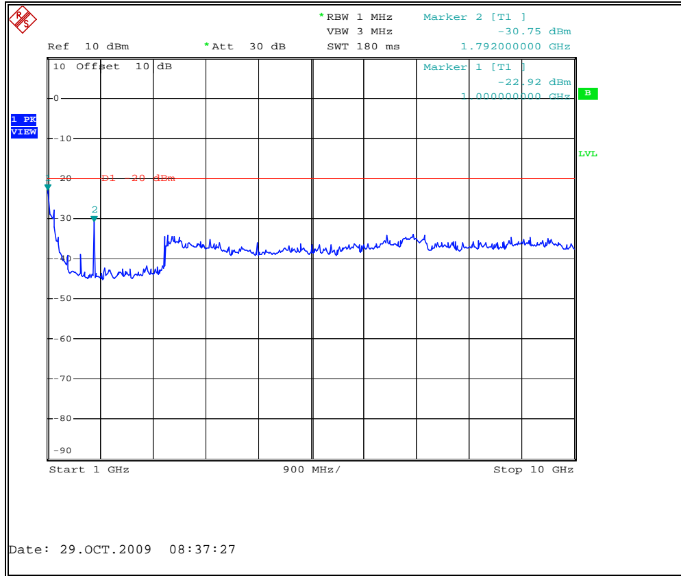
Figure 7.3.2-6: 896.05 MHz – 1GHz to 10GHz
