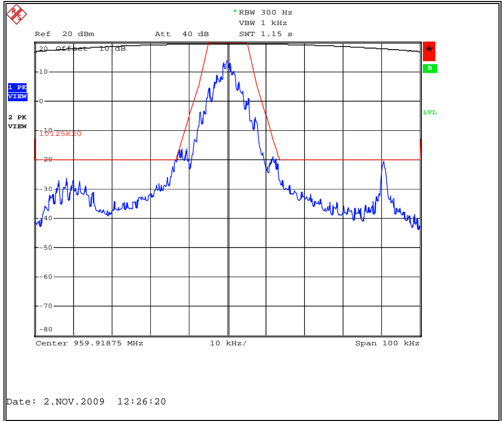
Figure 7.2.2-31: MPass Mode 12.5Kbps – 959. 91875 MHz
