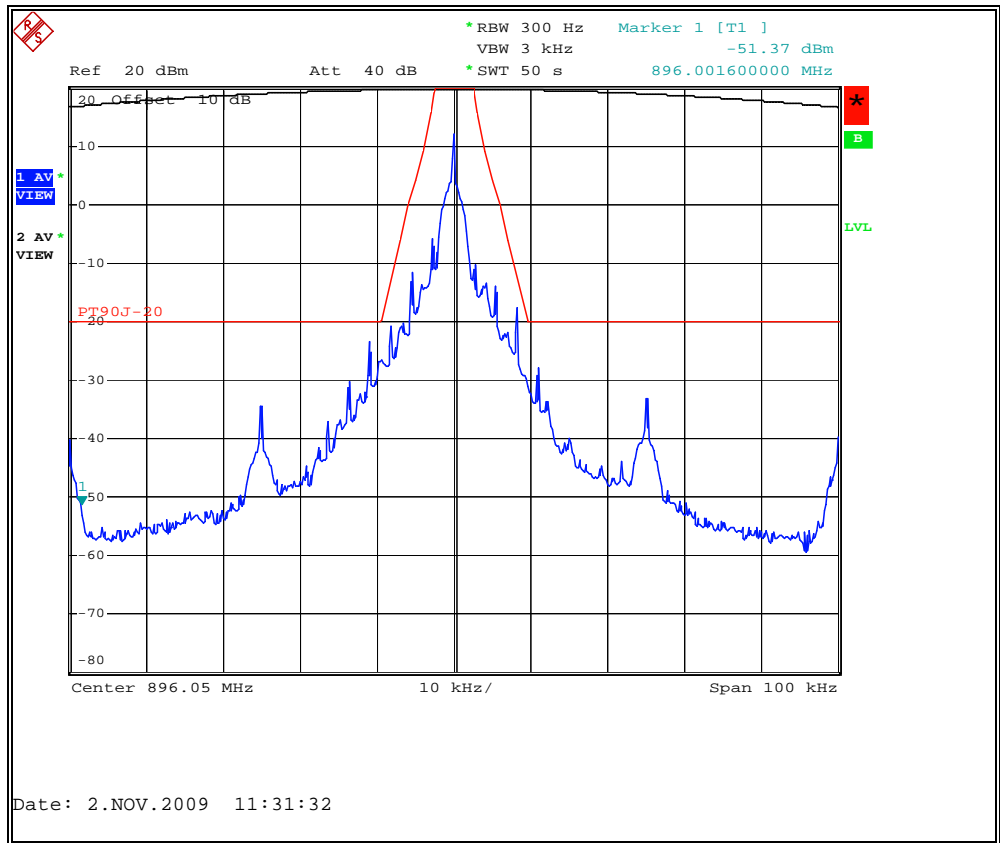
Figure 7.2.2-13: Amplitude Shift Keying Mode (ASK) – 896.05 MHz
