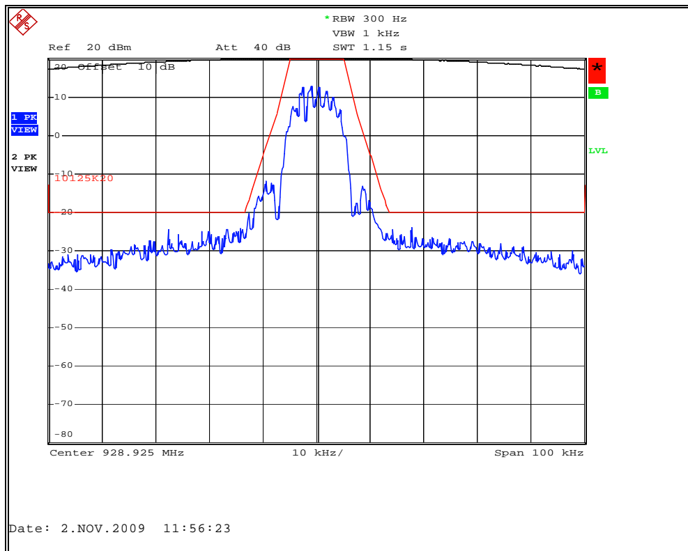
Figure 7.2.2-18: MPass Mode 10Kbps – 928.925 MHz
