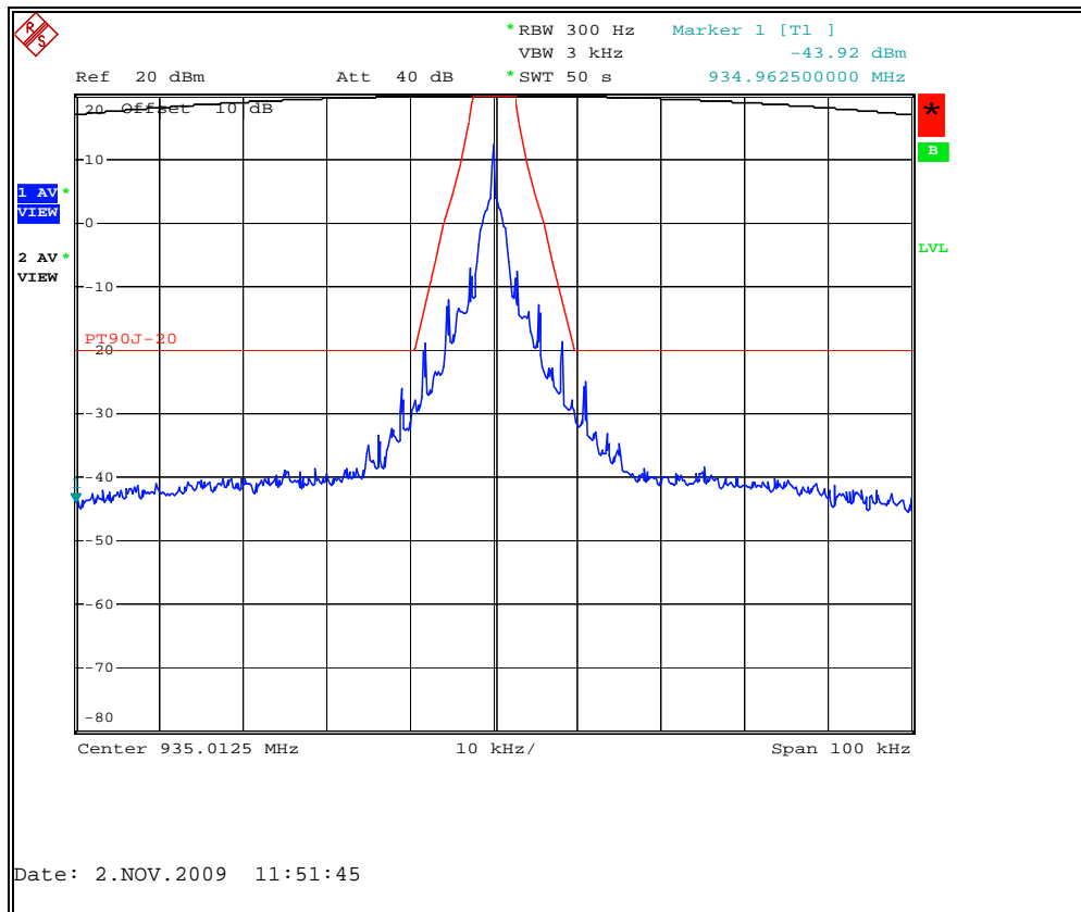
Figure 7.2.2-16: Amplitude Shift Keying Mode (ASK) – 935.0125 MHz
