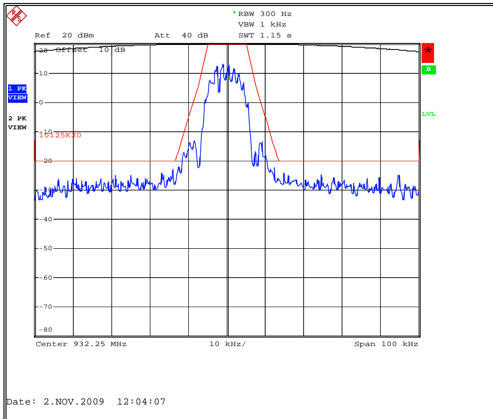
Figure 7.2.2-22: MPass Mode 10Kbps – 932.25 MHz
