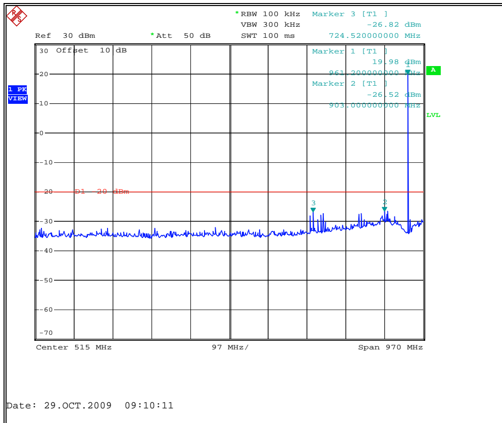
Figure 7.3.2-15: 959.91875 MHz – 30MHz to 1GHz
