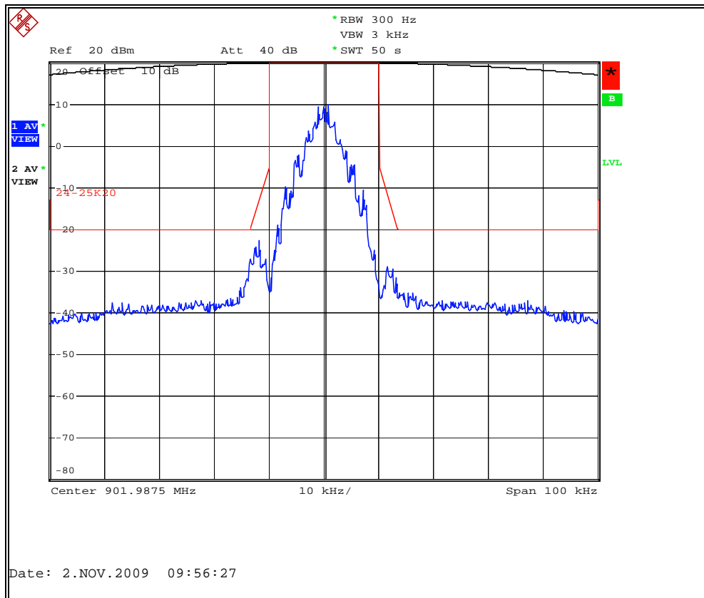
Figure 7.2.2-3: mPass Mode 12.5Kbps – 901.9875 MHz – 25 kHz Channel
