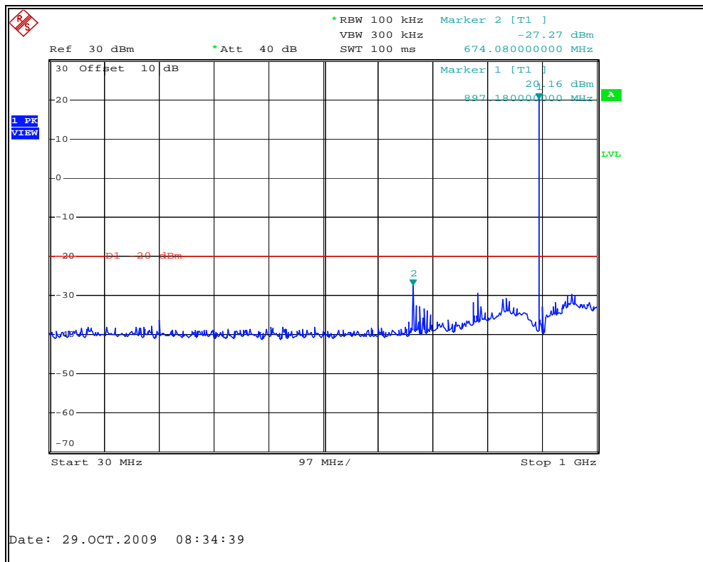
Figure 7.3.2-5: 896.05 MHz – 30MHz to 1GHz
