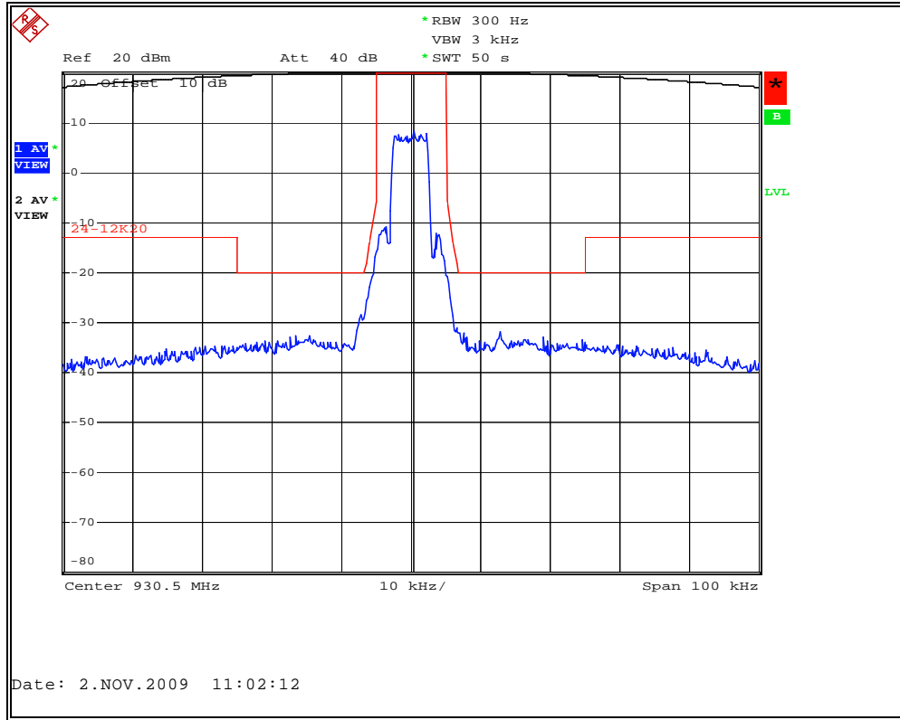
Figure 7.2.2-10: MPass Mode 5Kbps – 930.5 MHz – 12.5 kHz Channel
