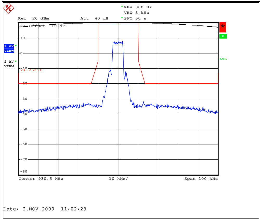
Figure 7.2.2-6: MPass Mode 5Kbps – 930.5 MHz – 25 kHz Channel
