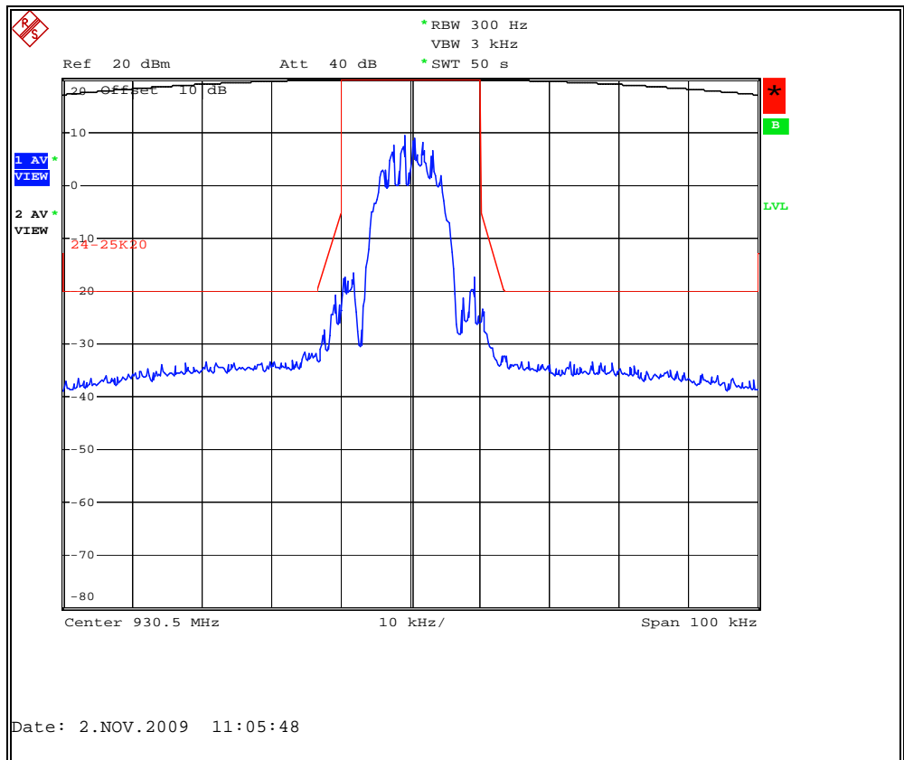
Figure 7.2.2-7: MPass Mode 10Kbps – 930.5 MHz – 25 kHz Channel
