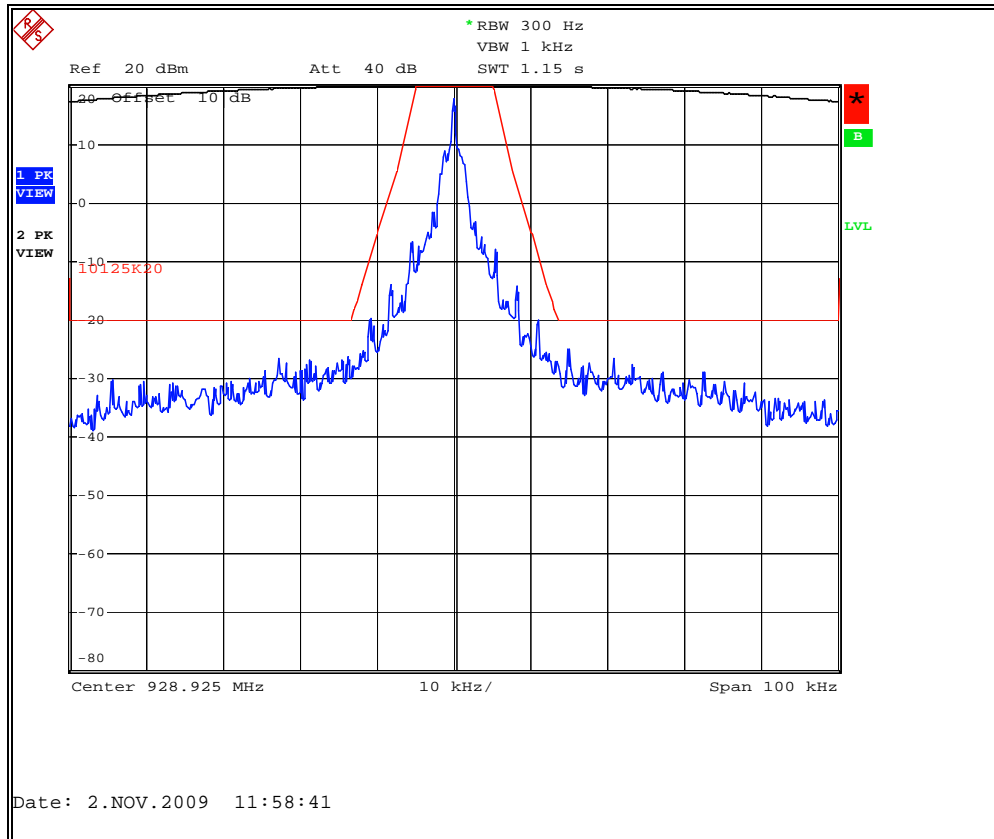
Figure 7.2.2-20: Amplitude Shift Keying Mode (ASK) – 928.925 MHz
