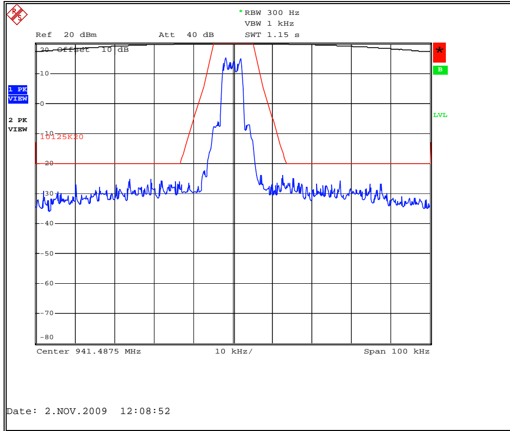
Figure 7.2.2-25: MPass Mode 5Kbps – 941.4875 MHz
