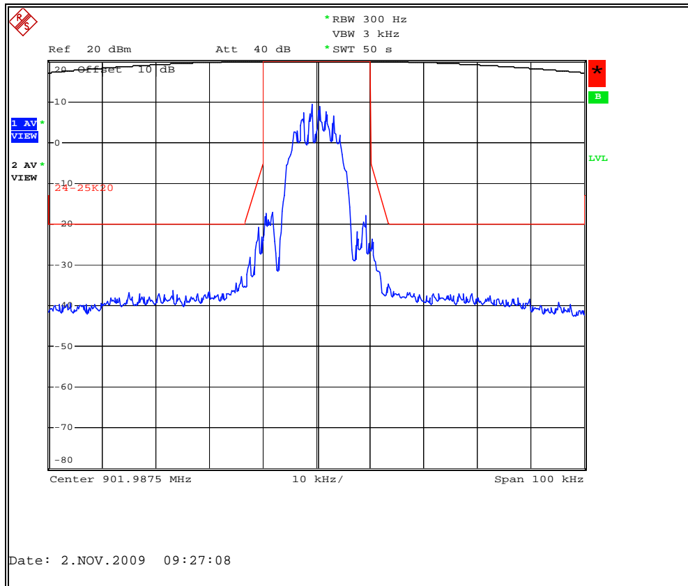
Figure 7.2.2-2: mPass Mode 10Kbps – 901.9875 MHz – 25 kHz Channel
