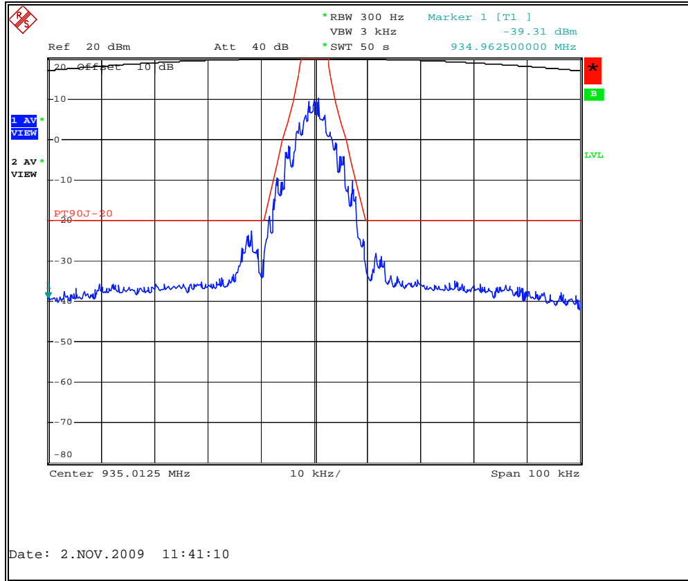
Figure 7.2.2-15: MPass Mode 12.5Kbps – 935.0125 MHz
