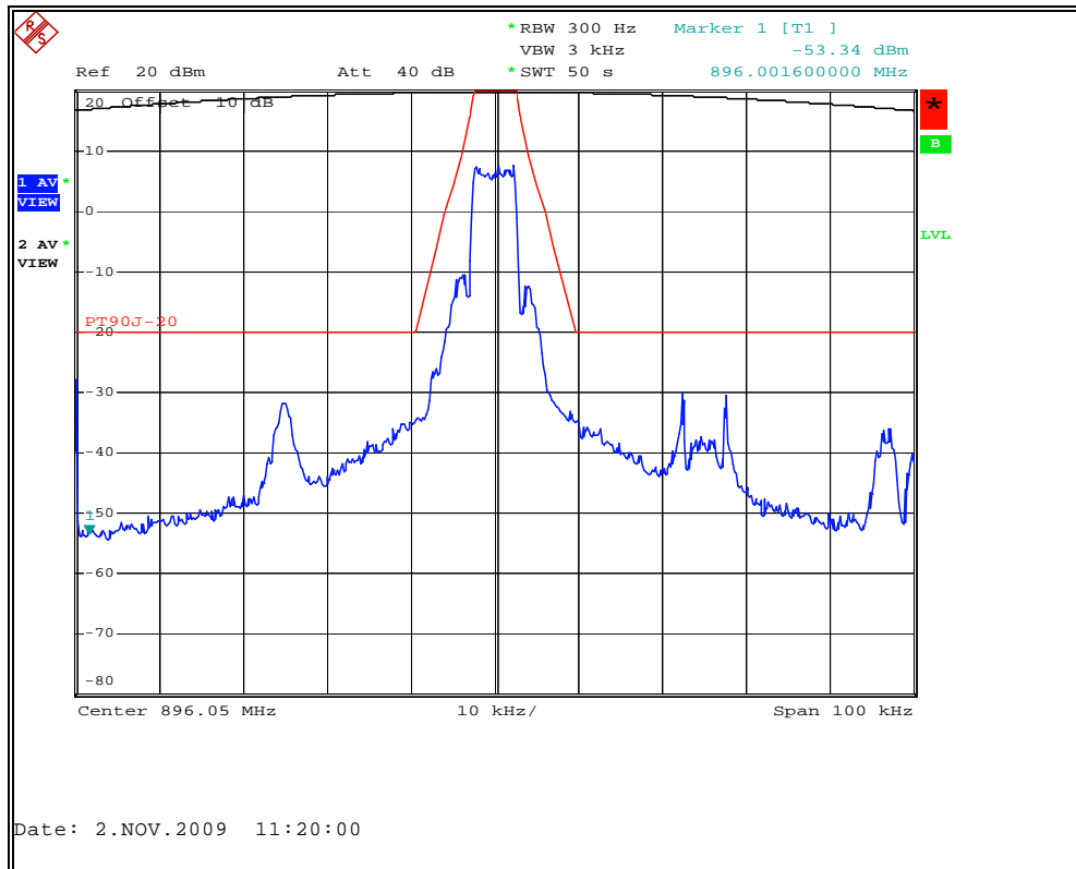
Figure 7.2.2-11: MPass Mode 5Kbps – 896.05 MHz
