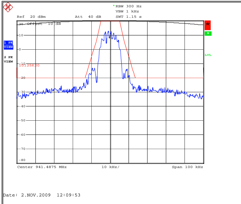
Figure 7.2.2-26: MPass Mode 10Kbps – 941.4875 MHz
