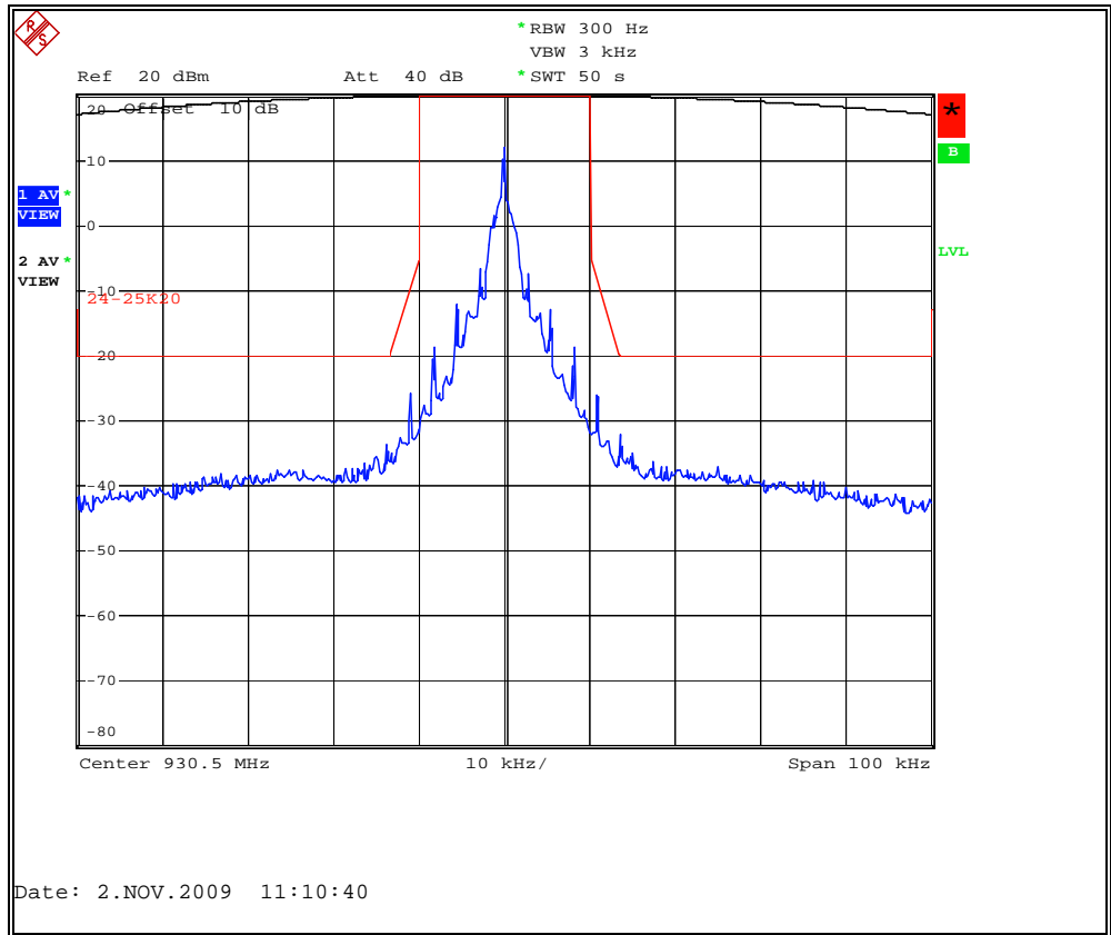
Figure 7.2.2-9: Amplitude Shift Keying Mode (ASK) – 930.5 MHz – 25 kHz Channel
