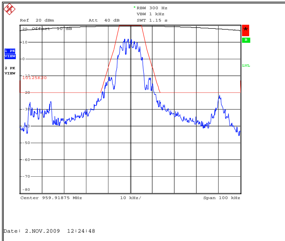
Figure 7.2.2-30: MPass Mode 10Kbps – 959.91875 MHz
