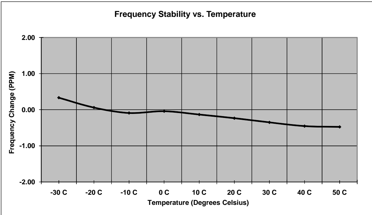
Figure 7.5.2-3: Frequency Stability – 959.91875MHz
