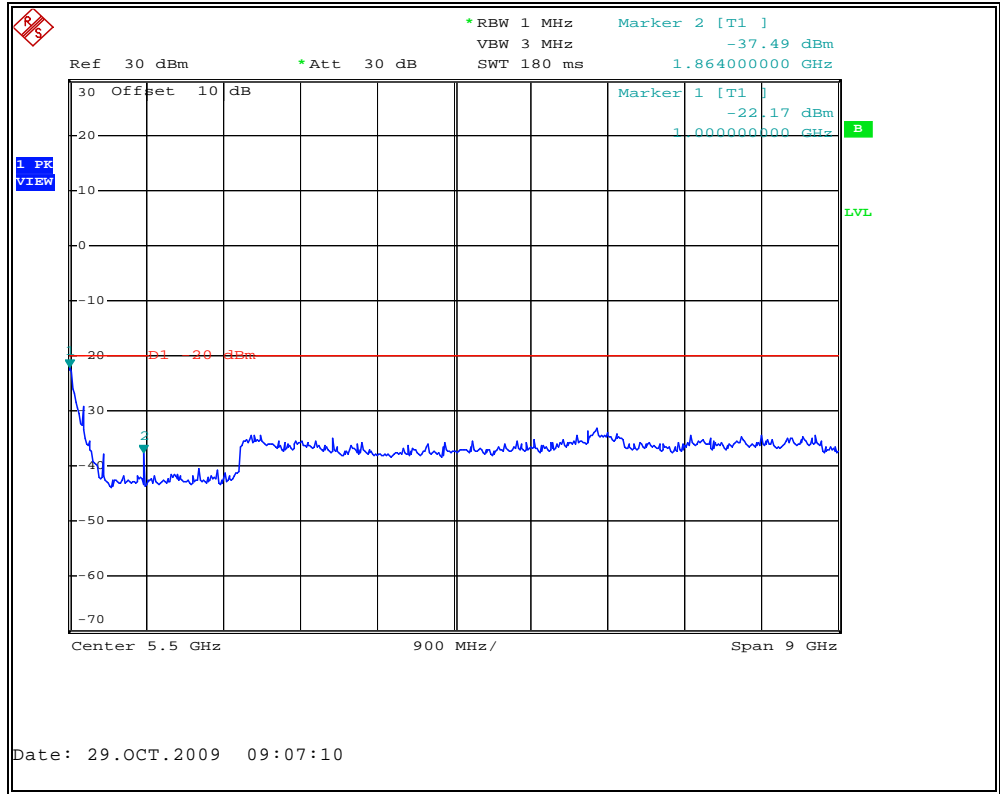
Figure 7.3.2-8: 935.0125 MHz – 1GHz to 10GHz
