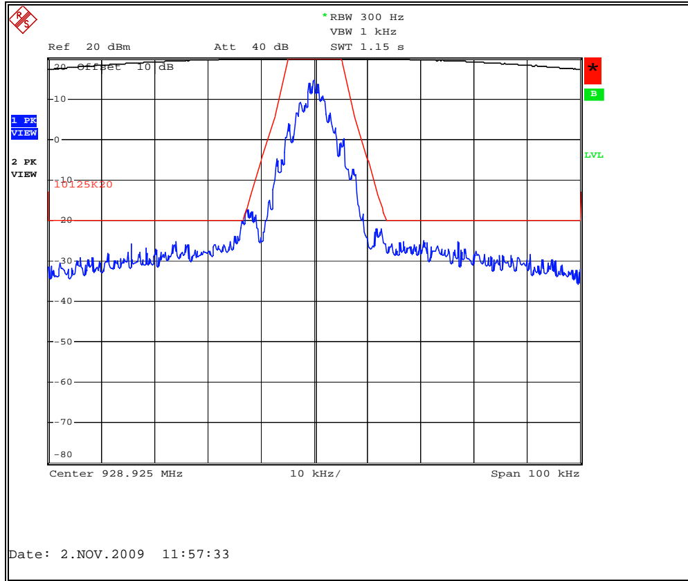
Figure 7.2.2-19: MPass Mode 12.5Kbps – 928.925 MHz
