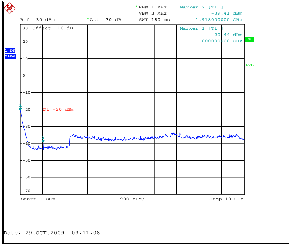
Figure 7.3.2-16: 959.91875 MHz – 1GHz to 10GHz
