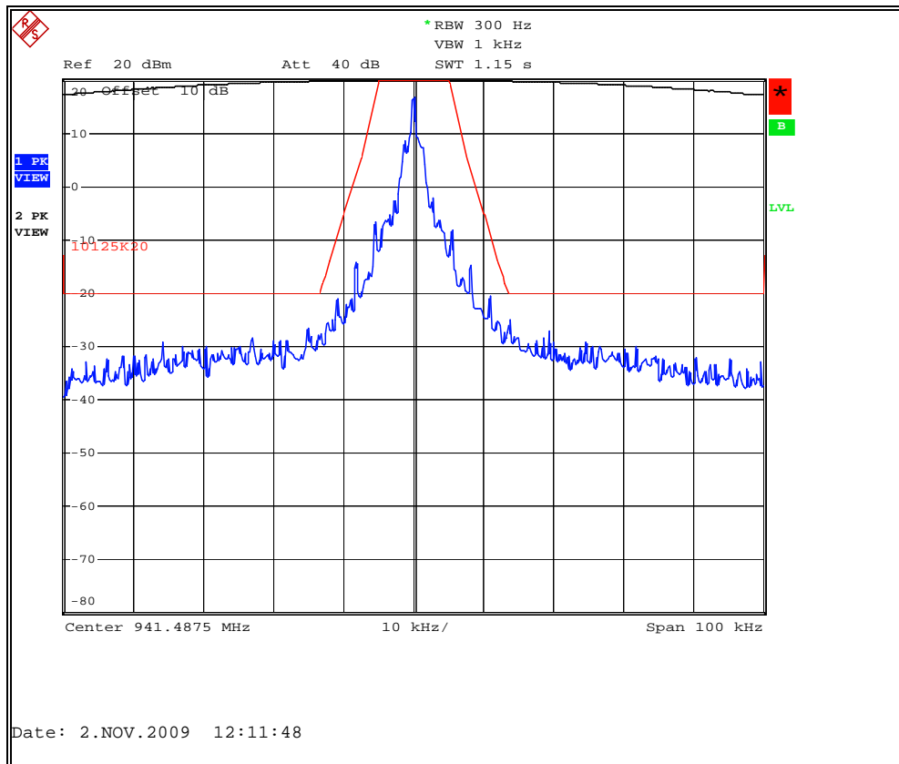
Figure 7.2.2-28: Amplitude Shift Keying Mode (ASK)– 941.4875 MHz
