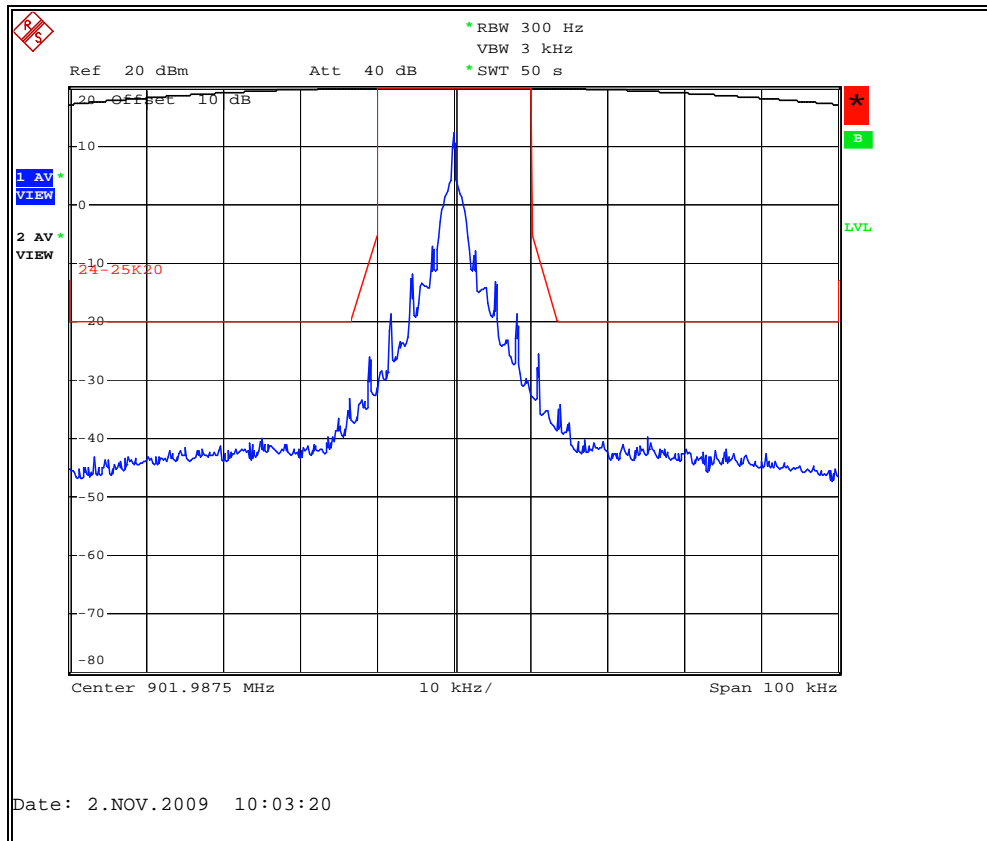
Figure 7.2.2-4: Amplitude Shift Keying Mode (ASK) – 901.9875 MHz – 25 kHz Channel
