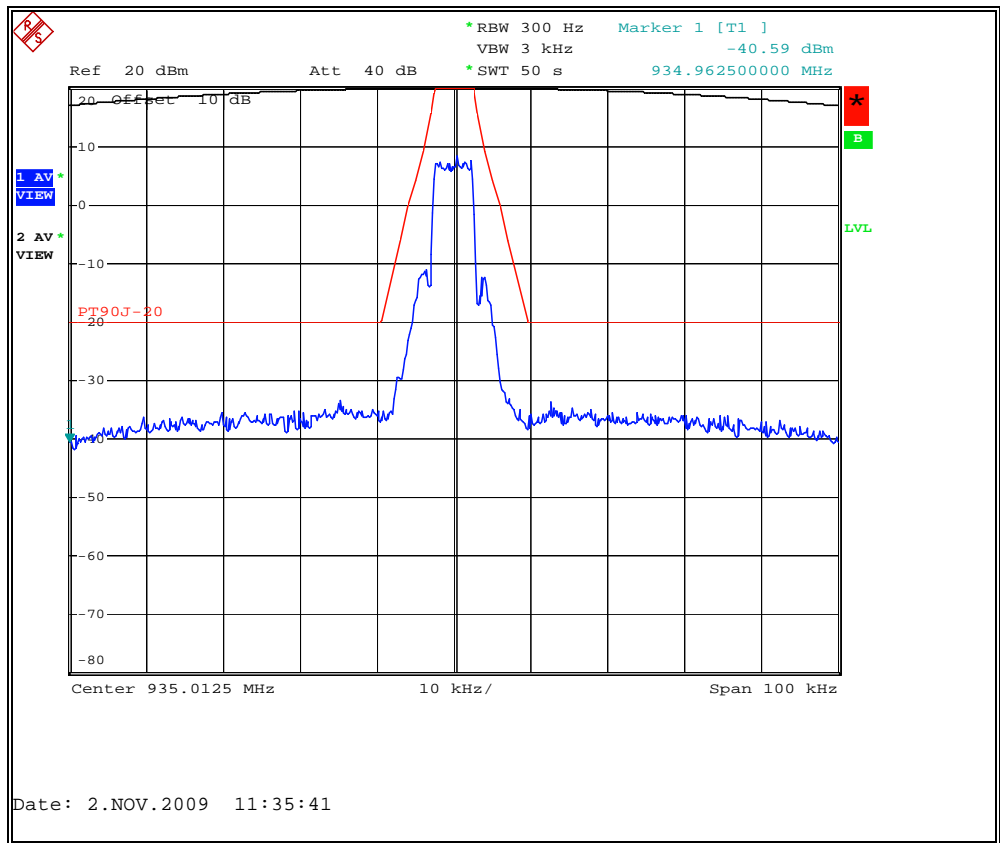
Figure 7.2.2-14: MPass Mode 5Kbps – 935.0125 MHz
