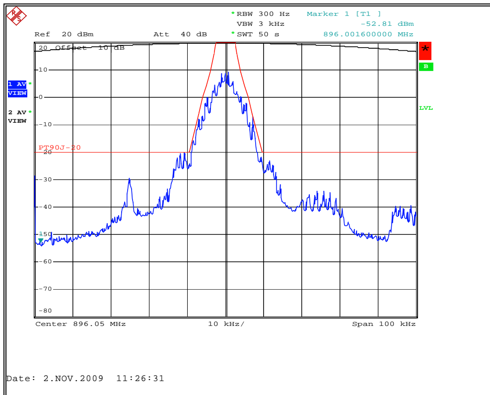
Figure 7.2.2-12: MPass Mode 12.5Kbps – 896.05 MHz
