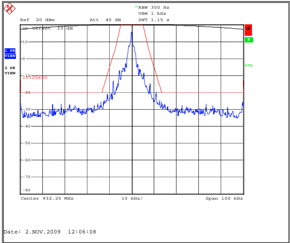
Figure 7.2.2-24: Amplitude Shift Keying Mode (ASK) – 932.25 MHz
