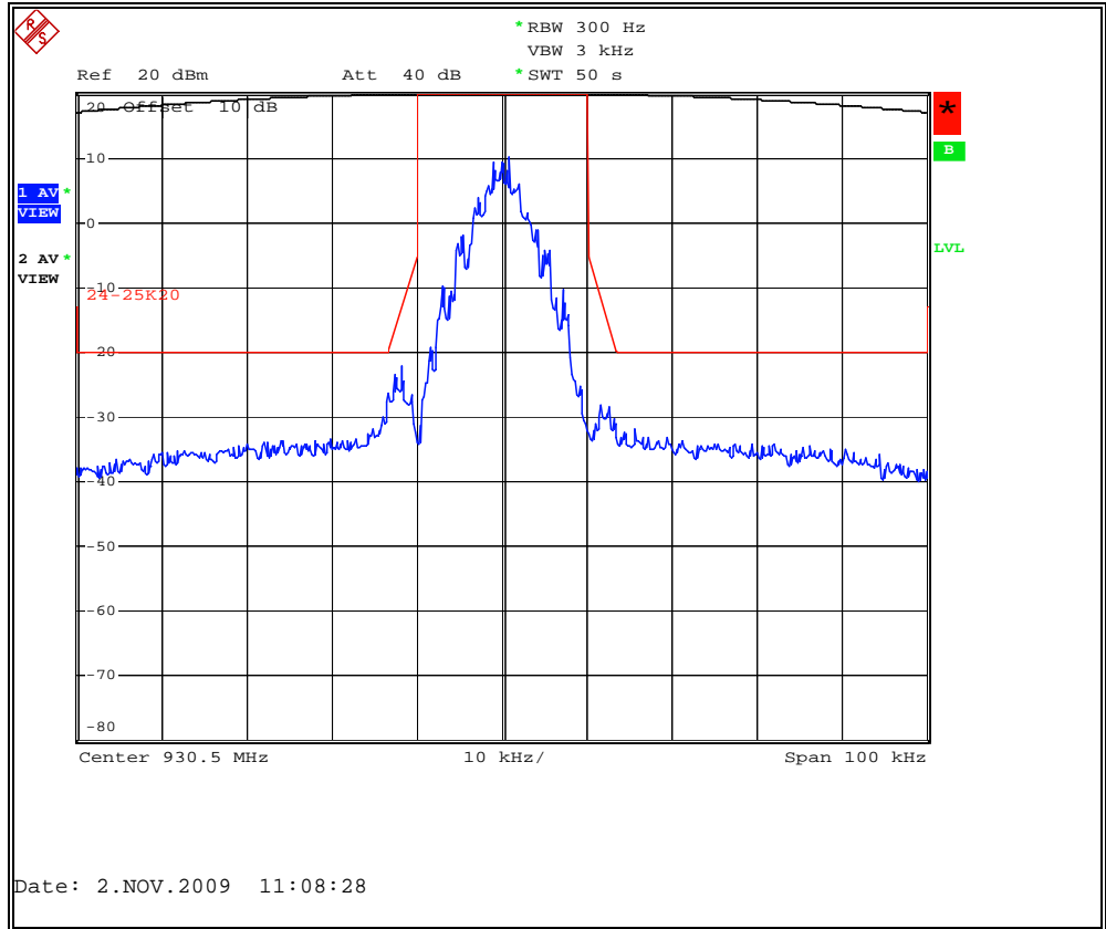
Figure 7.2.2-8: MPass Mode 12.5Kbps – 930.5 MHz – 25 kHz Channel
