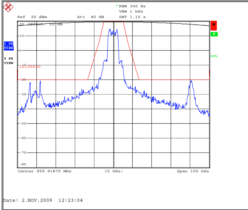
Figure 7.2.2-29: MPass Mode 5Kbps – 959.91875 MHz
