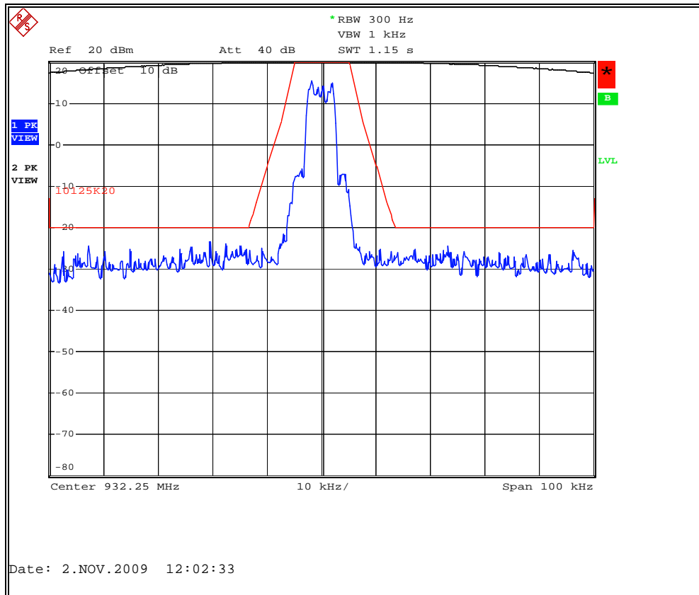
Figure 7.2.2-21: MPass Mode 5Kbps – 932.25 MHz
