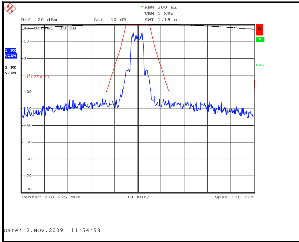
Figure 7.2.2-17: MPass Mode 5Kbps – 928.925 MHz
