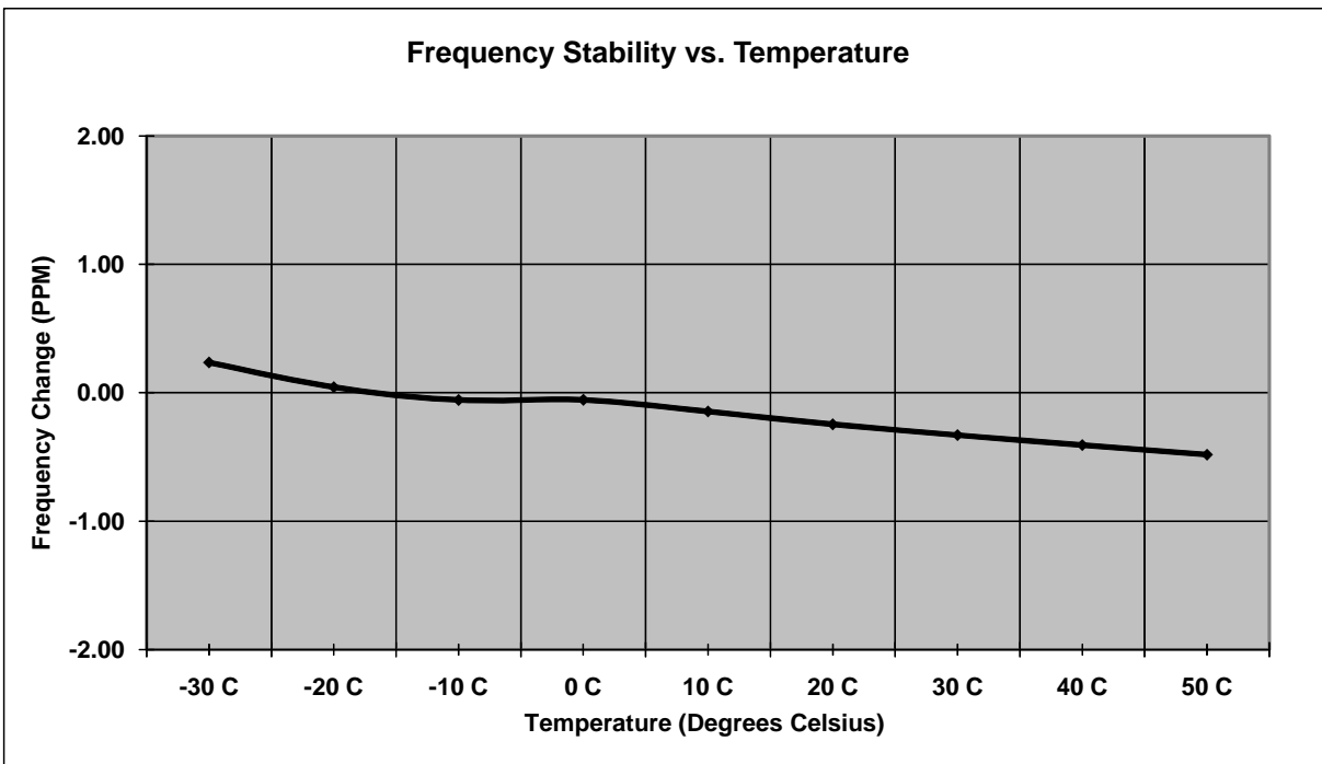
Figure 7.5.2-2: Frequency Stability – 896.05MHz
