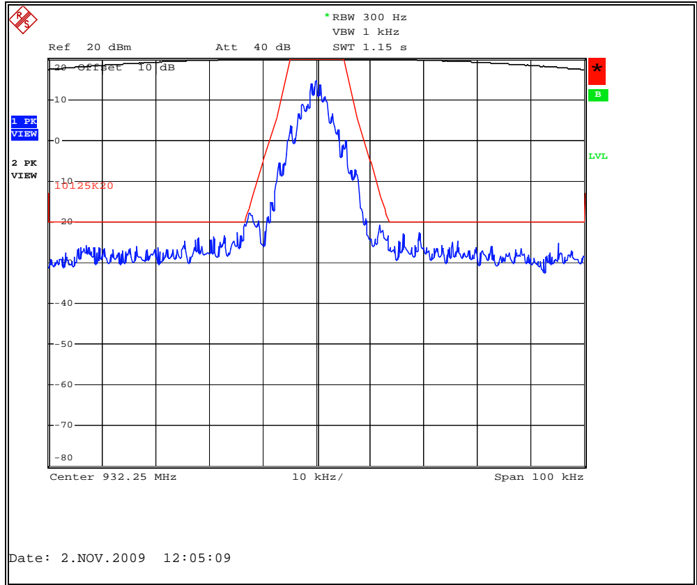
Figure 7.2.2-23: MPass Mode 12.5Kbps – 932.25 MHz
