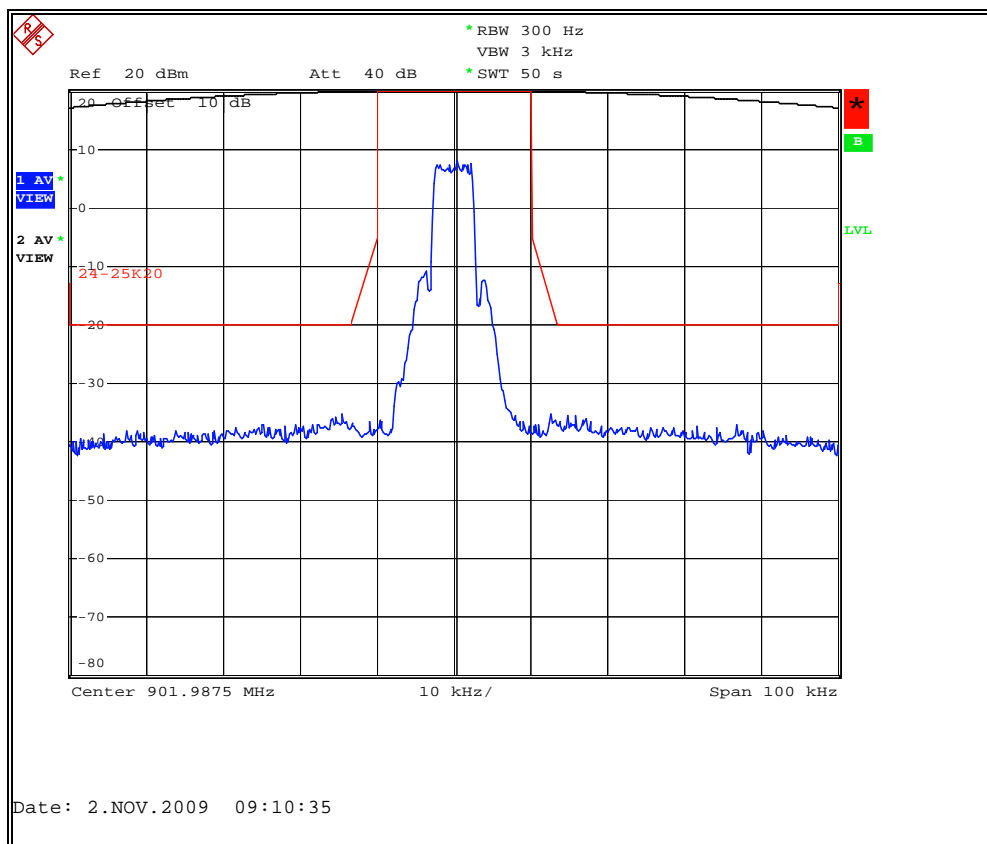
Figure 7.2.2-1: mPass Mode 5Kbps – 901.9875 MHz – 25 kHz Channel
