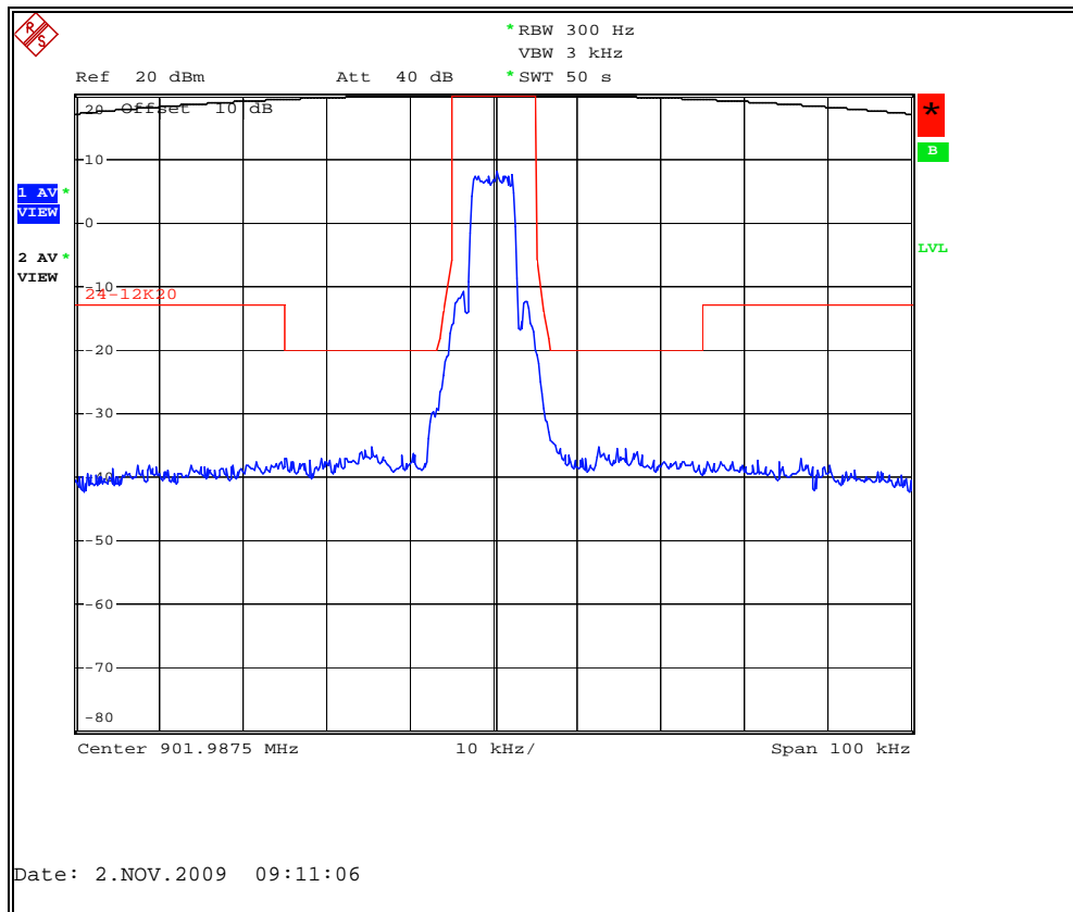
Figure 7.2.2-5: mPass Mode 5Kbps – 901.9875 MHz – 12.5 kHz Channel
