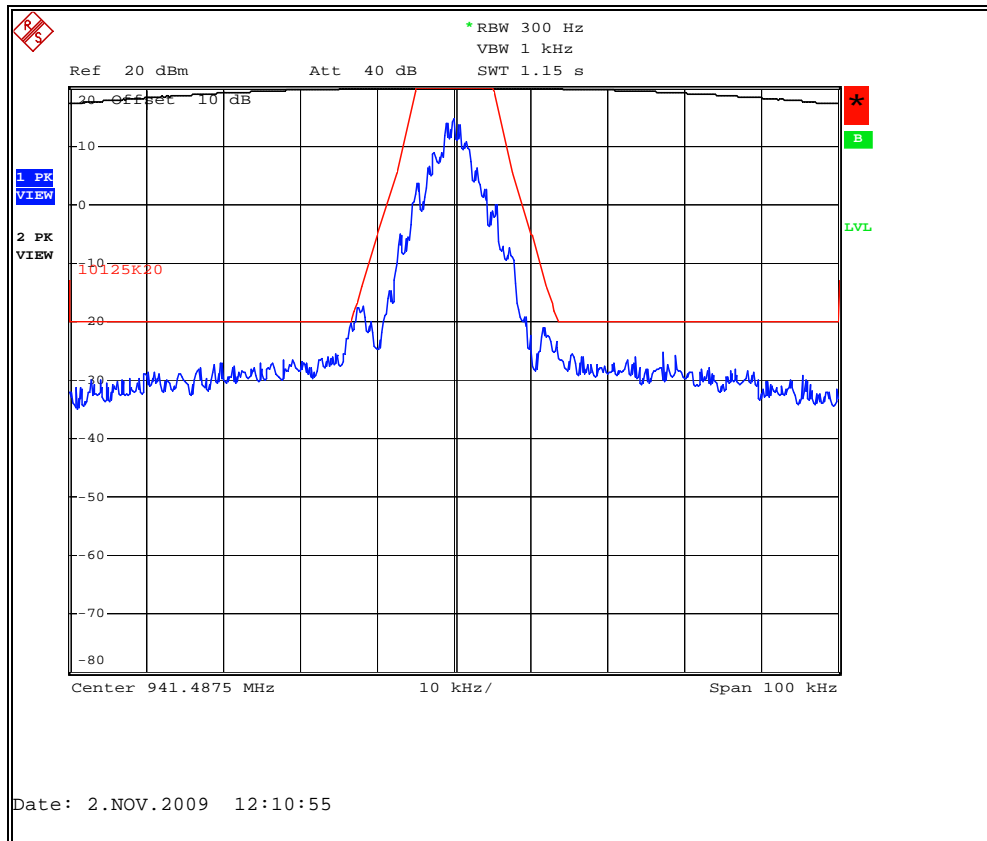
Figure 7.2.2-27: MPass Mode 12.5Kbps – 941.4875 MHz
