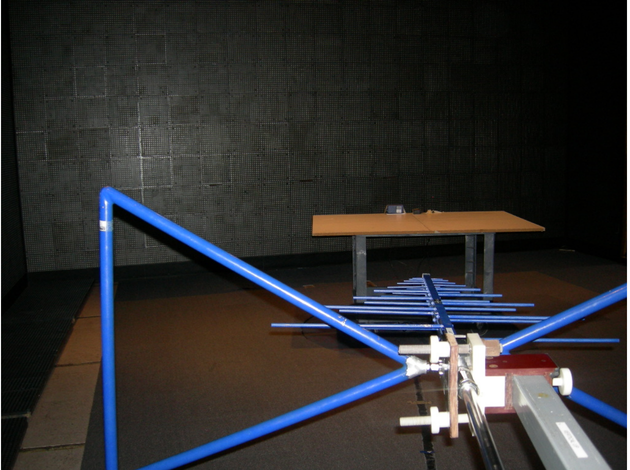
Figure 5: Unintentional Radiated Emissions
