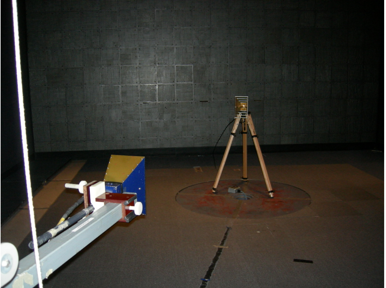
Figure 3: Intentional Radiated Emissions (Substitution)
