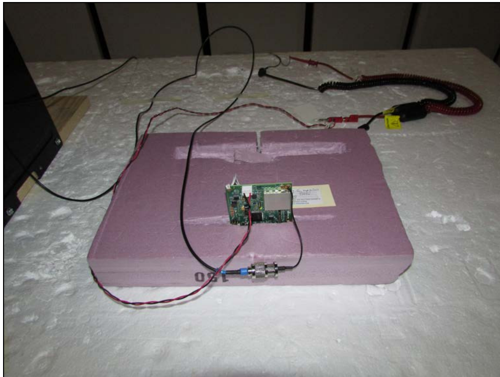
Figure 3: Test Setup
