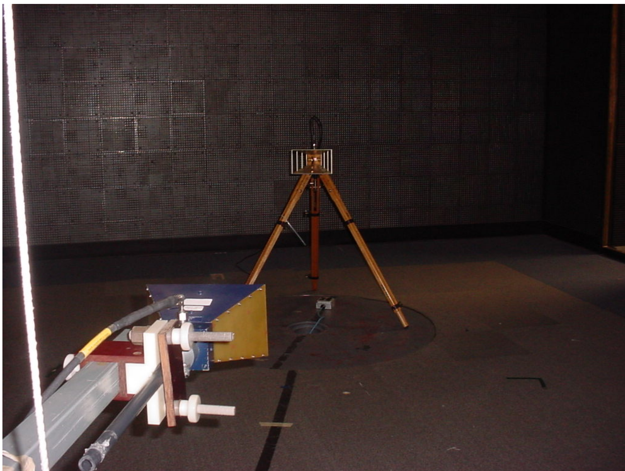
Figure 4: Radiated – Intentional – Substitution
