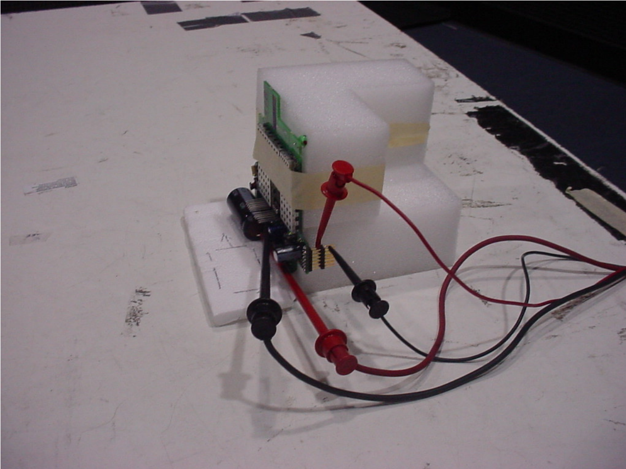
Figure 3: Radiated – Intentional – Close Up View
