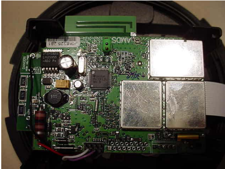
Figure 3. RF Board Front
