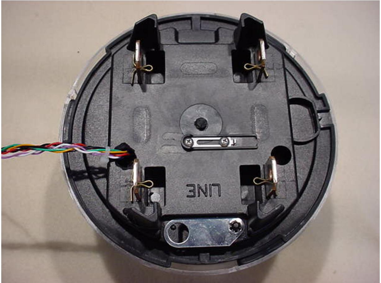
Figure 2. External - Rear
