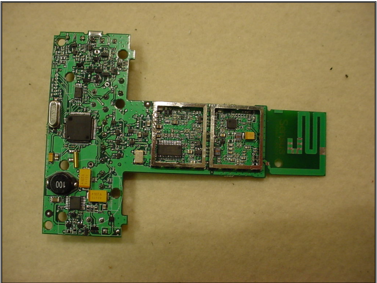
Figure 1: RF Board
