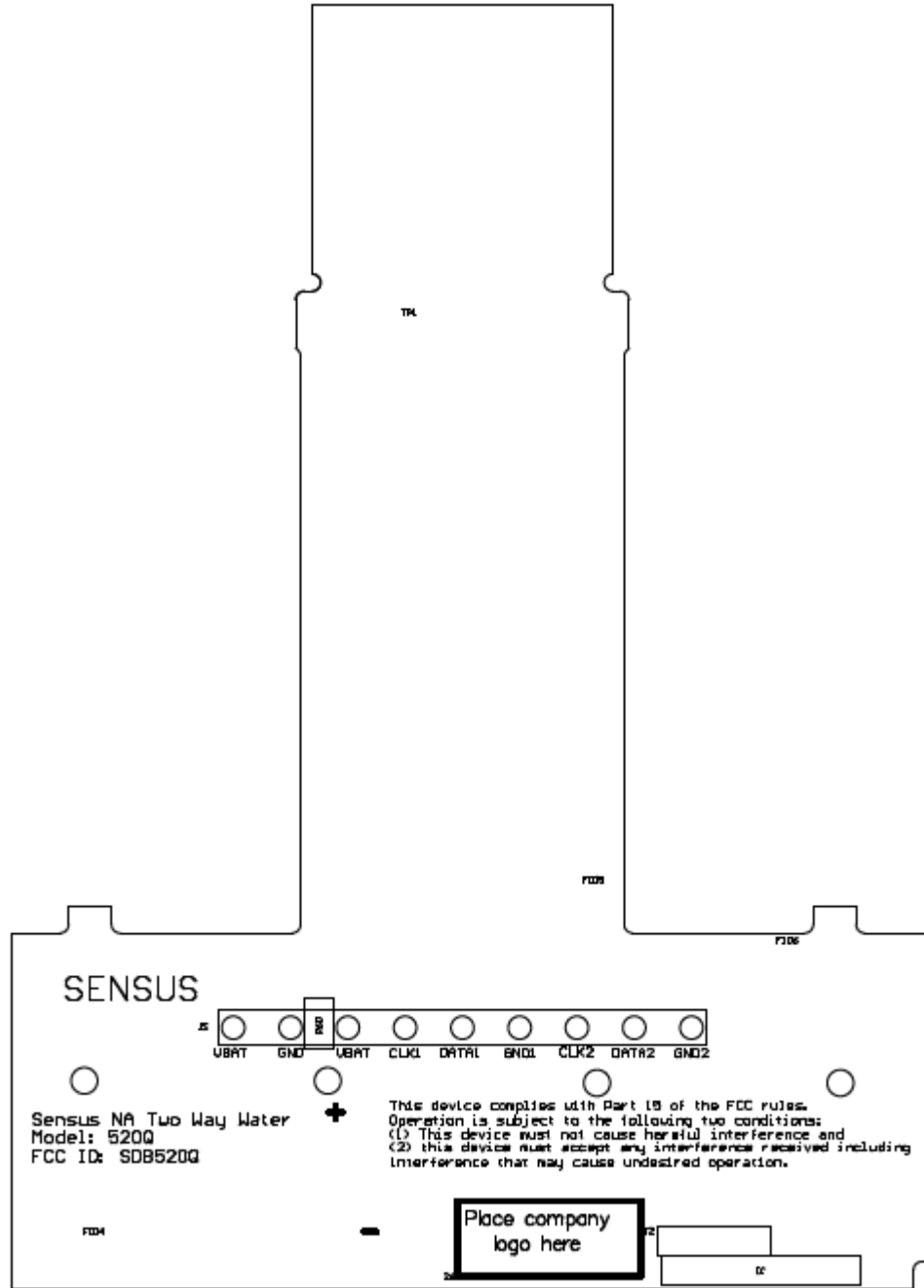
Figure 2: 520Q Module – Label and Location (Bottom View)
