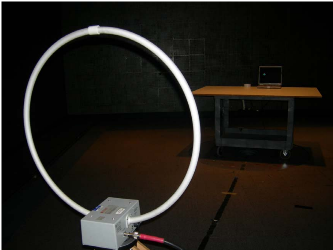
Figure 2: USB - Radiated Emissions
