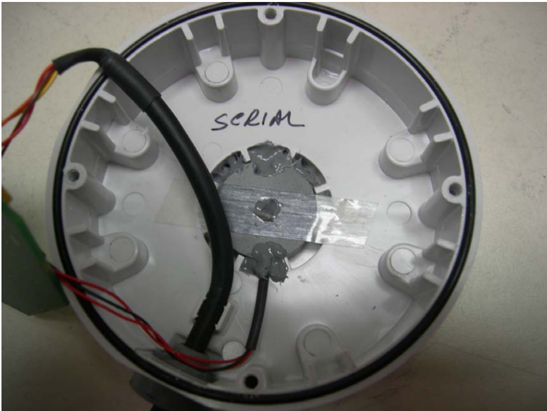
Figure 6: RS232 Serial Magnetic Coupling Coil
