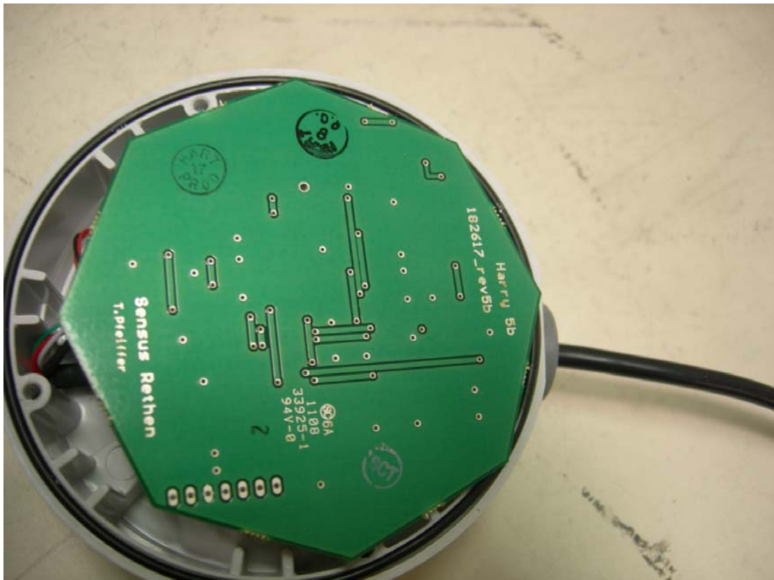
Figure 2: USB PCB – Back
