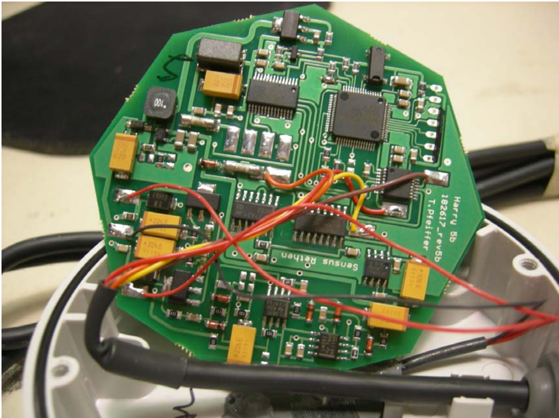
Figure 3: RS-232 Serial PCB – Front
