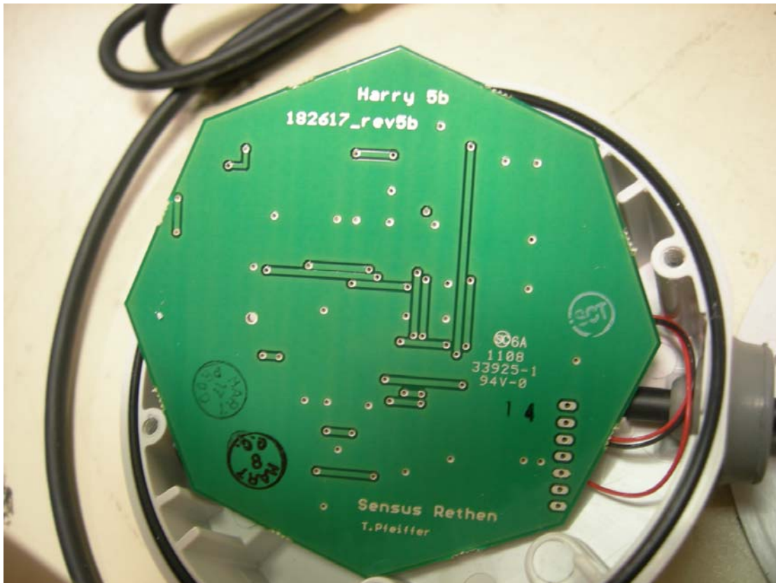
Figure 4: RS-232 Serial USB PCB – Back
