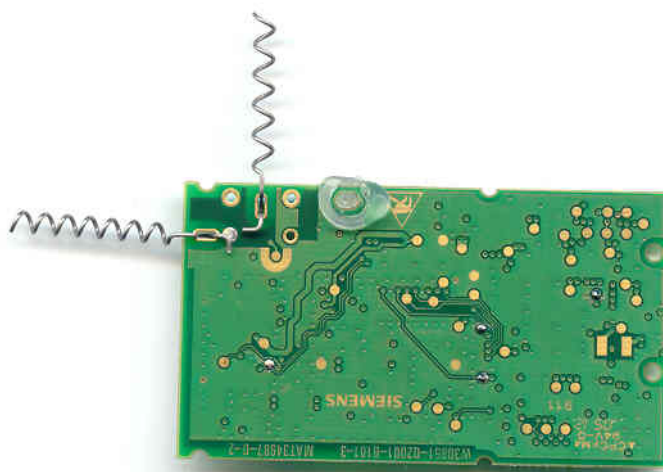
Bottom of RF PCB
