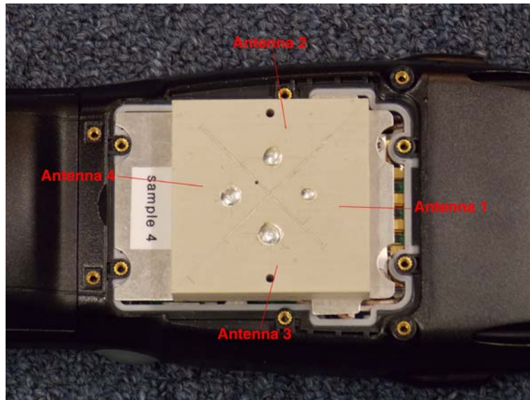
Antenna Location
