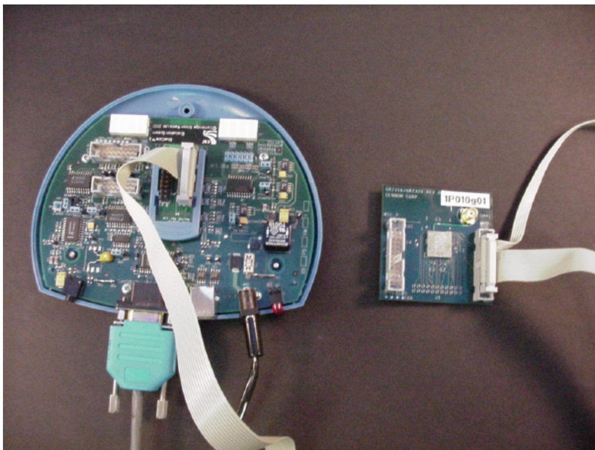
Photo 3: Test setup for conducted measurements (setup_b01, EUT B + AE 2)
