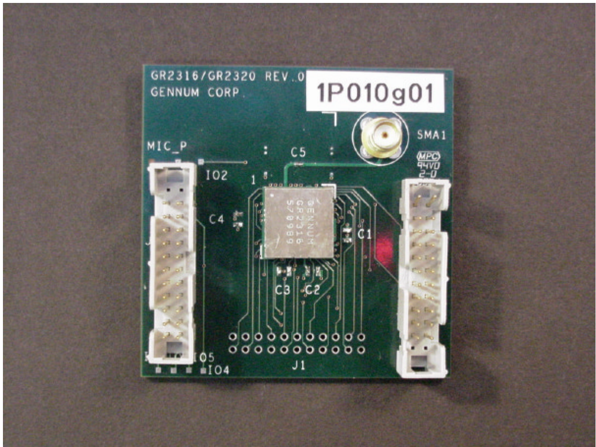
Photo 4: EUT (front side)
