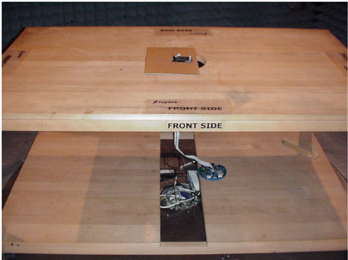
Photo 2: Test setup for radiated measurements (semi anechoic chamber, tests < 1 GHz)
