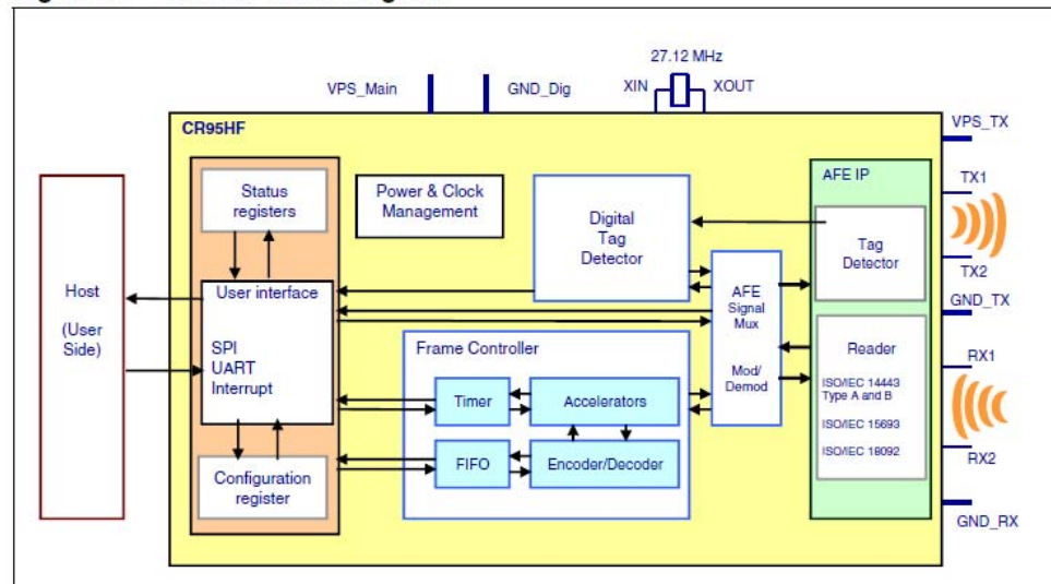
Figure 2. CR95HF block diagram
