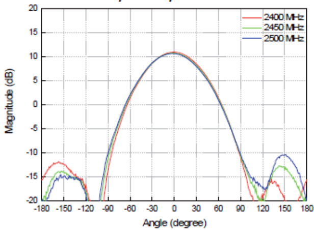
H-plane Co-polar. Pattern
