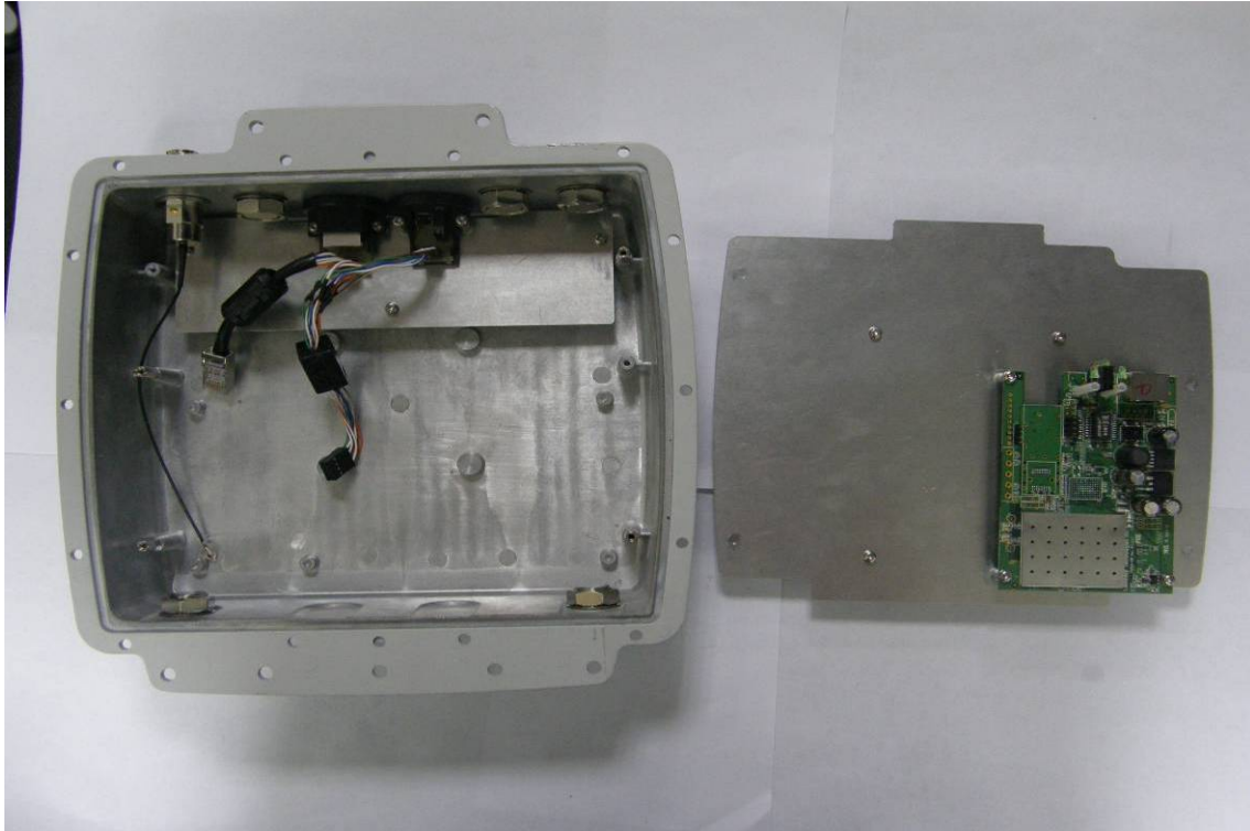
Open View of EUT – 1 (Patch 1 Internal Antenna)
