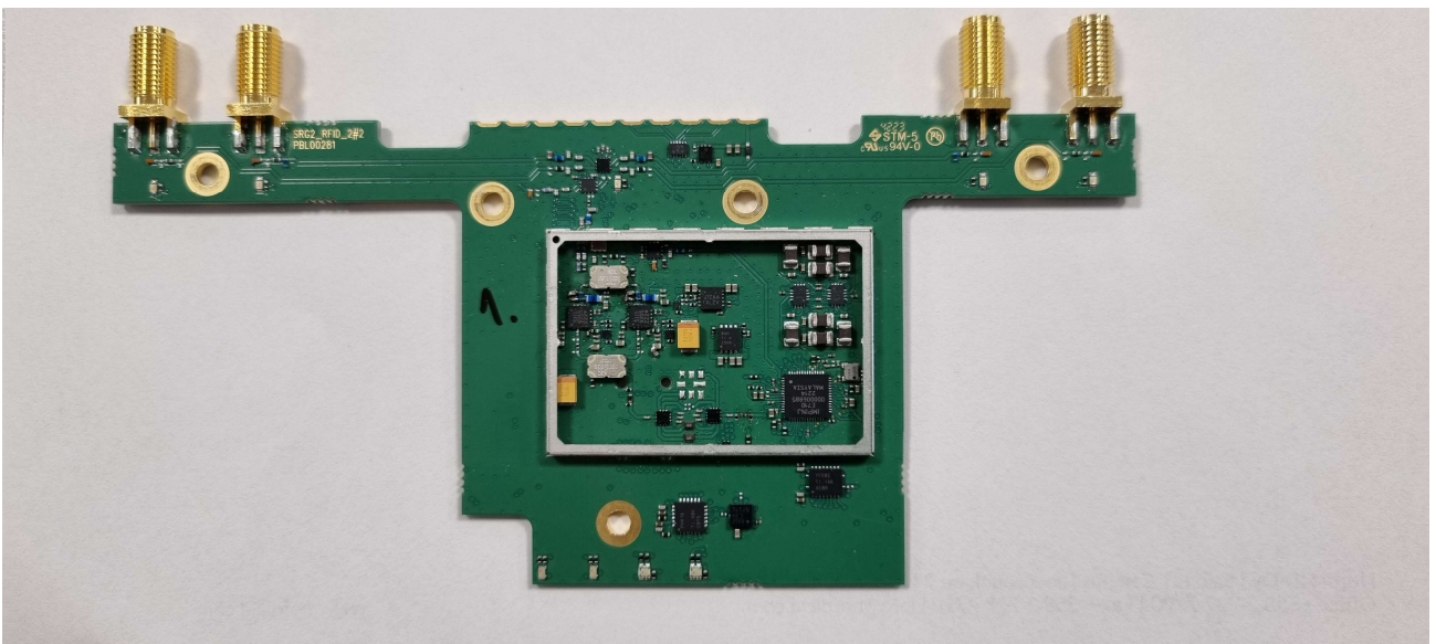
Picture 2. NUR3-1W6 top side without shield
