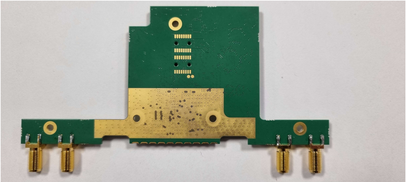
Picture 1. NUR3-1W6 bottom view
