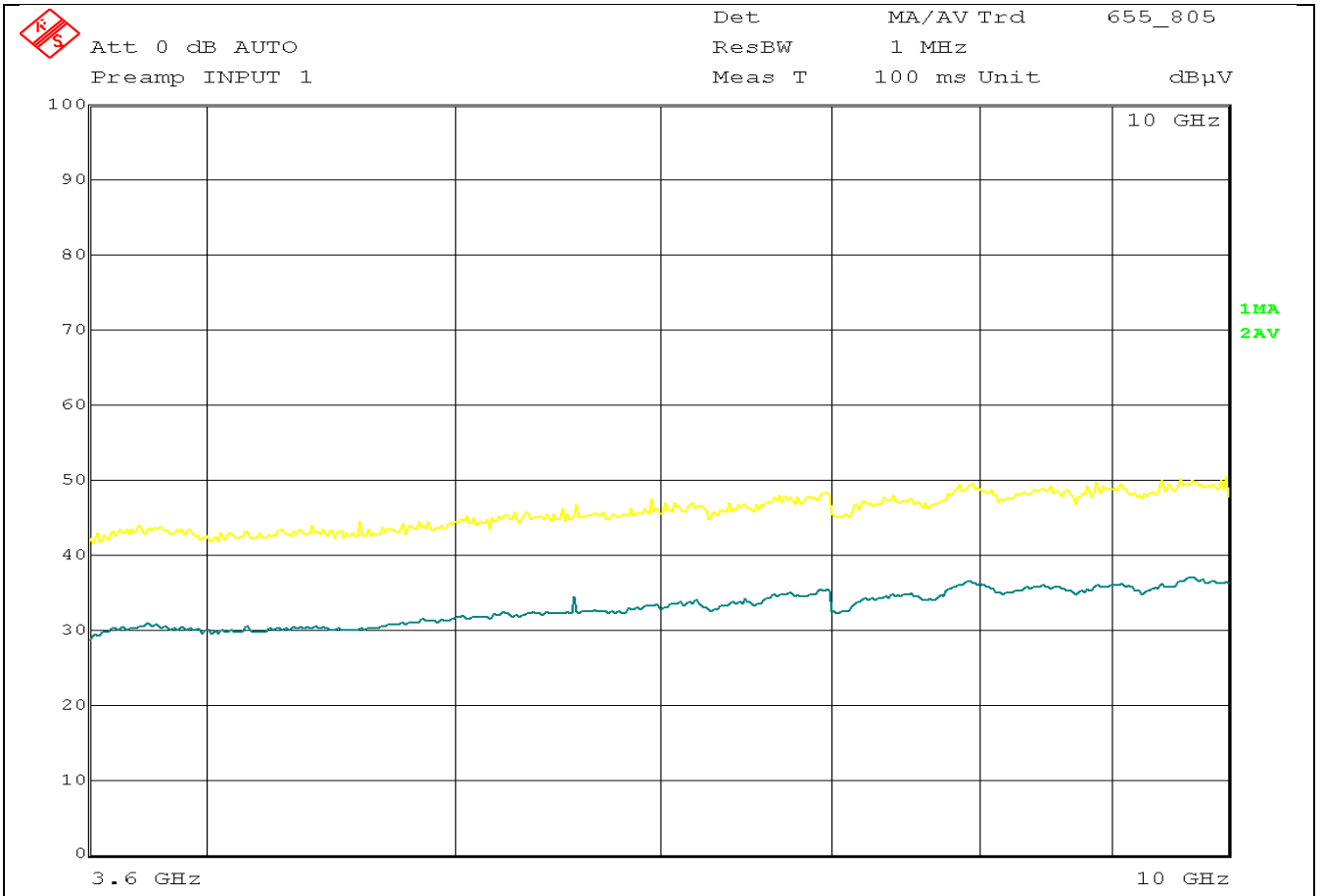
Fig E7: High Channel Radiated Emissions 3.6GHz - 10GHz, Vertical, 3metre
