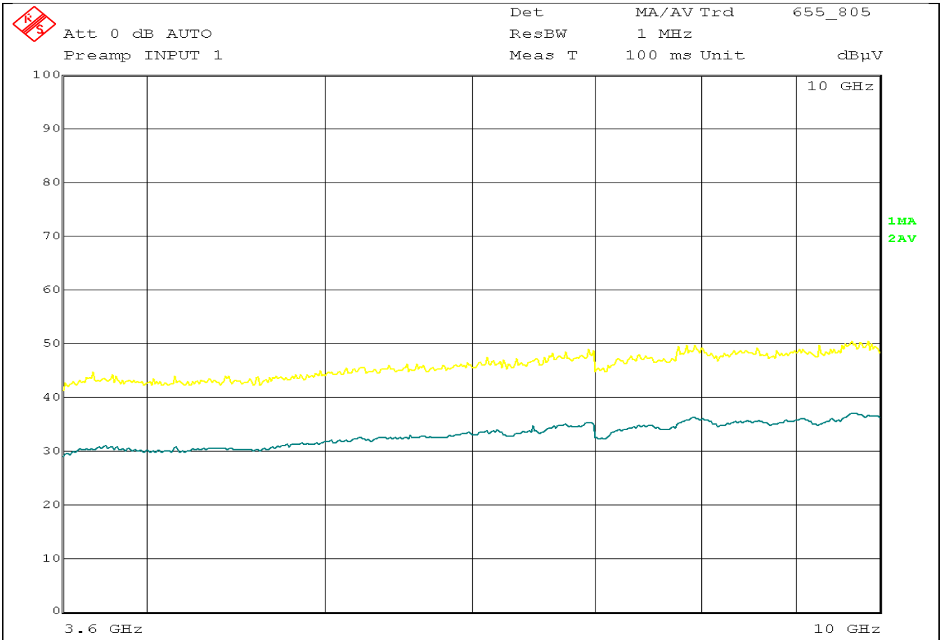
Fig D7: High Channel Radiated Emissions 3.6GHz - 10GHz, Vertical, 3metre
