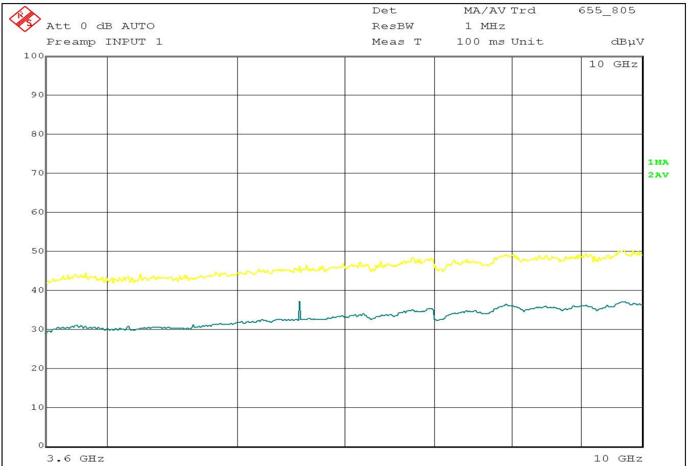
Fig D8: High Channel Radiated Emissions 3.6GHz - 10GHz, Horizontal, 3metre
