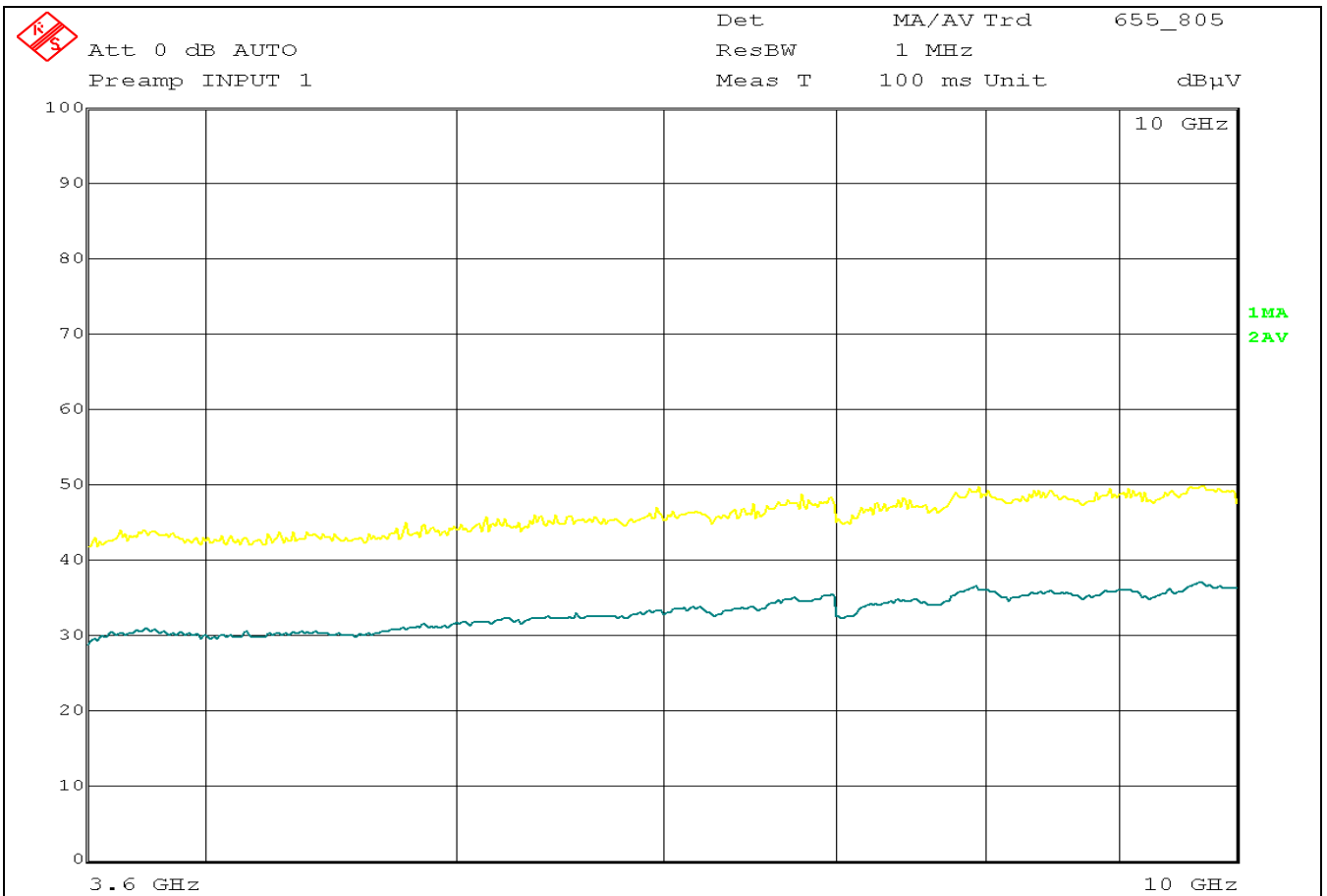
Fig E8: High Channel Radiated Emissions 3.6GHz - 10GHz, Horizontal, 3metre
