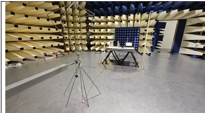
Fig A1: Radiated Emissions Below 1GHz
