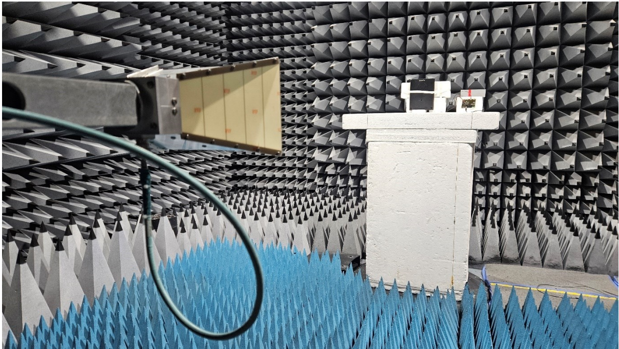
Radiated Emissions 1GHz to 10GHz S0 Antenna
