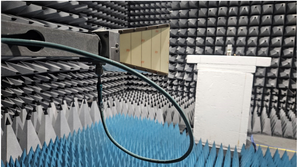
EUT Close up SA0408 Antenna Radiated Emissions
