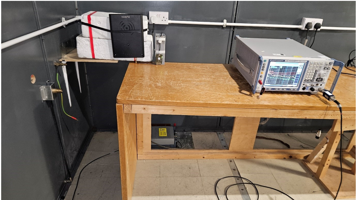
Conducted Emissions on the mains
