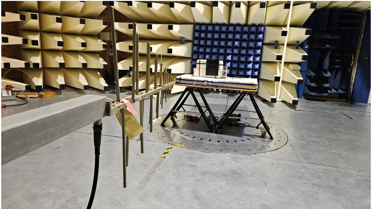
Radiated Emissions 300MHz-1GHz S0 Antenna
