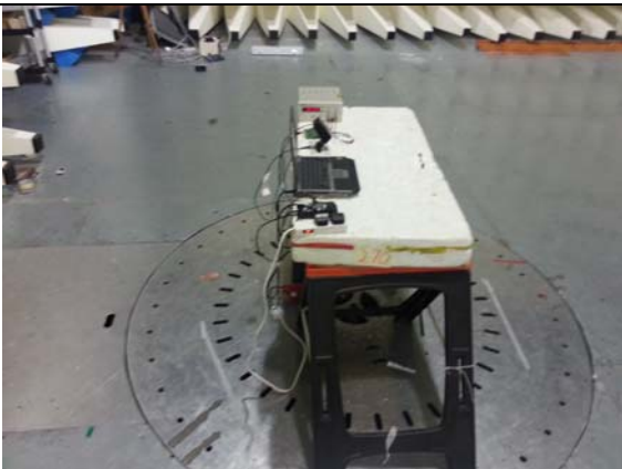
Fig 4 Radiated Emissions
