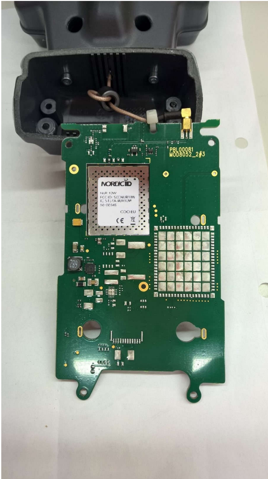
Picture 15. NUR-10W RFID module in Merlin CD ONE 805-2F Mod board (top view).
