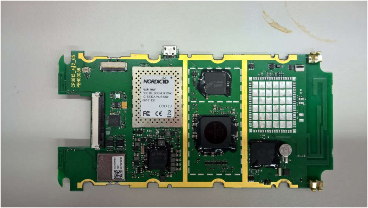
Picture 1: CPU815 board top side where NUR-10W and SDC-SSD40NBT modules are located.
