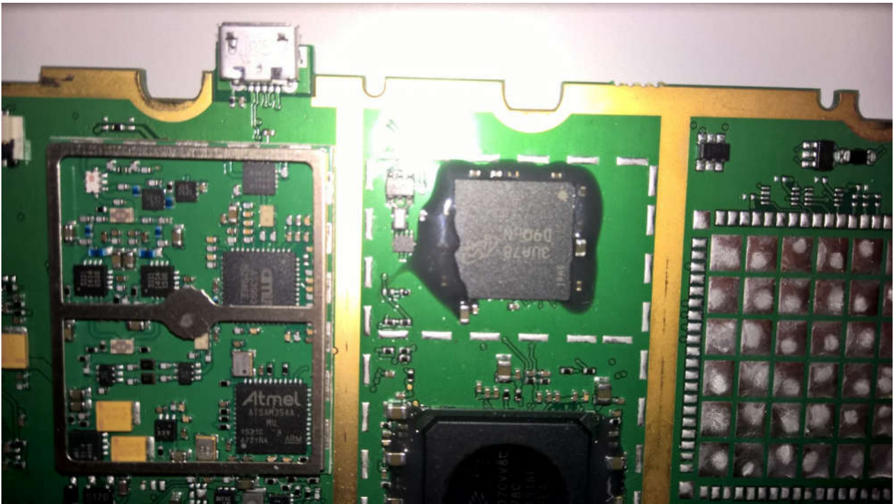
Picture 3: NUR-10W without RF shield
