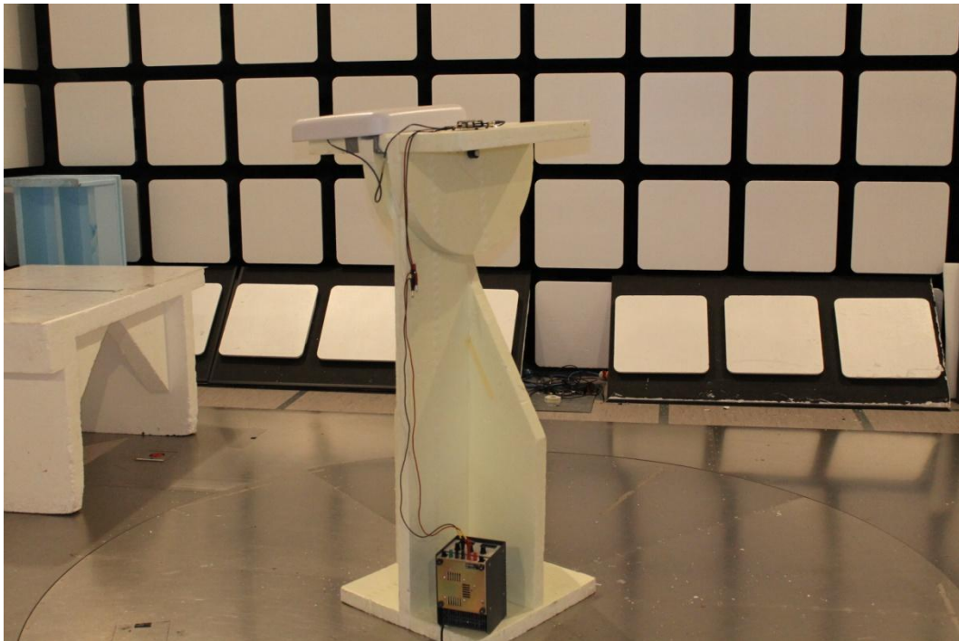
Photograph 1. Radiated emissions 1000 - 10000 MHz ant2.
