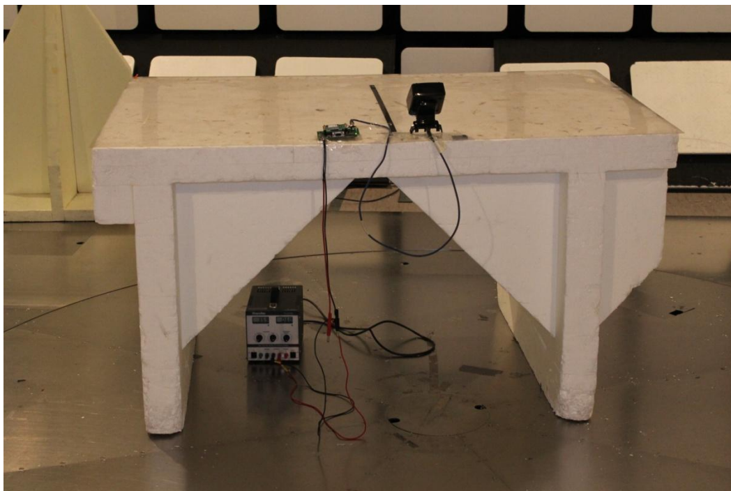
Photograph 1. Radiated emissions 30 - 1000 MHz ant1.
