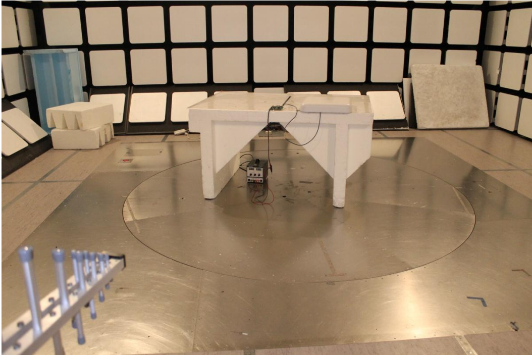
Photograph 1. Radiated emissions 30 - 1000 MHz ant2.
