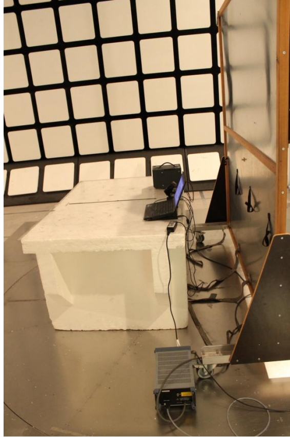
Photograph 2. Conducted emissions at mains ports 0.150 – 30 MHz
