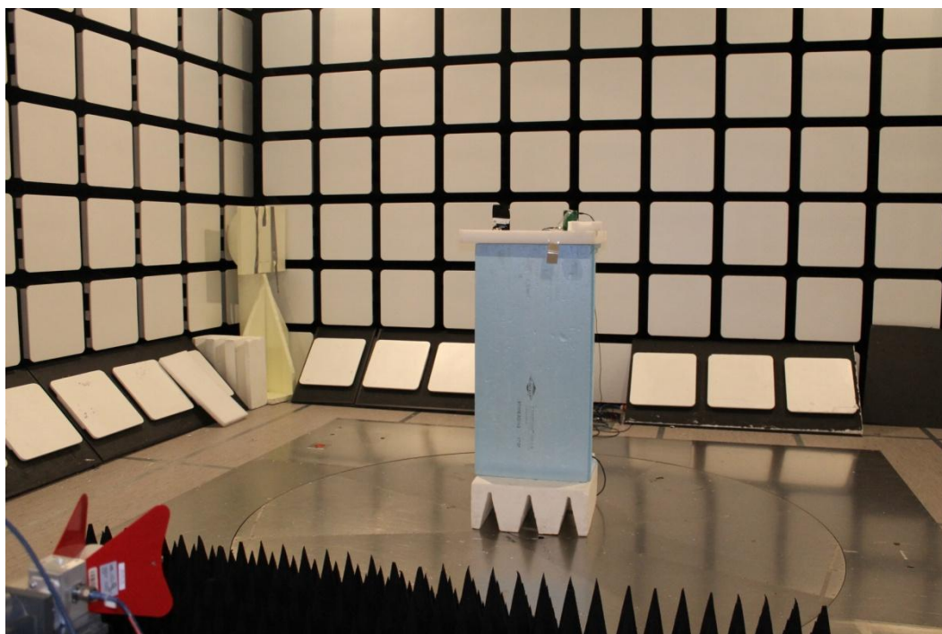
Photograph 1. Radiated emissions 1000 - 10000 MHz ant1.
