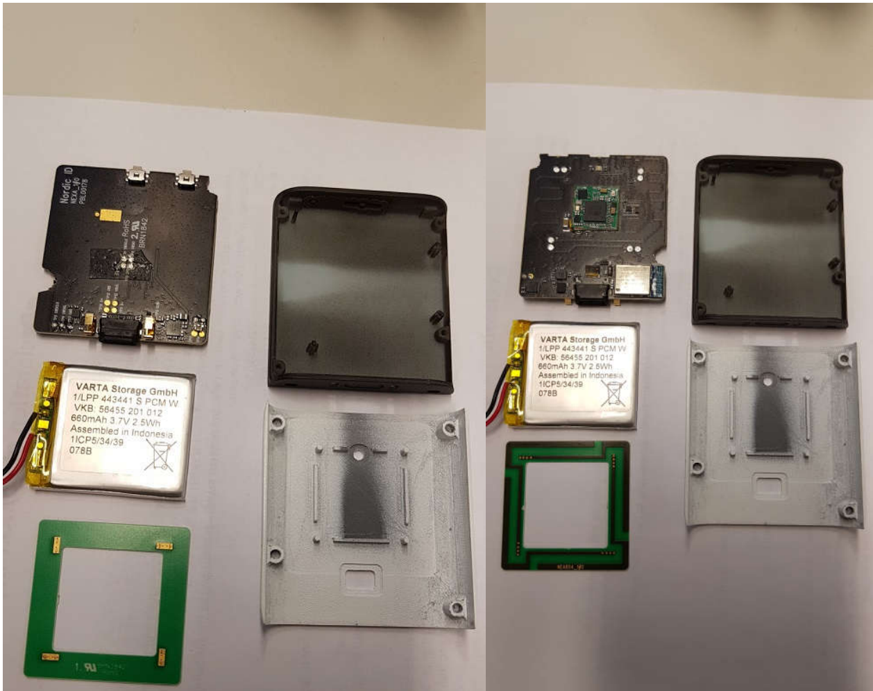
Pic. 3 and 4: Overview of EXA21 parts. A & B covers, antenna, battery and CPU board.
