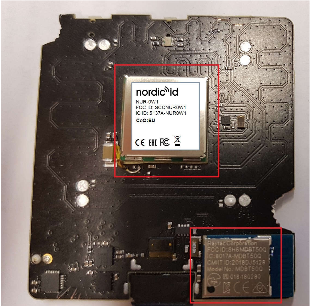
Pic.1: EXA21 CPU board bottom view. NUR-0W1 and MDBT50Q modules marked with red rectangle.
