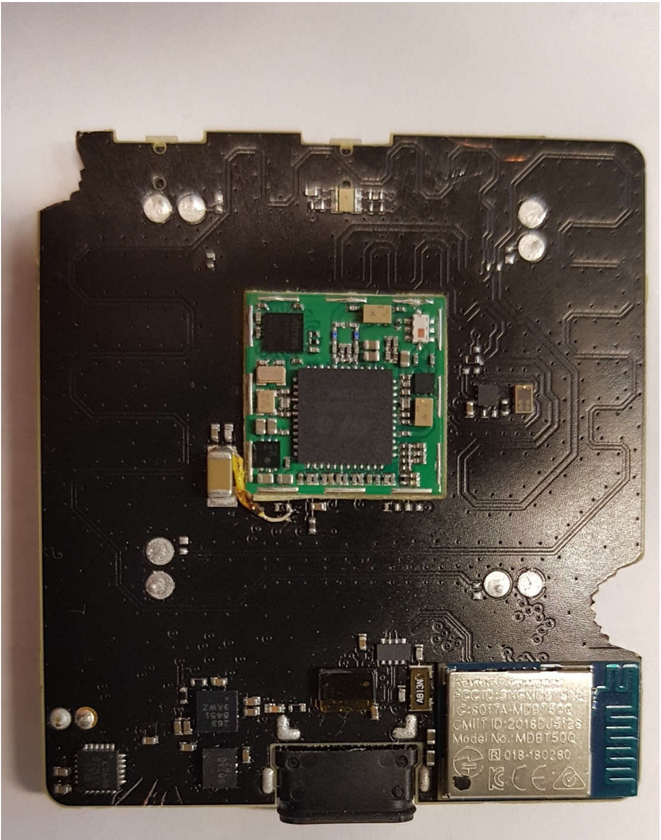
Pic.2: EXA21 CPU board bottom view. NUR-0W1 module without shield.
