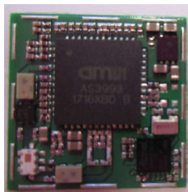
Picture 2. NUR-0W1 without shield
