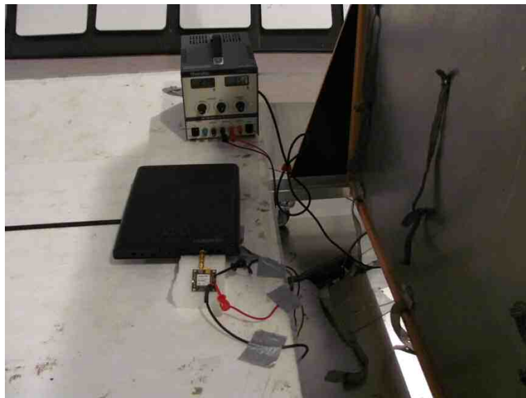
Photograph 4. Conducted Emissions
