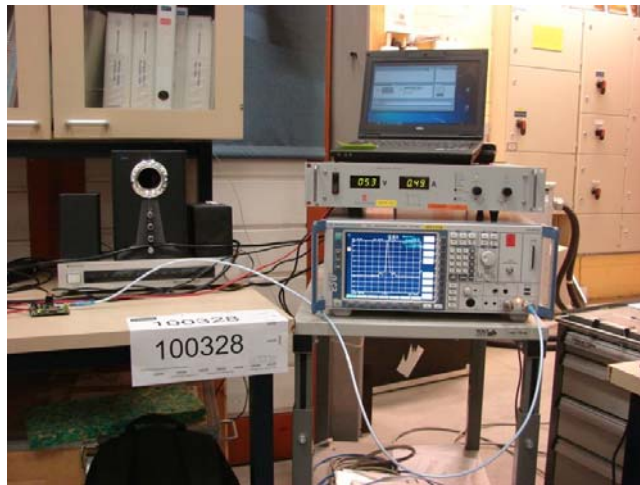
Picture 1: Conducted RF measurement test setup
