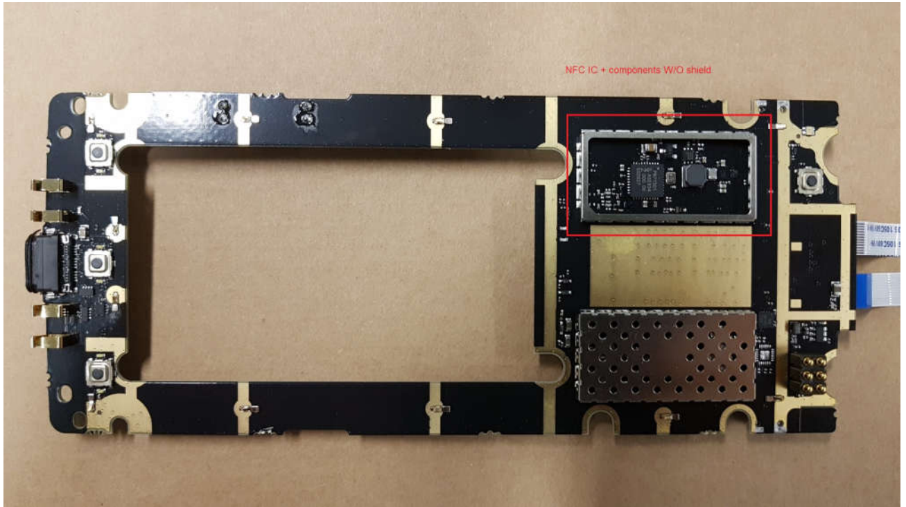
Picture 7. NFC radio without shield.
