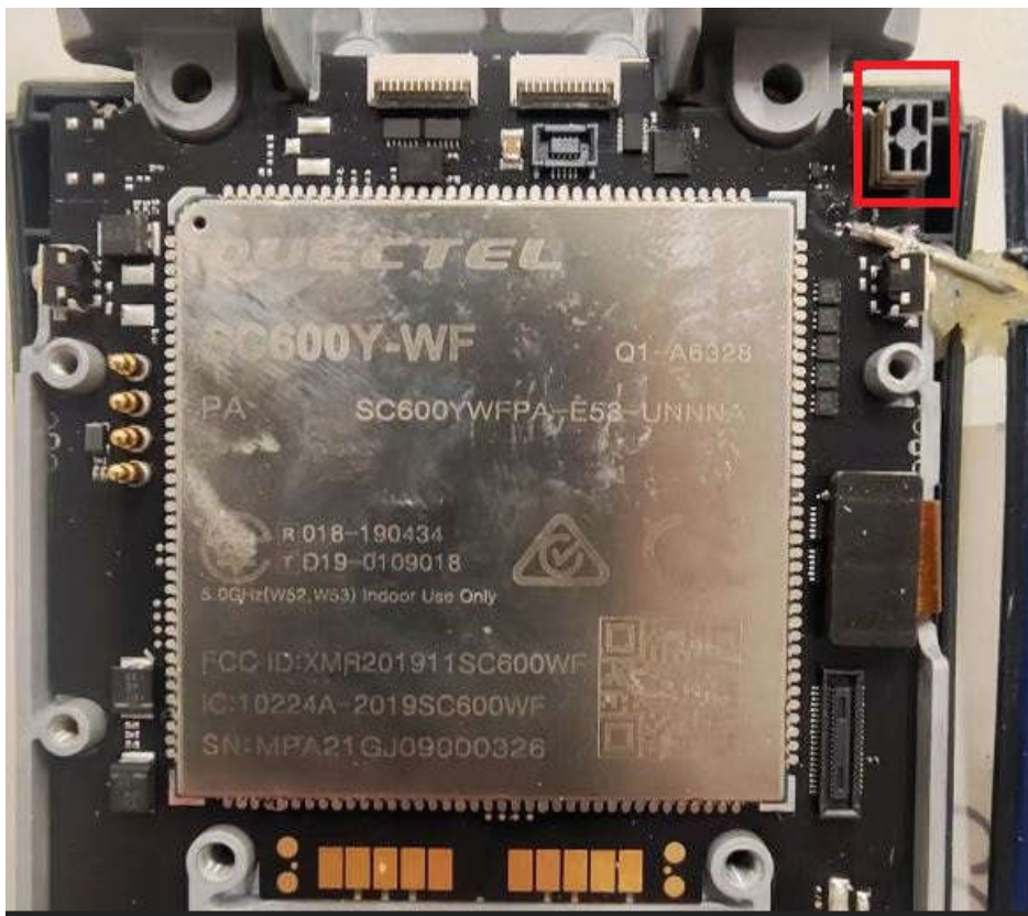
Picture 4. SC600Y-WF module information and WLAN/BT antenna location marked with red rectangular.
