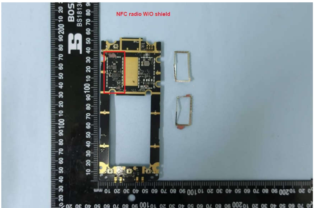
Picture 8. NFC radio without shield.
