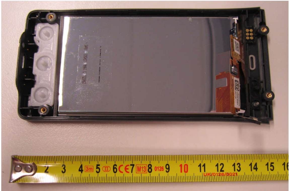
Picture 5. HH83 BARCODE main unit internal.
