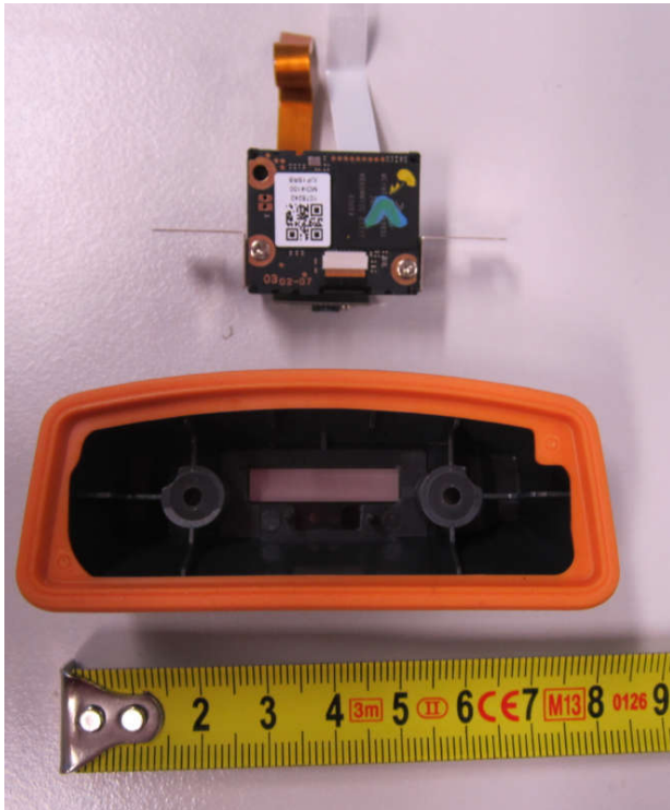
Picture 13. HH83 BARCODE 837-1A imager.
