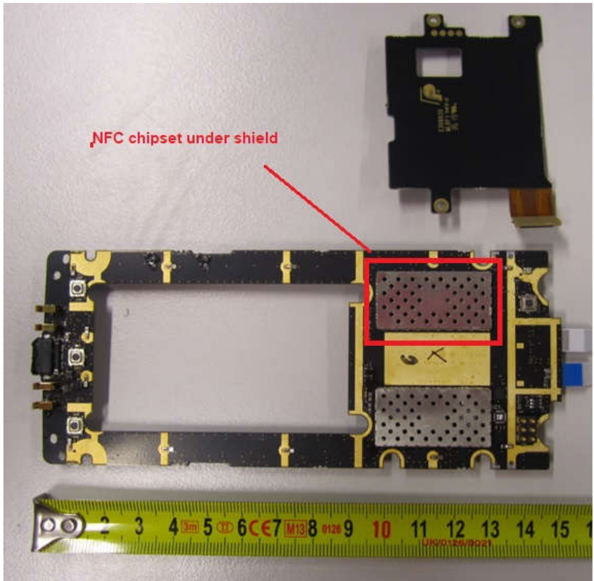
Picture 6. HH83 BARCODE main unit PCB side 2.
