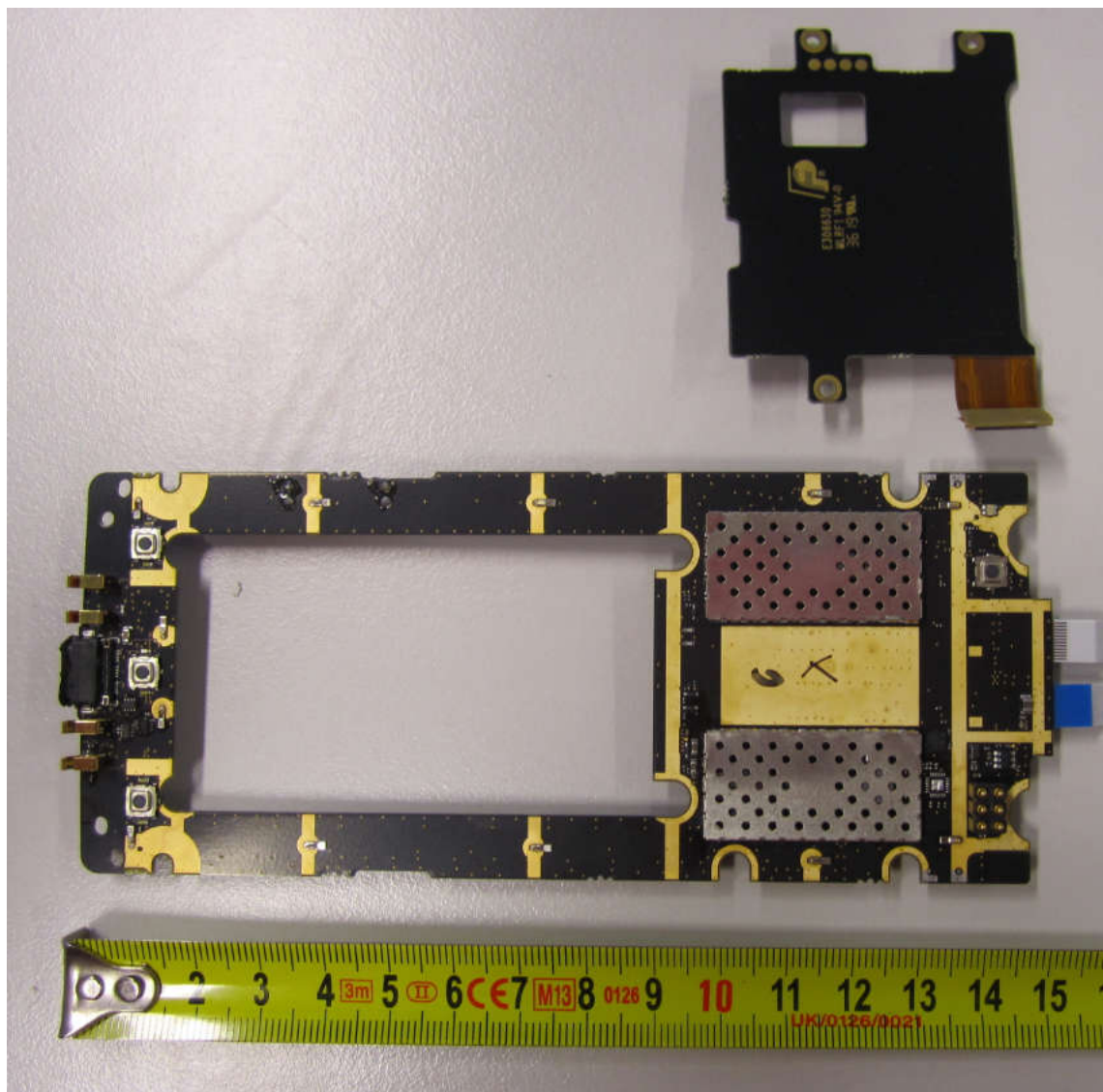
Picture 23. HH83 main unit PCBs 2.
