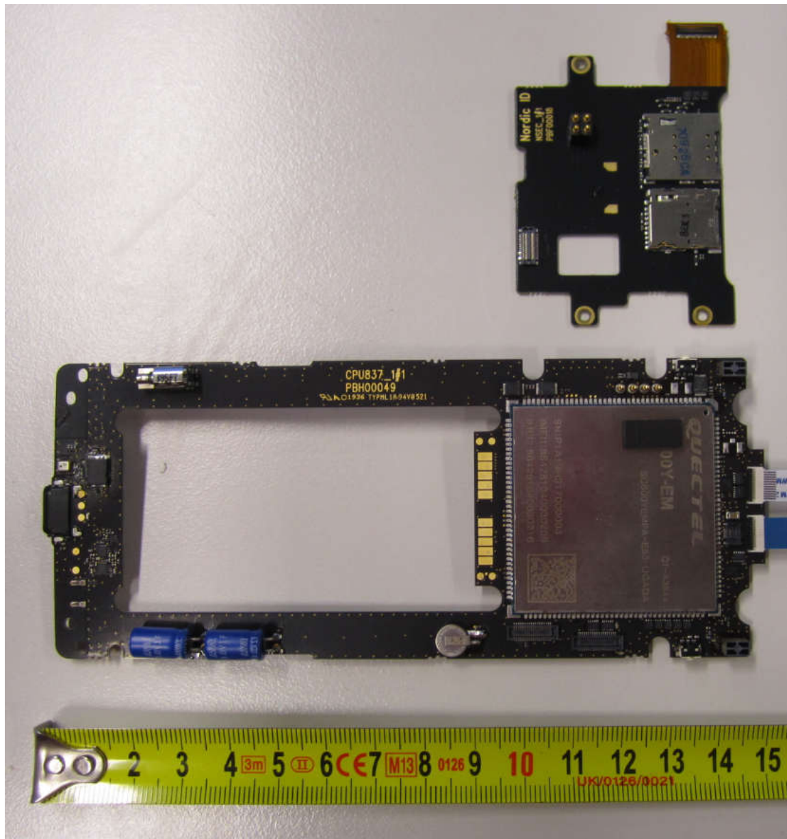
Picture 22. HH83 main unit PCBs 1.
