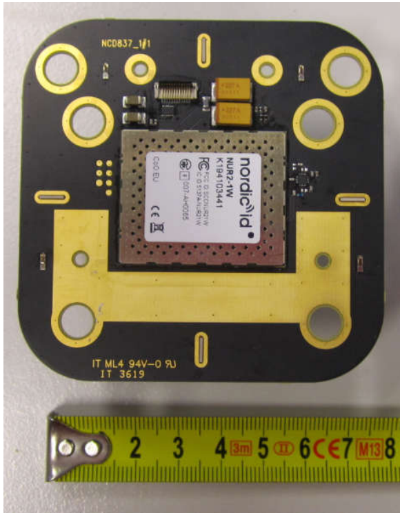
Picture 26. HH83 837-2A front end internal 3.
