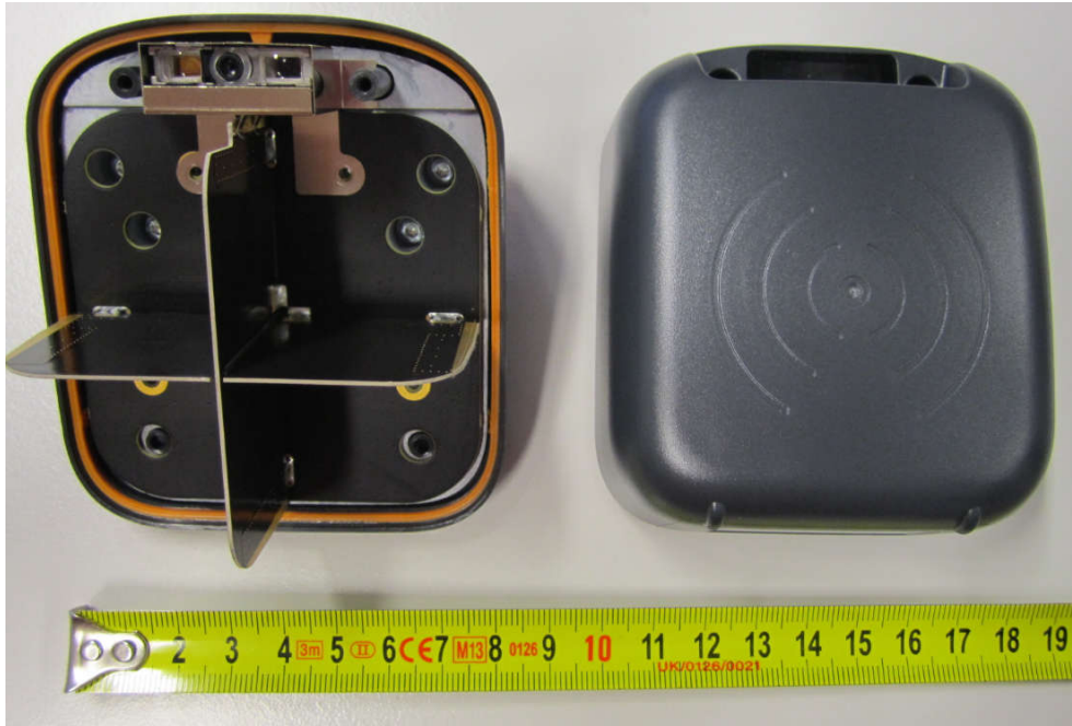
Picture 24. HH83 837-2A front end internal 1.
