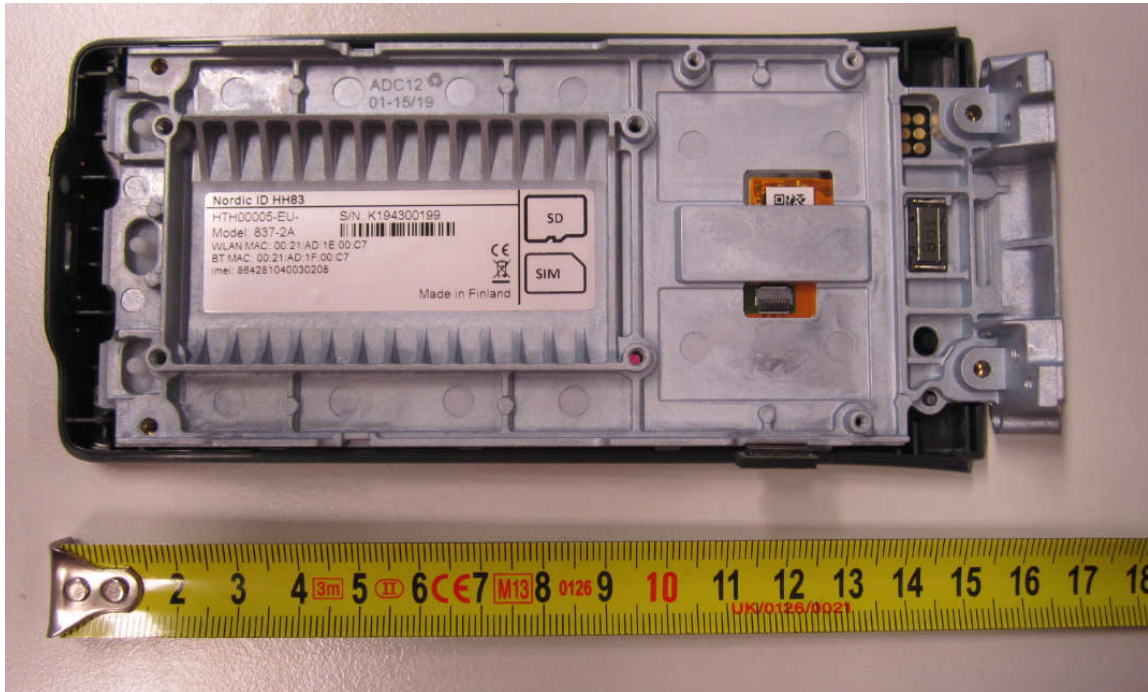
Picture 20. HH83 main unit internal 2.
