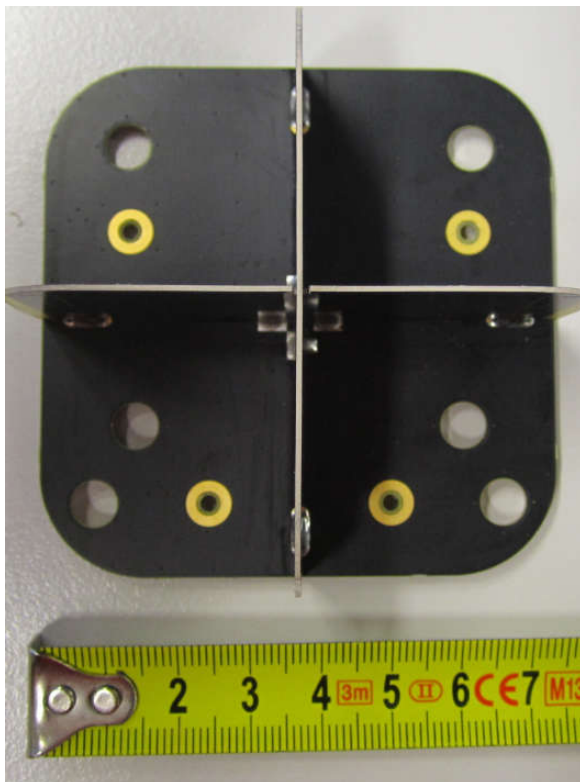
Picture 27. HH83 837-2A front end internal 4.
