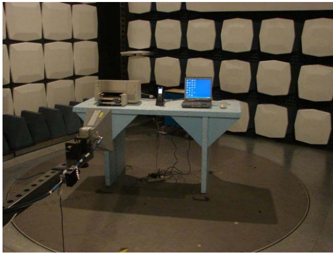
Picture 4: Receiver Radiated emission test setup 1 GHz – 12,5 GHz
