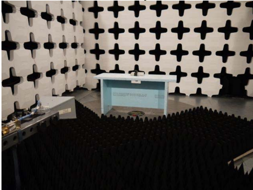
Picture 2: Radiated emission test setup above GHz
