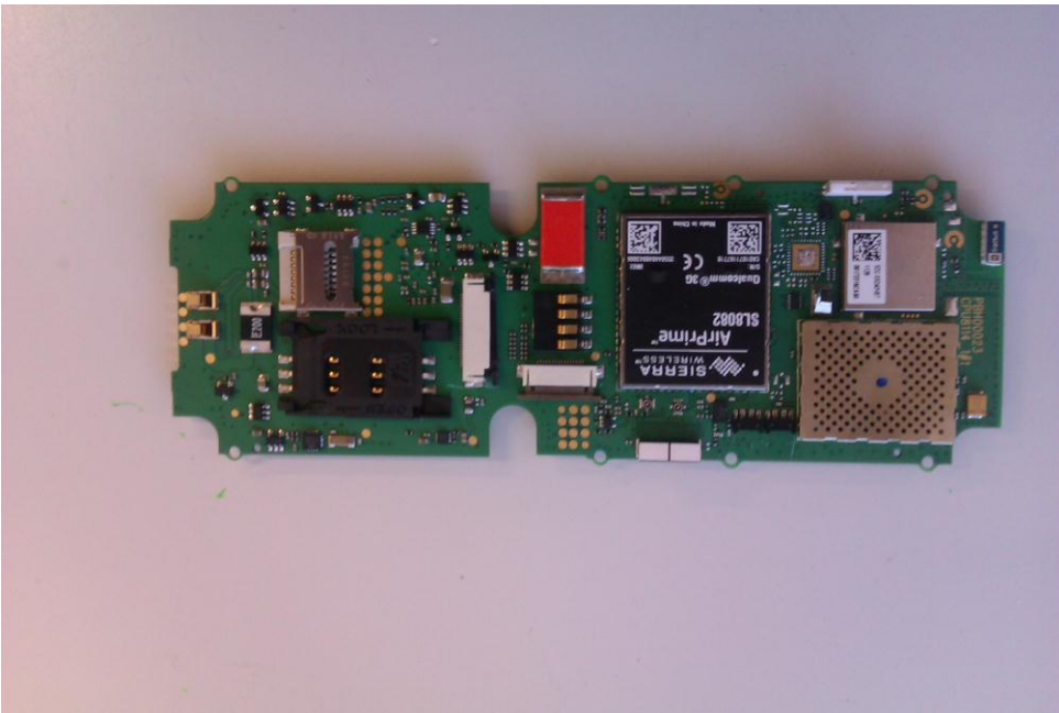
Picture 13: CPU811 board top side
