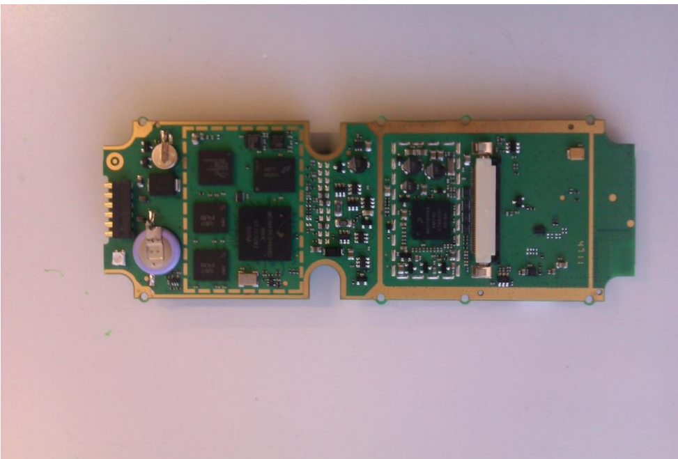
Picture 14: CPU811 board bottom side
