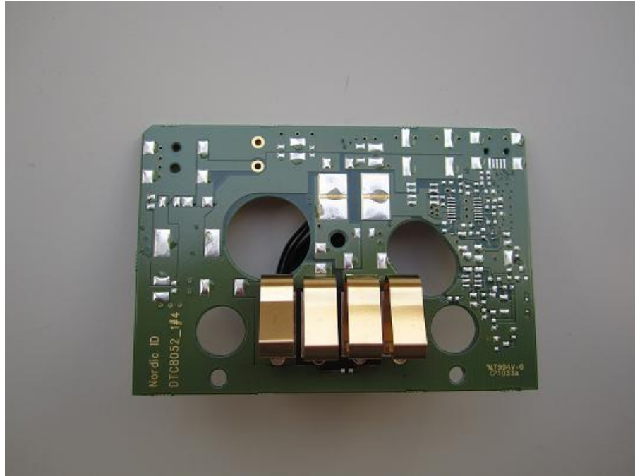
Picture 15: DTC8052 board top side
