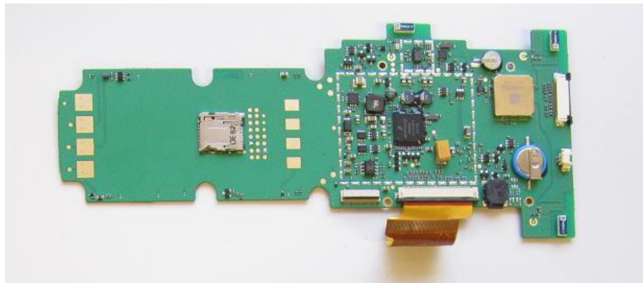
Picture 12: CPU805_2 board bottom side
