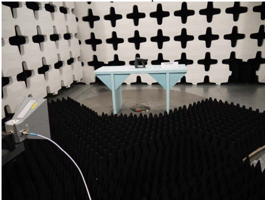
Picture 3: Radiated emission test setup 16 GHz – 26 GHz.
